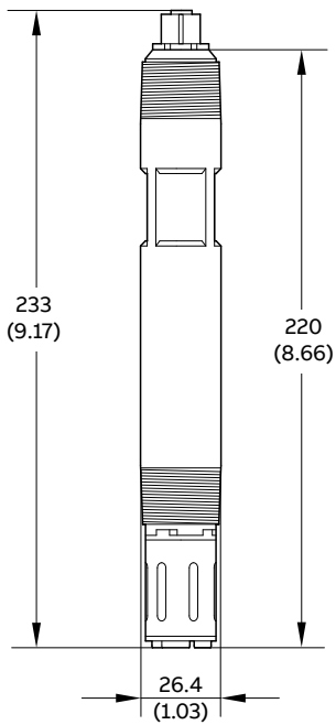
Figure 6 ADS420 cable detached
