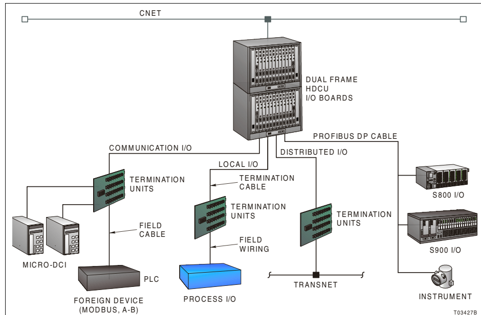
Figure 4. Harmony DCU I/O
