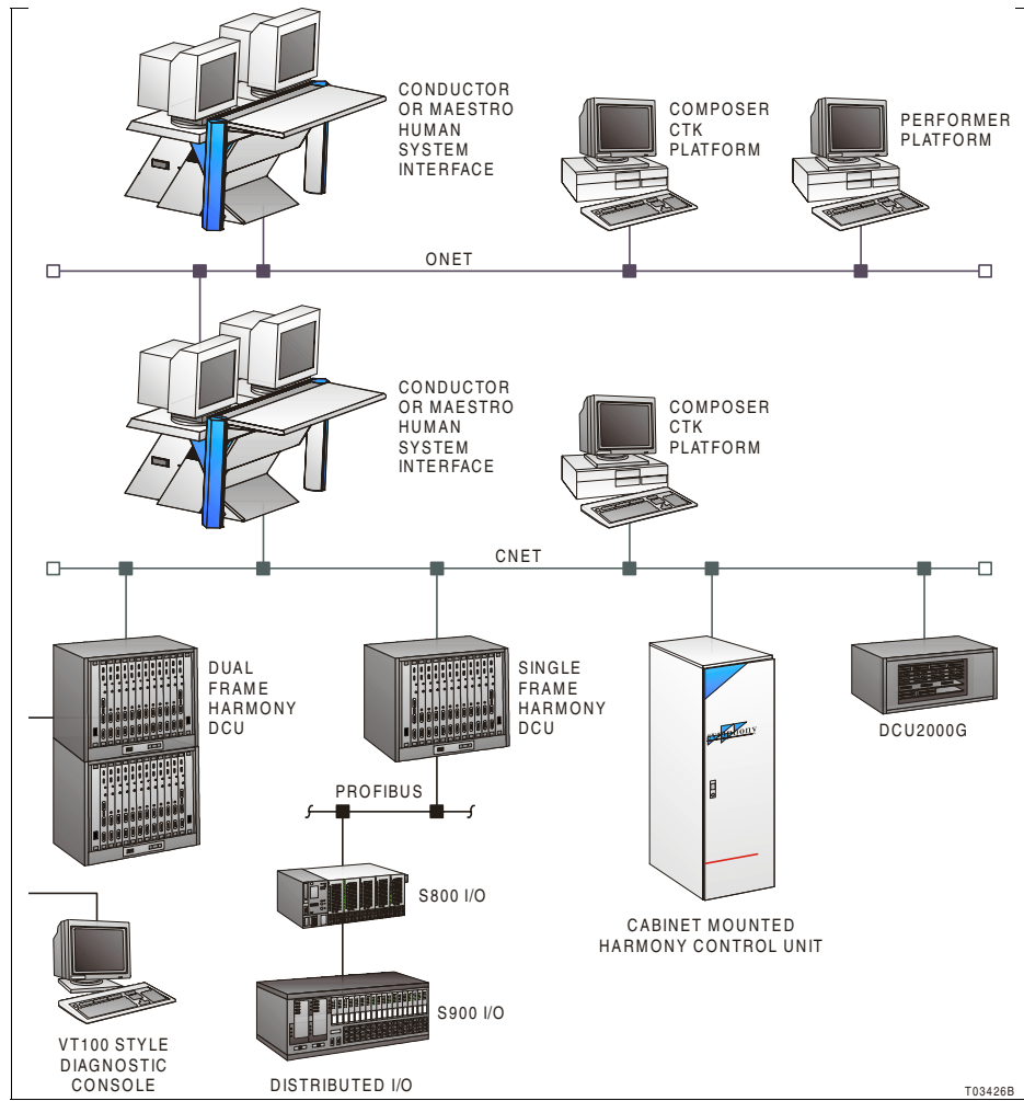
Figure 3. Harmony Communications Architecture
