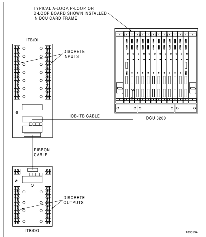
Figure 2. Typical IOB Connection to ITB
