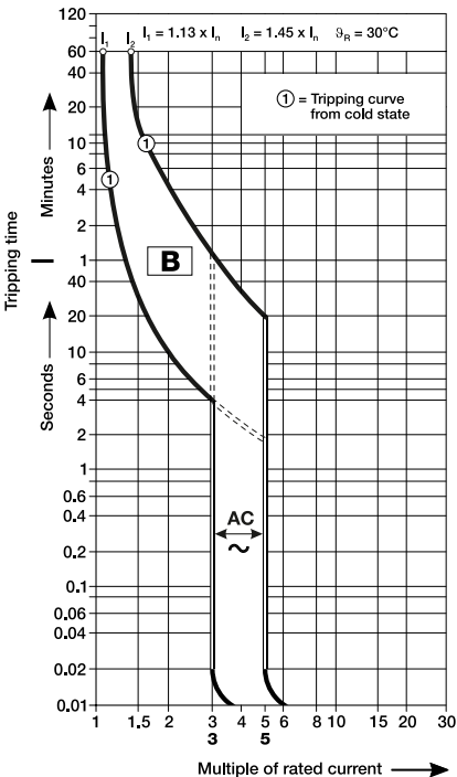
Characteristic B IEC-EN60898-1
