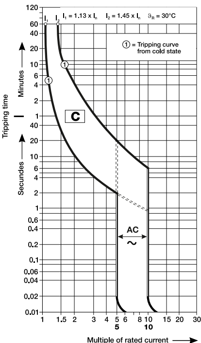
Characteristic C IEC-EN60898-1
