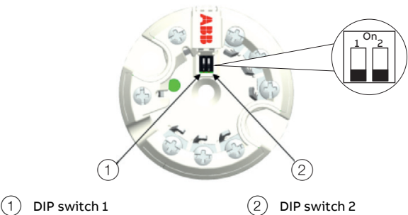
Figure 23: DIP switch on the transmitter
