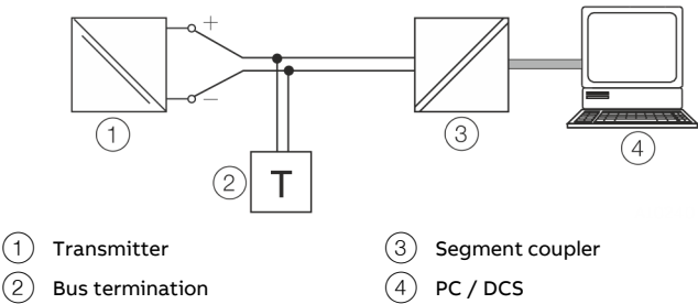
Figure 21: Example for PROFIBUS PA® connection
