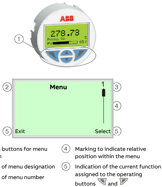
Figure 24: LCD indicator (example)
