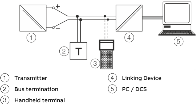
Figure 22: Example for FOUNDATION Fieldbus® connection
