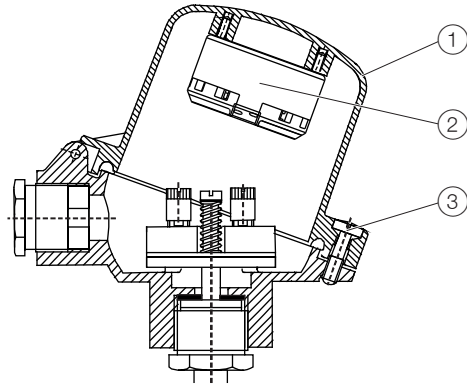
Figure 12: Installation example
