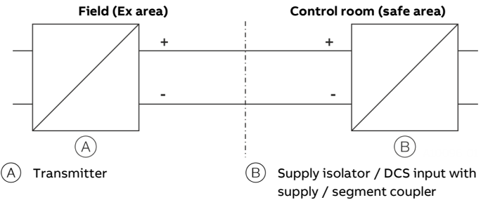
Figure 1: Intrinsic safety installation check
