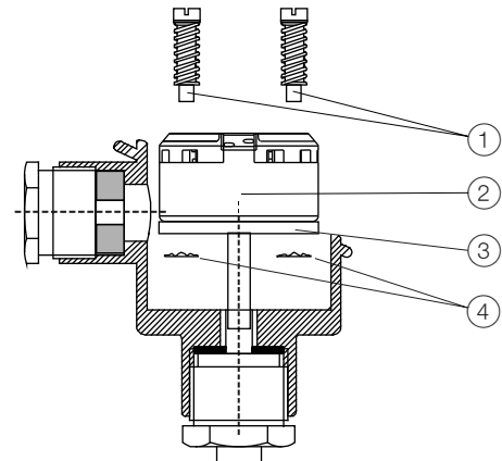
Figure 11: Installation example
