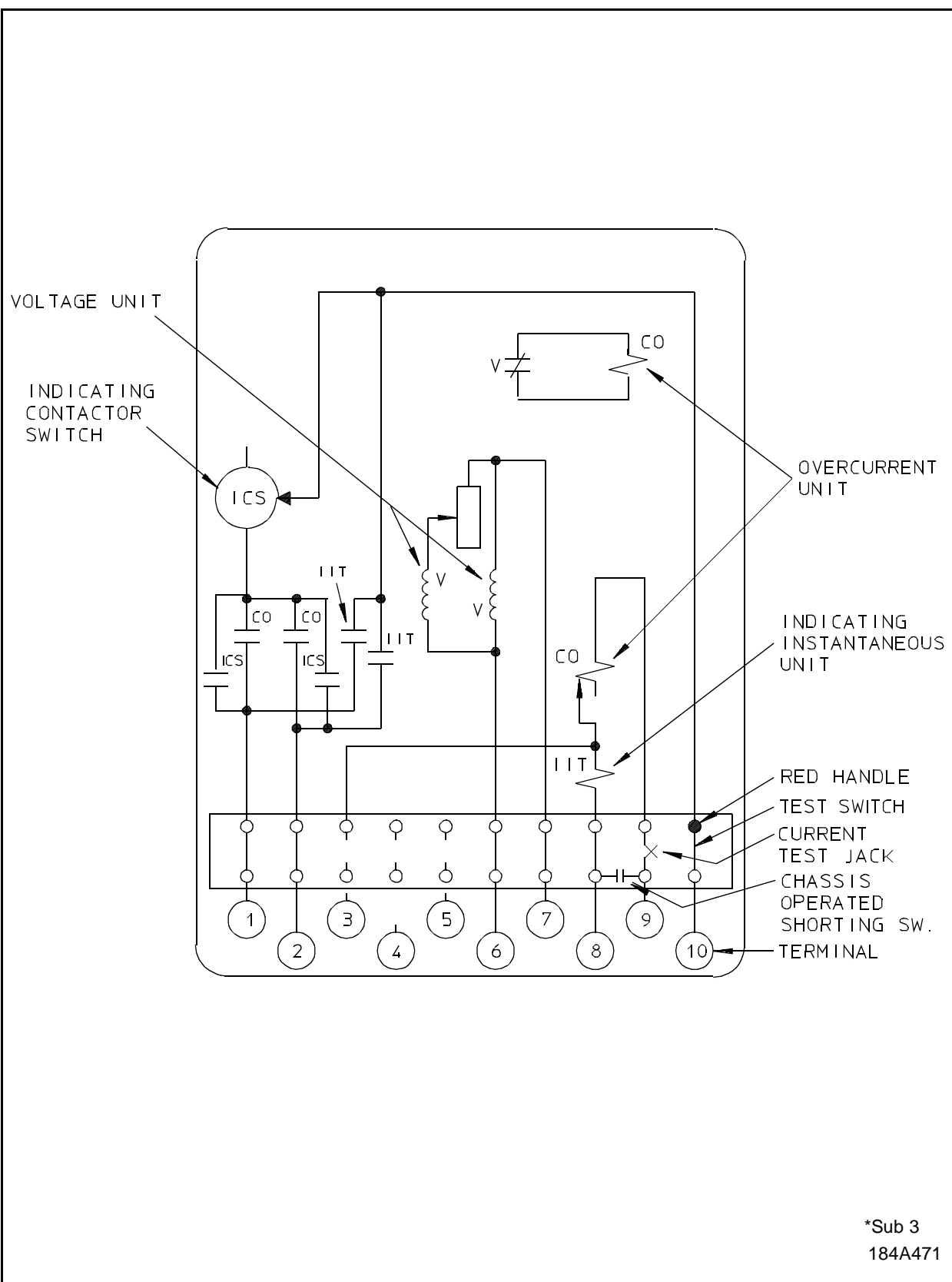
Figure 1 1 Relay Types COV-6, COV-7, COV-8, COV-9 & COV-11 Voltage Controlled Overcurrent Relay, Double Trip with Indicating Instantaneous Trip, in Type FT21 Case
