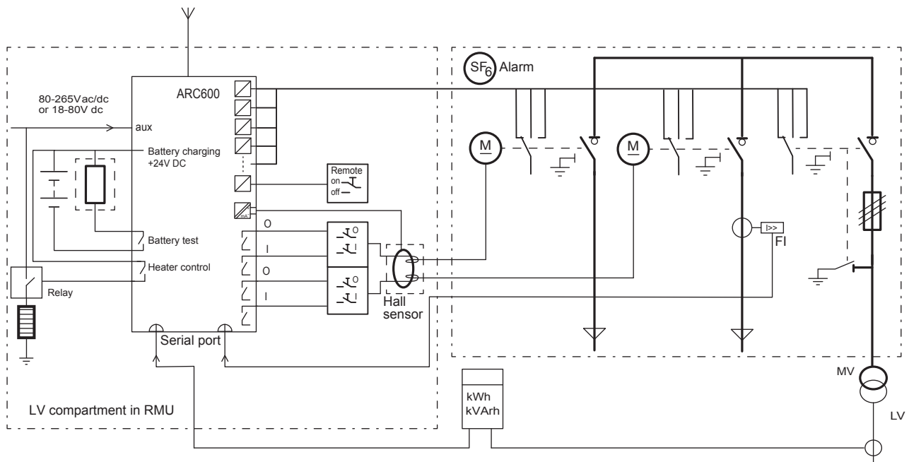
Figure 5. An ARC600 unit used for the remote control of a Ring Main Unit and fault indication
