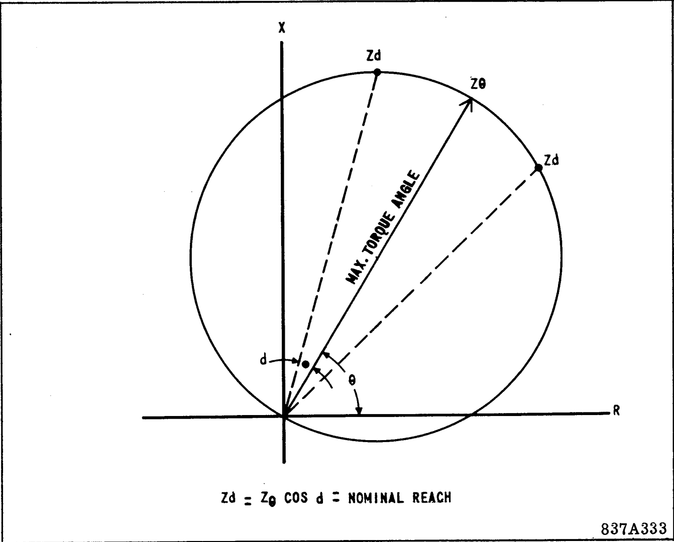
Fig. 4 Test Unit Check Points
