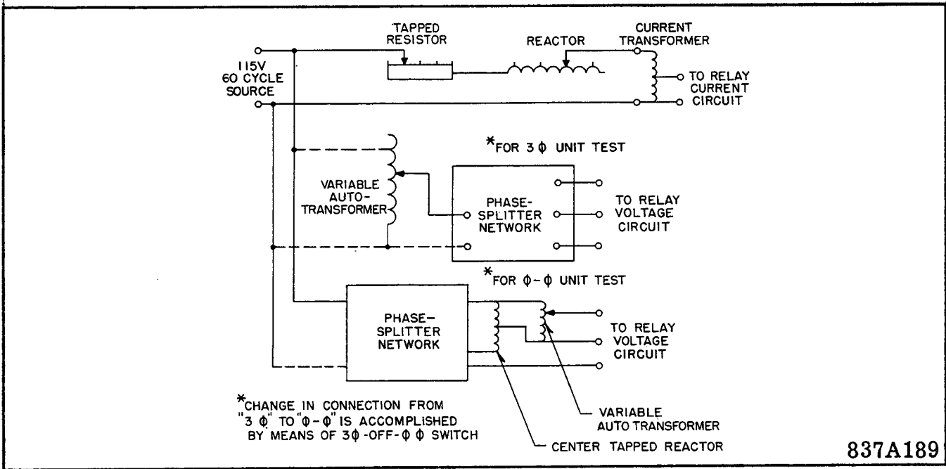
Fig. 2 Basic Schematic Diagram
