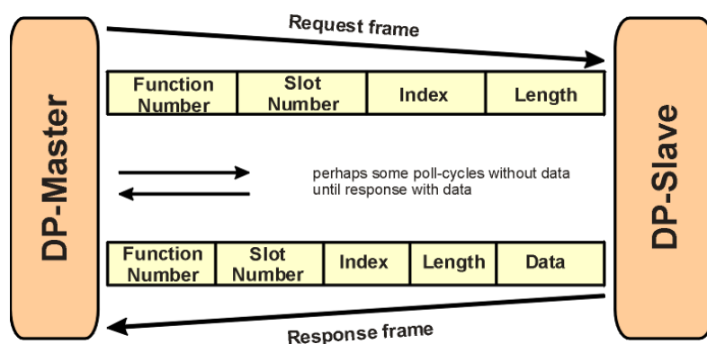
Fig. 2 Acyclic Communication in DP-V1: Read Service
