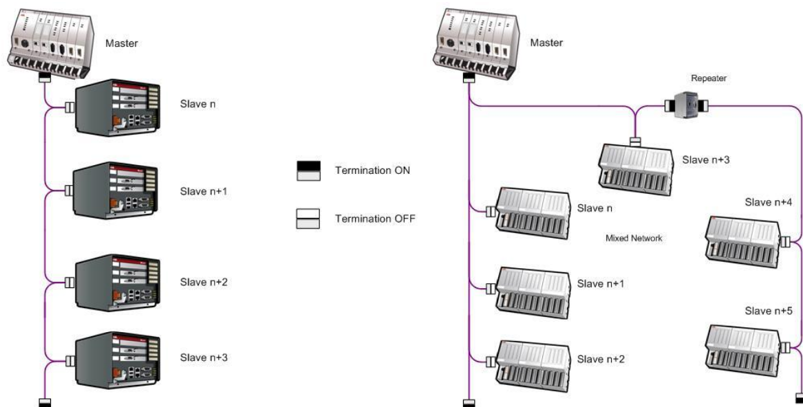
Fig. 4 MLink PROFIBUS connection and termination examples
