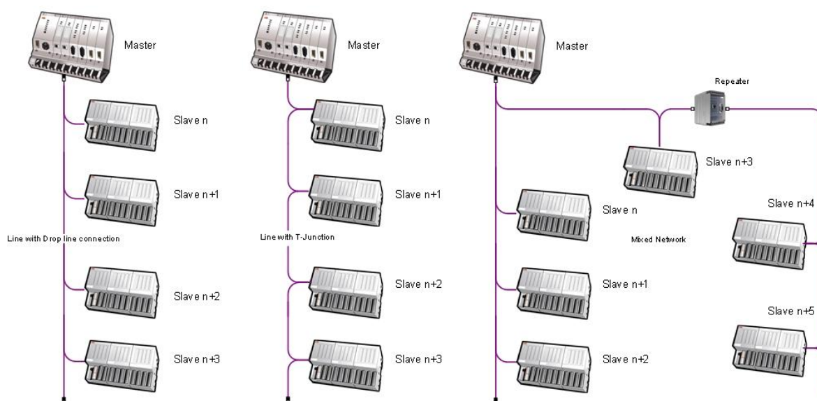
Fig. 3 PROFIBUS network principles
