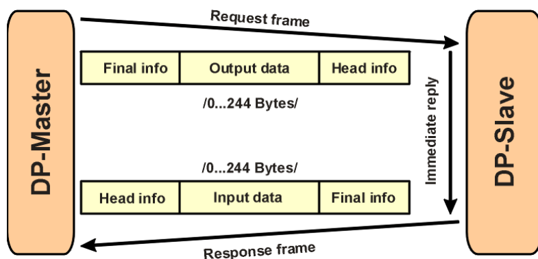
Fig. 1 Cyclic User Data Transmission in DP
