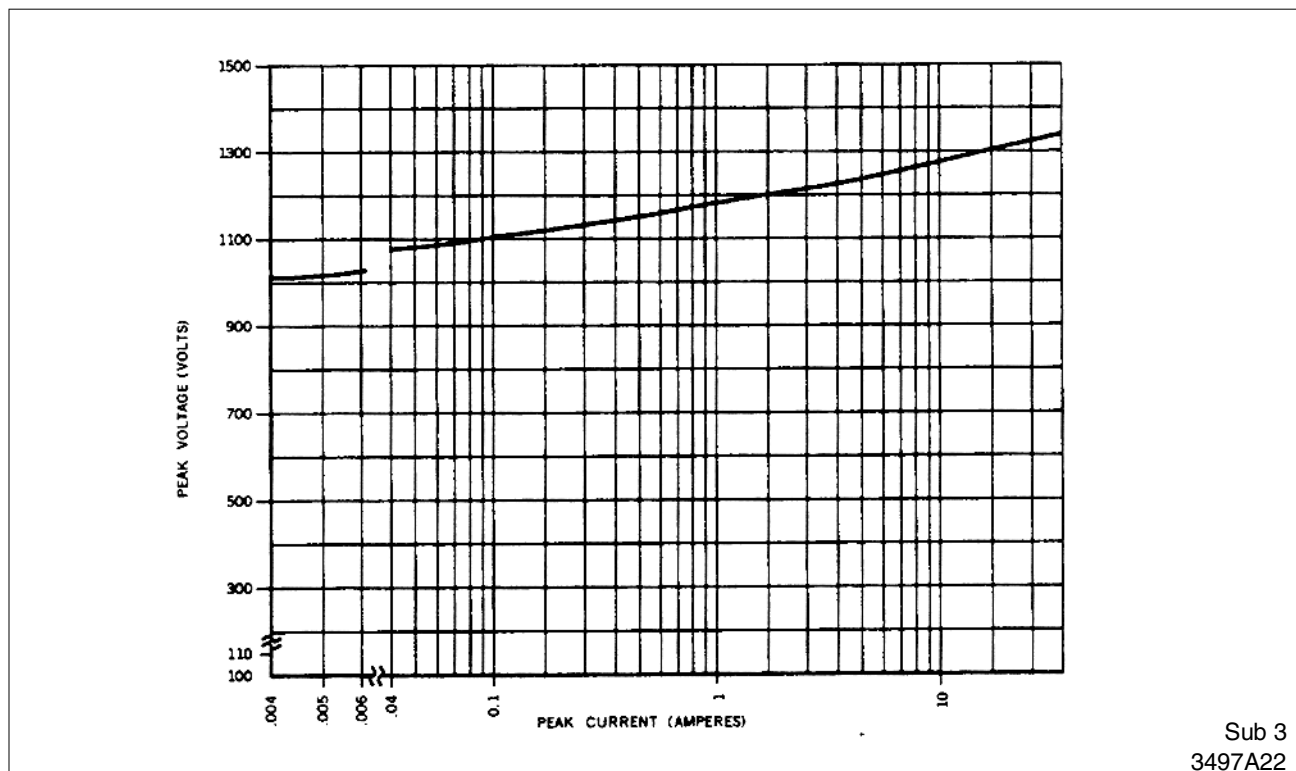
Figure 3: Typical Volt-Ampere Characteristic of Varistor in Type KAB Relay (Peak Value).
