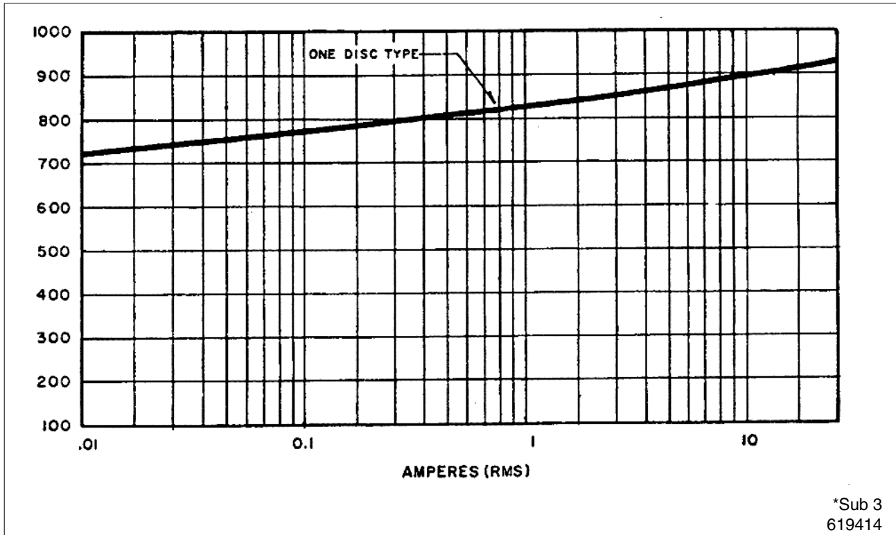
Figure 4: Typical Volt-ampere characteristic of Varistor in Type KAB Relay (RMS).
