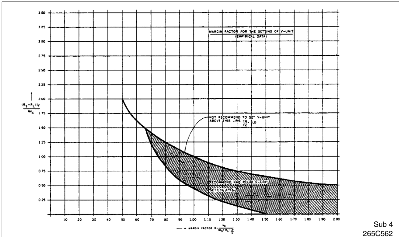
Figure 5: Margin Factor for V-Unit Setting
