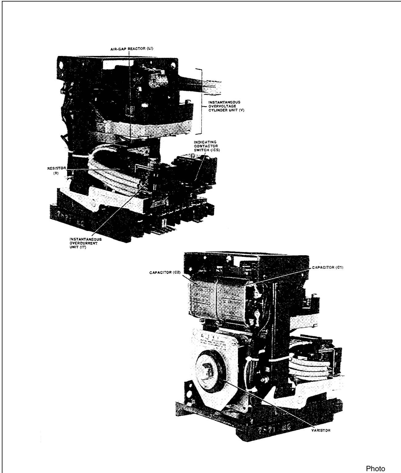
Figure 1: Type KAB Relay without case
