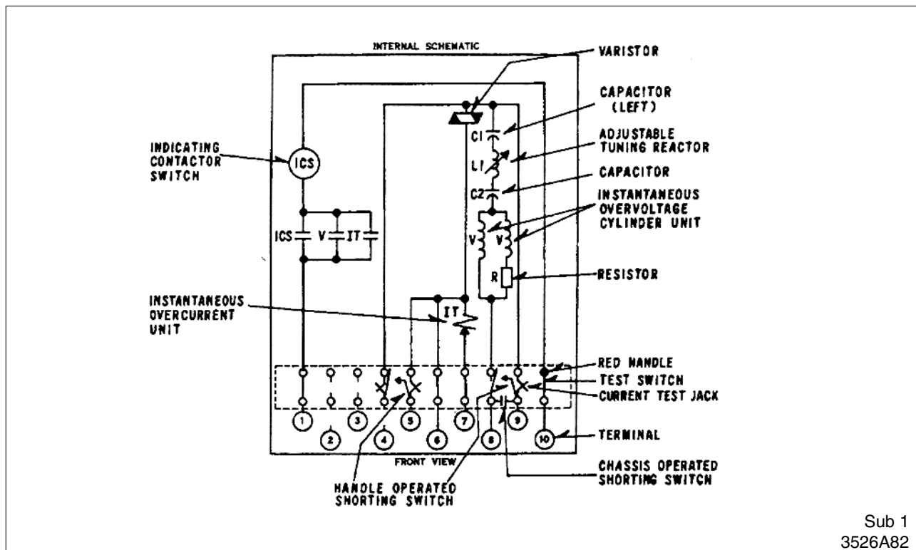
Figure 2: Internal Schematic of KAB Relay with in Service CT Check Feature.
