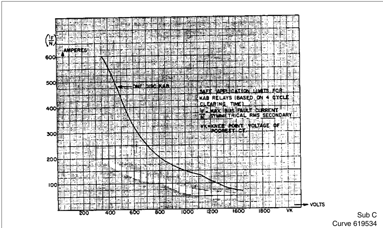
Figure 8: Safe Application Limits for KAB Relays
