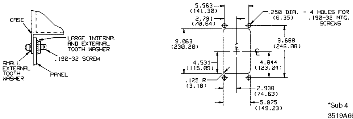
Figure 9: Outline and Drilling Plan for TYPE KAB Relay in Type FT-21 Case
