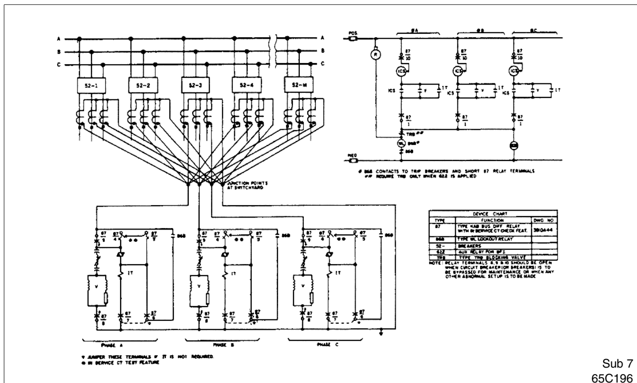
Figure 7: External Connections
