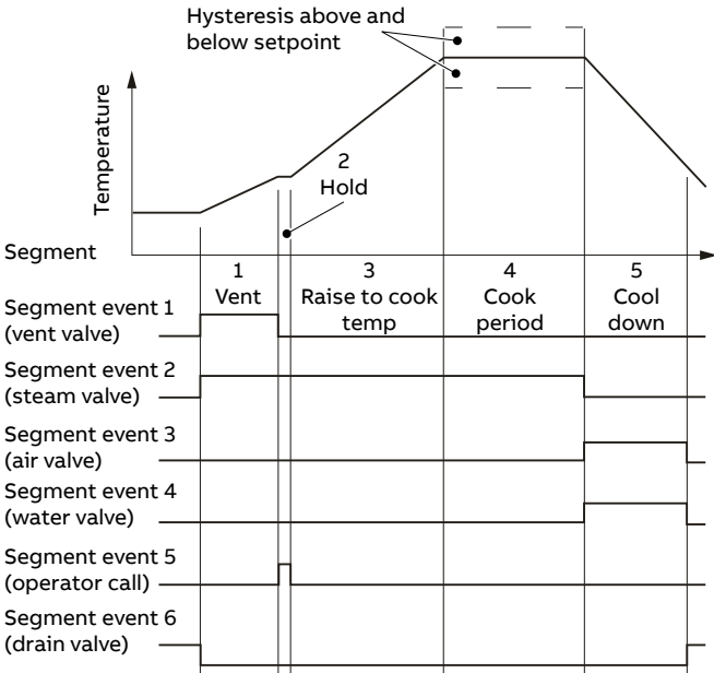
Figure 18 Profile control
