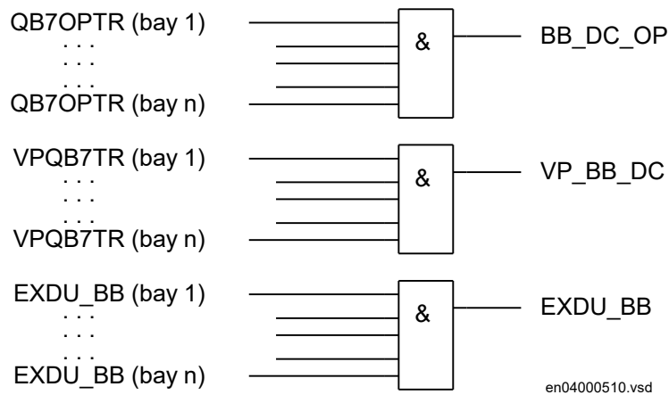
Figure 359: Signals from bypass busbar to busbar earthing switch
