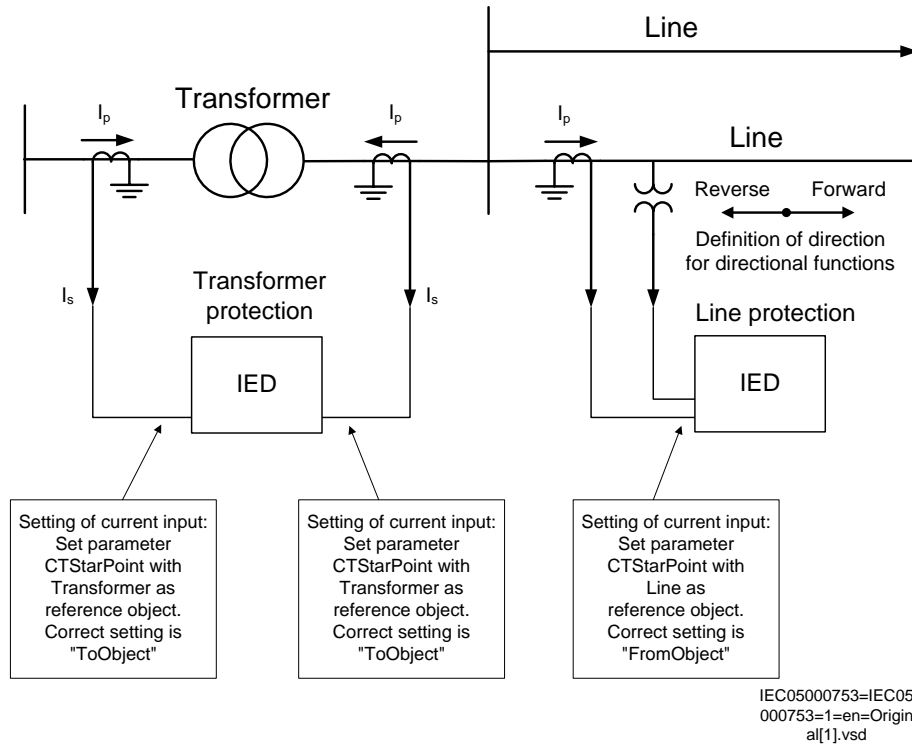
Figure 8: Example how to set CTStarPoint parameters in the IED
