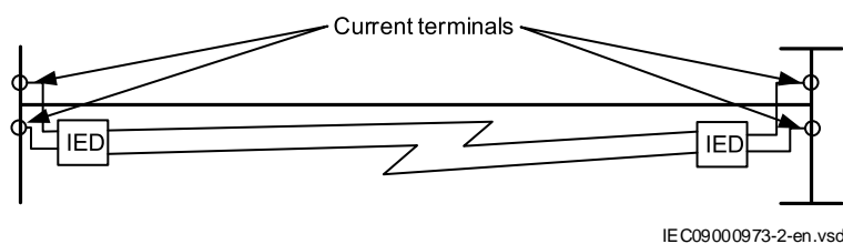
Figure 49: Example when setting NoOfUsedCTs = 4 in 1½ breaker configurations
