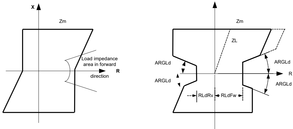
Figure 146: Load encroachment phenomena and shaped load encroachment characteristic
