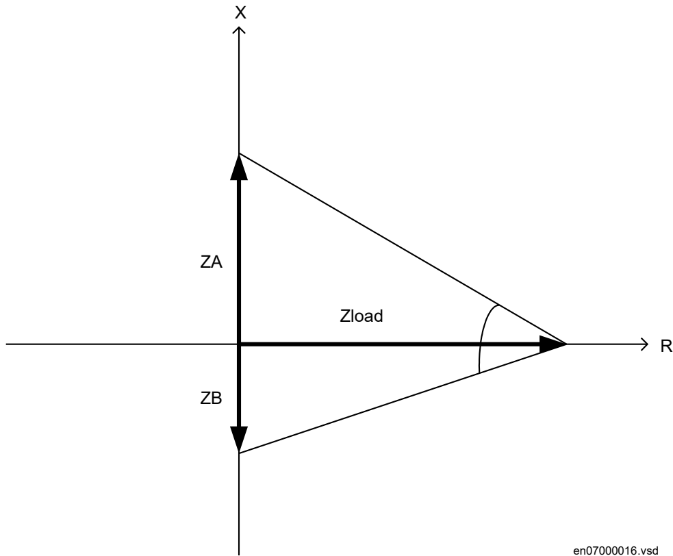
Figure 245: Simplified figure to derive StartAngle
