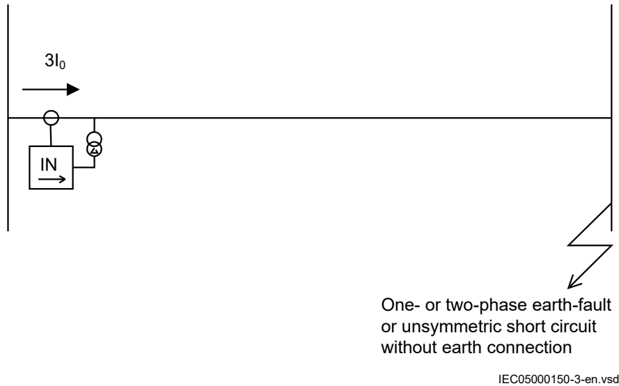
Figure 271: Step 1, first calculation
