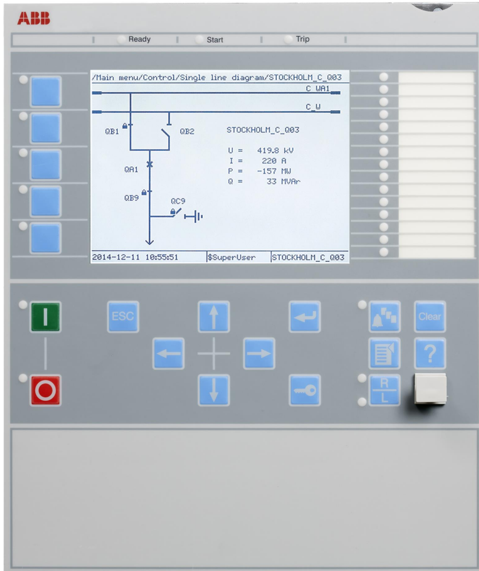
Figure 26: Local human-machine interface
