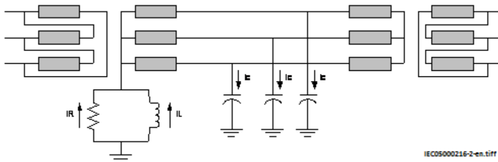
Figure 180: High impedance earthing network
