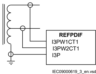
Figure 389: REFPDIF function inputs for autotransformer application
