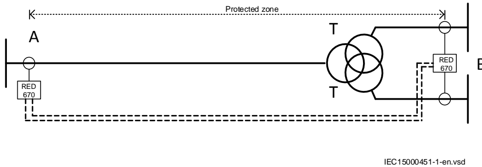
Figure 56: One three-winding transformer in the protected zone
