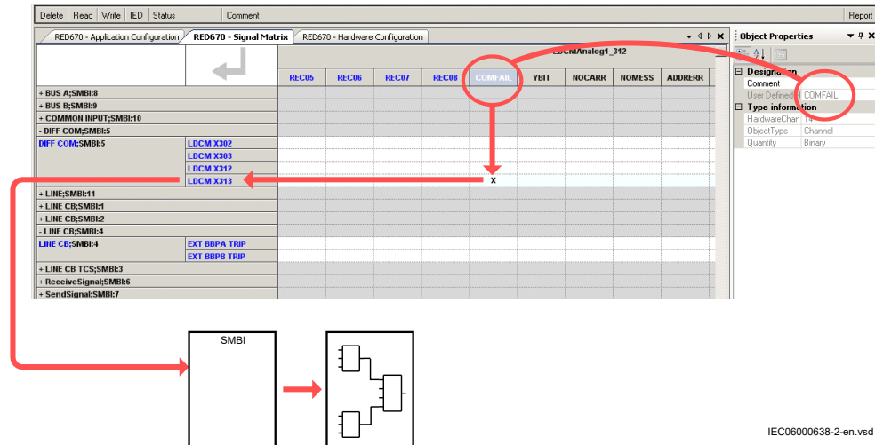
Figure 48: Example of LDCM signals as seen in the Signal matrix tool
