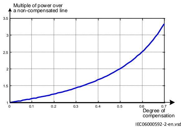
Figure 82: Increase in power transfer over a transmission line depending on degree of series compensation
