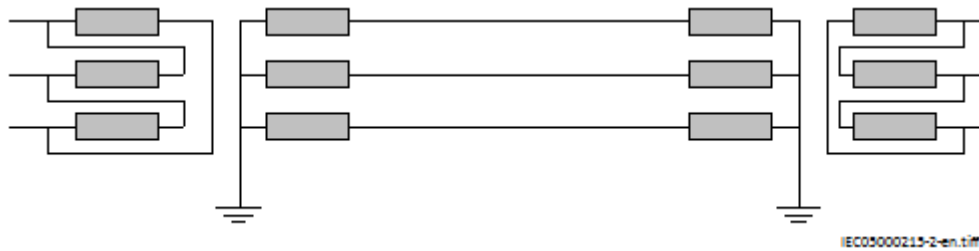
Figure 156: Solidly earthed network.
