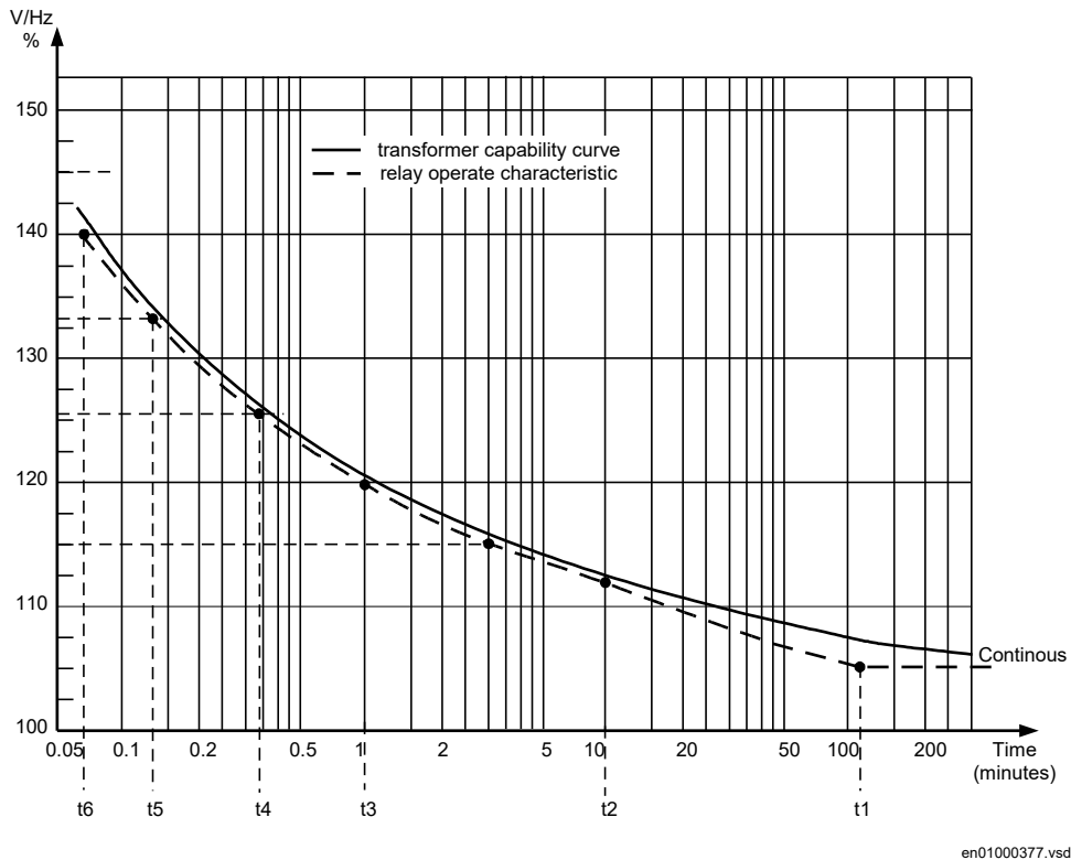
Figure 296: Example on overexcitation capability curve and V/Hz protection settings for power transformer
