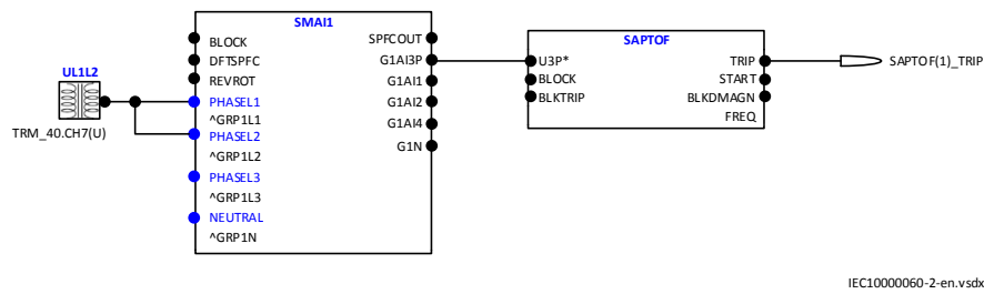
Figure 419: Connection example
