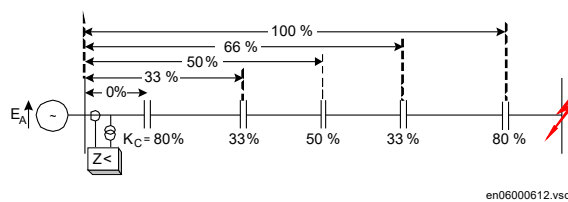
Figure 96: Typical locations of capacitor banks on series compensated line
