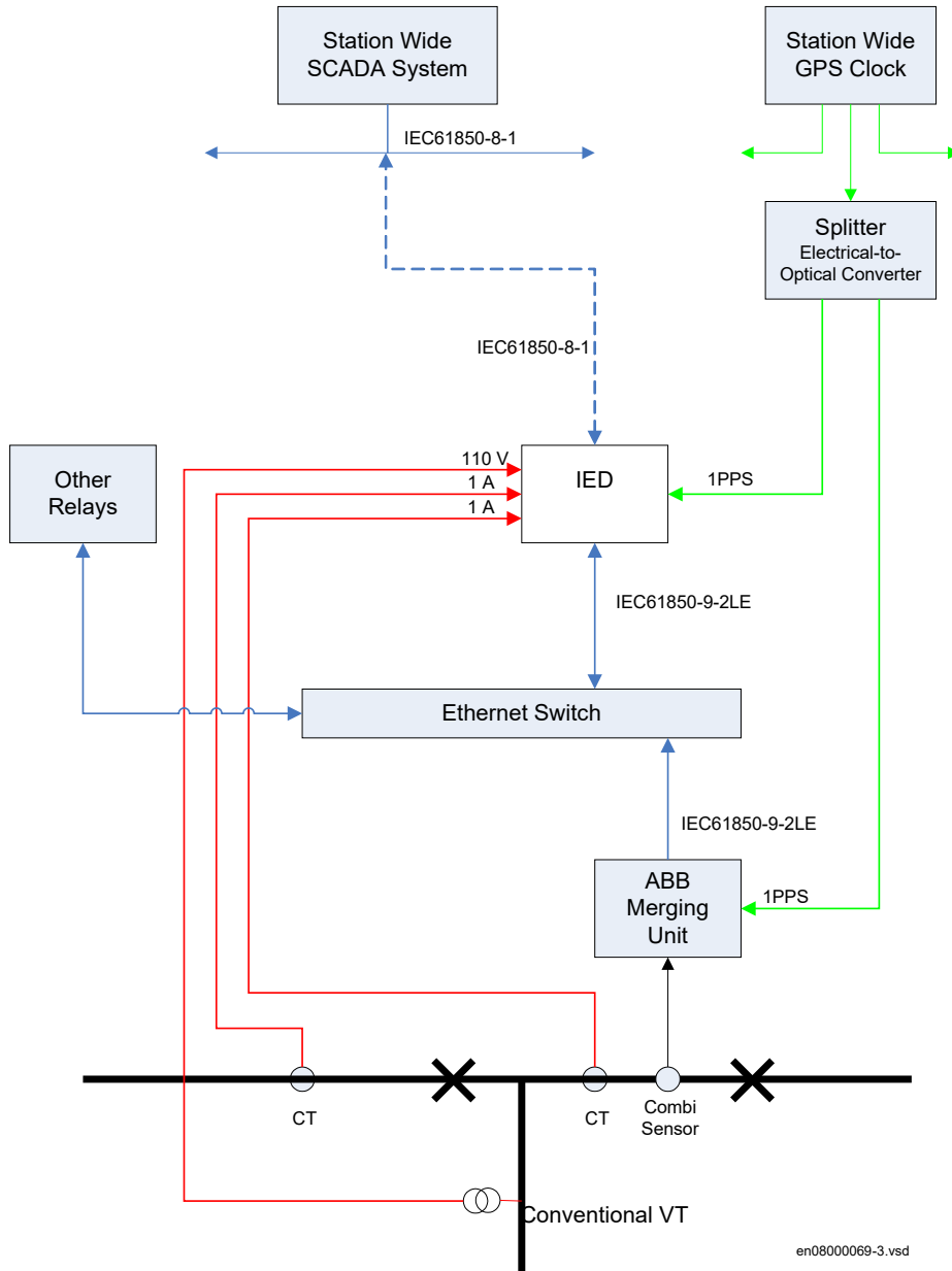
Figure 406: Example of a station configuration with the IED receiving analog values from both classical measuring transformers and merging units.
