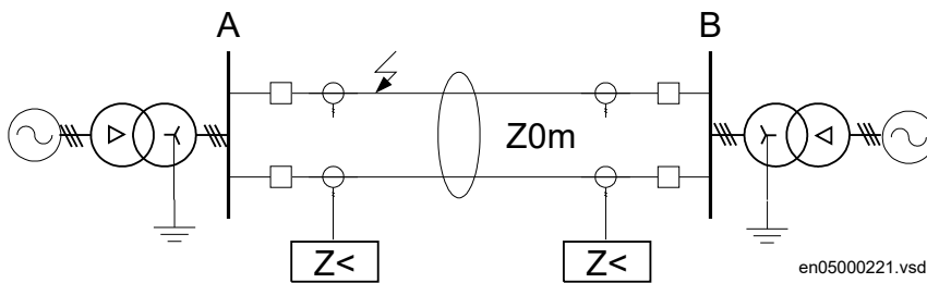
Figure 147: Class 1, parallel line in service.
