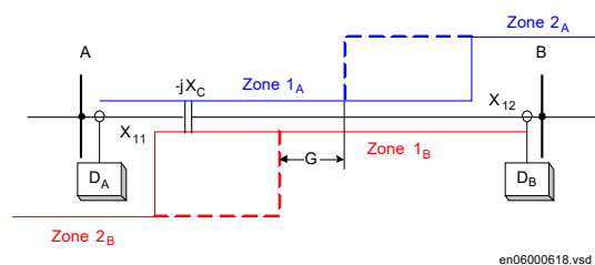
Figure 101: Underreaching (Zone 1) and overreaching (Zone 2) on series compensated line
