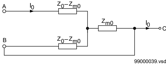
Figure 150: Equivalent zero-sequence impedance circuit for the double-circuit line that operates with one circuit disconnected and earthed at both ends.
