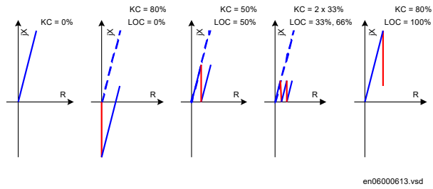
Figure 215: Apparent impedances seen by distance IED for different SC locations and spark gaps used for overvoltage protection
