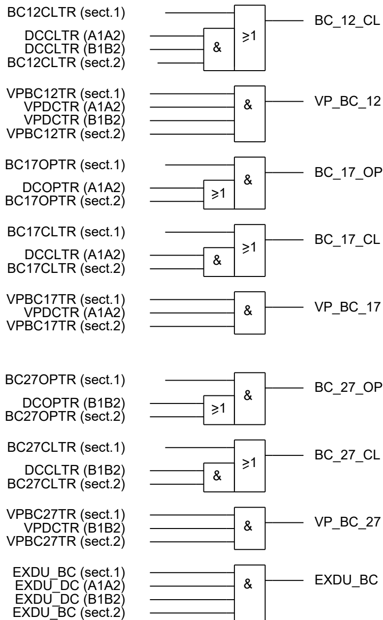
Figure 328: Signals to a line bay in section 1 from the bus-coupler bays in each section
