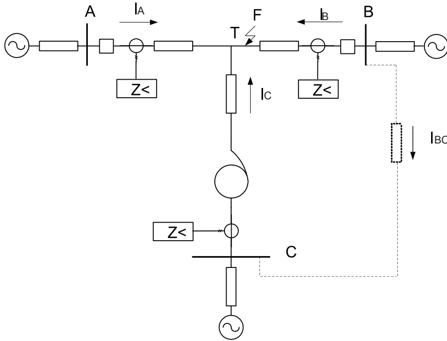
Figure 138: Example of tapped line with Auto transformer
