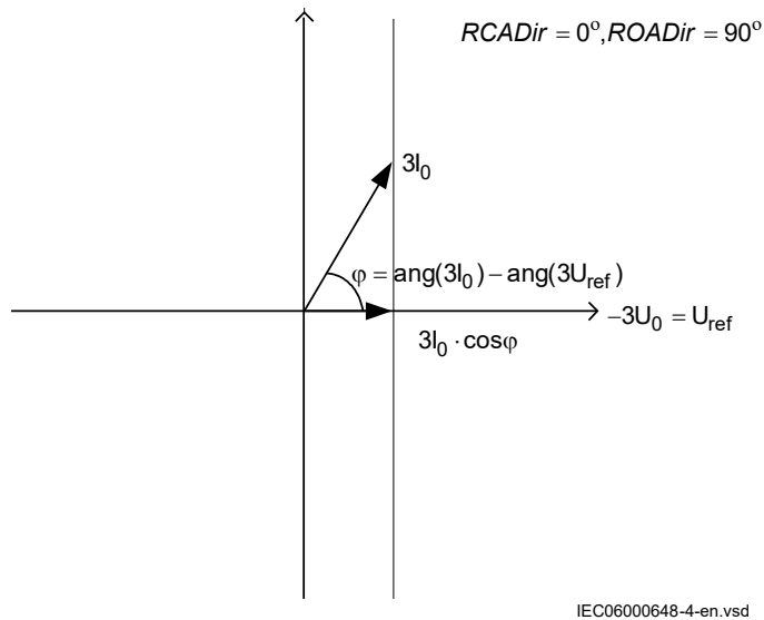
Figure 281: Characteristic for RCADir equal to 0^\circ
