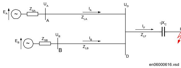
Figure 100: Voltage inversion in series compensated network due to fault current infeed
