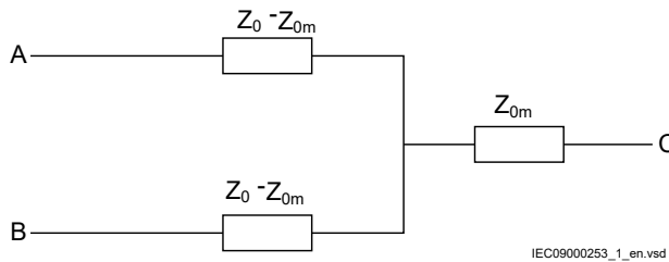
Figure 123: Equivalent zero sequence impedance circuit of the double-circuit, parallel, operating line with a single phase-to-earth fault at the remote busbar
