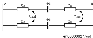
Figure 225: Double circuit, parallel operating line
