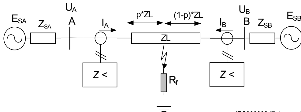
Figure 181: Influence of fault current infeed from remote line end
