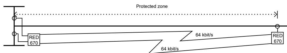
Figure 46: Two-terminal line with 1½ breaker
