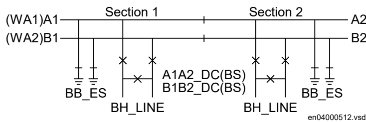
Figure 361: Busbars divided by bus-section disconnectors (circuit breakers)
