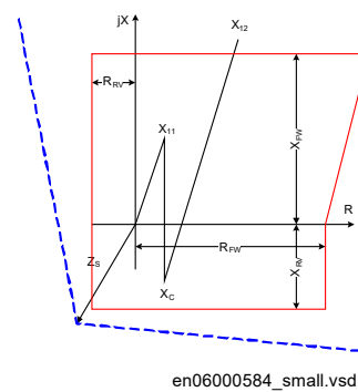
Figure 106: Quadrilateral characteristic with separate impedance and directional measurement
