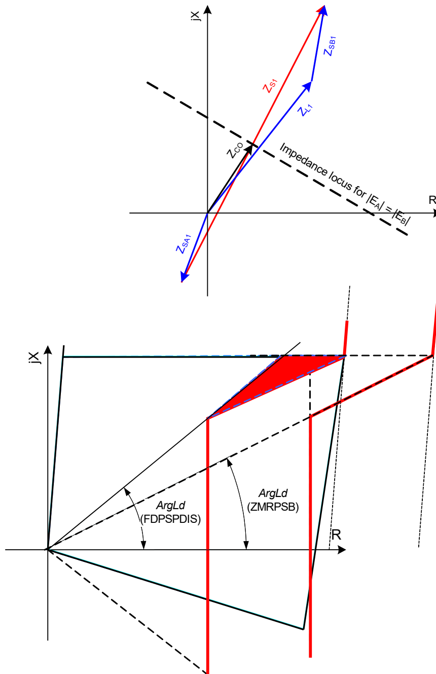
Figure 235: Impedance diagrams with corresponding impedances under consideration
