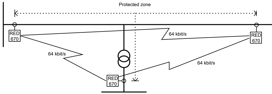
Figure 41: Transformer situated in tap
