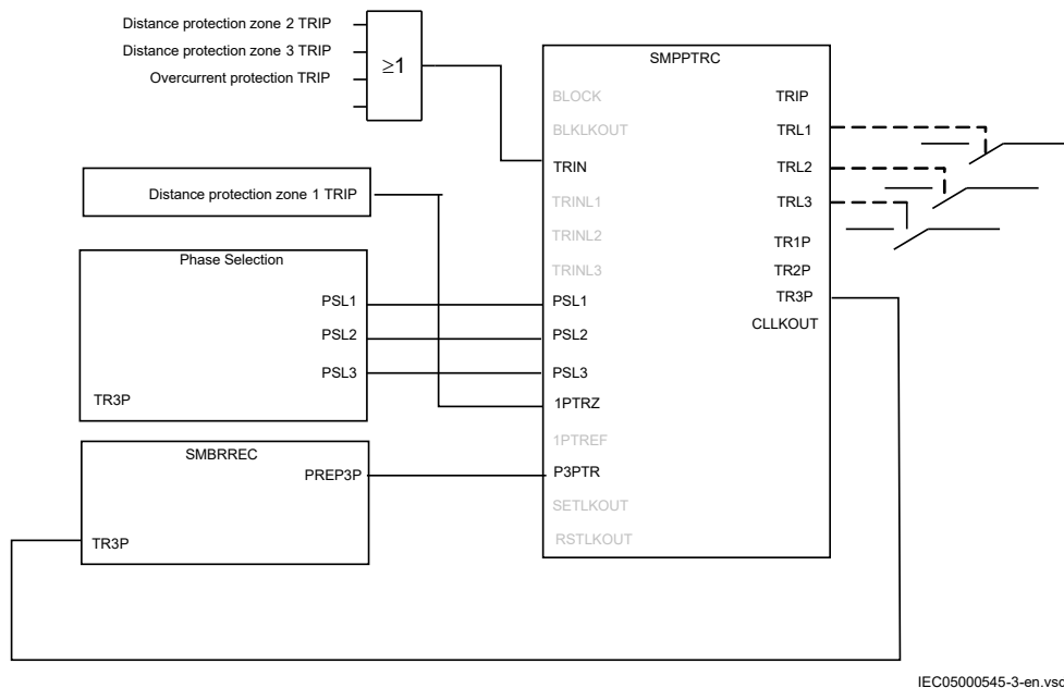
Figure 386: The trip logic function SMPPTRC used for single-phase tripping application
