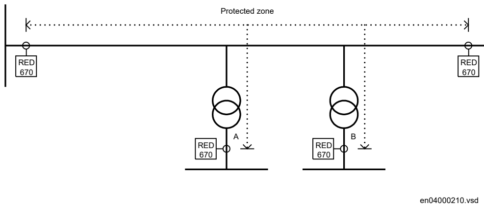
Figure 54: Two two-winding transformers in the protected zone
