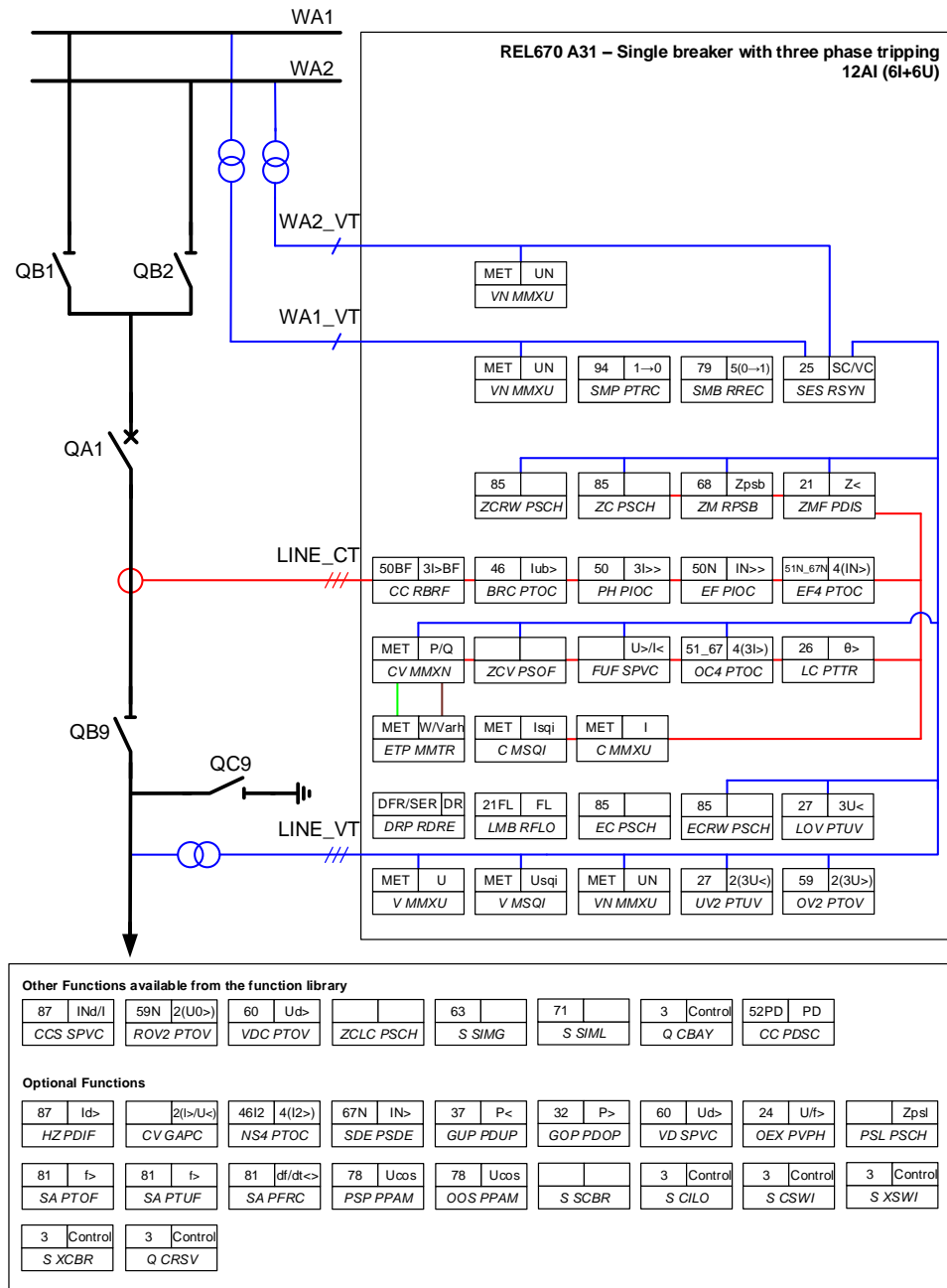
Figure 3: Configuration diagram for configuration A31
