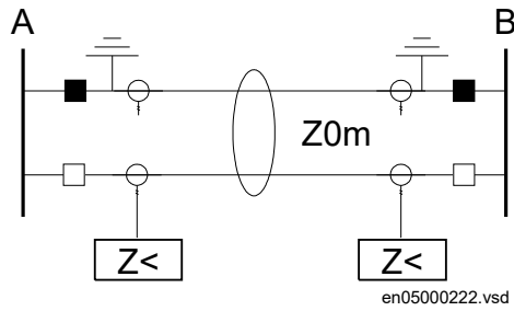
Figure 71: The parallel line is out of service and earthed
