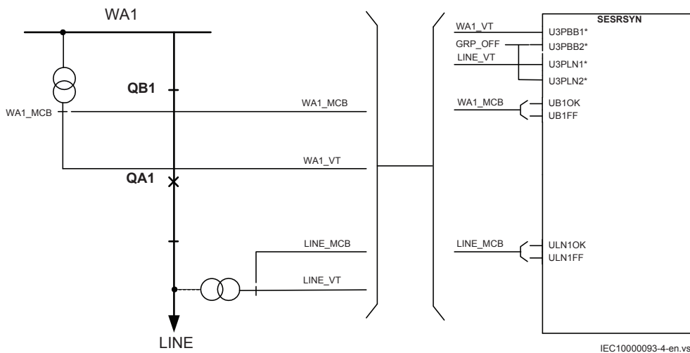
Figure 306: Connection of SESRSYN function block in a single busbar arrangement
