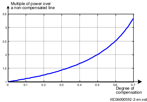
Figure 208: Increase in power transfer over a transmission line depending on degree of series compensation
