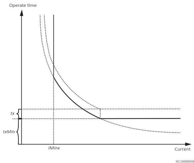
Figure 277: Minimum operate current and operation time for inverse time characteristics
