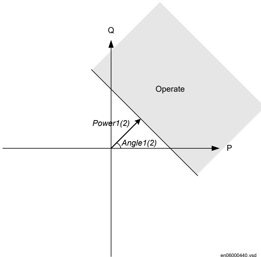
Figure 290: Overpower mode
