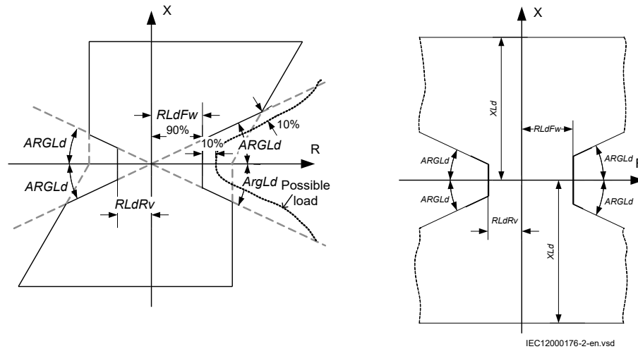
Figure 191: Load impedance limitation with load encroachment
