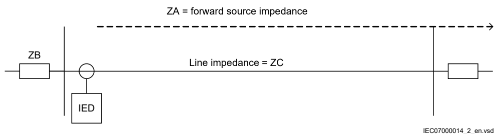
Figure 243: Line application of pole slip protection
