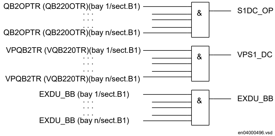
Figure 345: Signals from any bays in section B1 to a bus-section disconnecter
