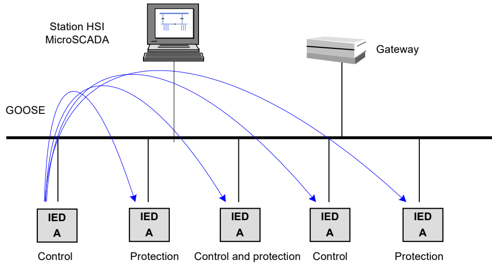
Figure 402: Example of a broadcasted GOOSE message
