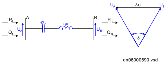
Figure 207: Transmission line with series capacitor
