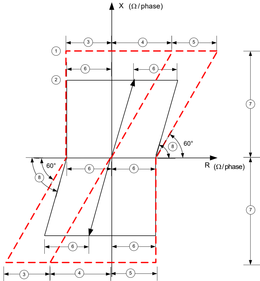
Figure 115: Relation between distance protection (ZMQPDIS) and FDPSPDIS characteristic for phase-to-phase fault for \phi_{line} > 60^\circ (setting parameters in italic )
