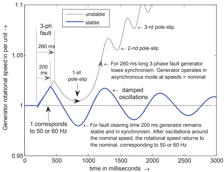
Figure 250: Stable and unstable case. For the fault clearing time t_{cl} = 200\text{ ms} , the generator remains in synchronism, for t_{cl} = 260\text{ ms} , the generator loses step.
