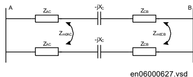
Figure 107: Double circuit, parallel operating line
