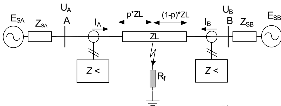
Figure 158: Influence of fault current infeed from remote line end
