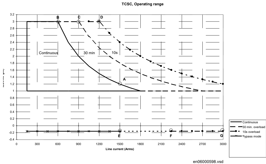
Figure 88: Operating range of a TCSC installed for damping of power oscillations (example)
