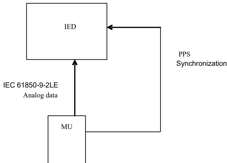
Figure 410: Setting example when MU is the synchronizing source
