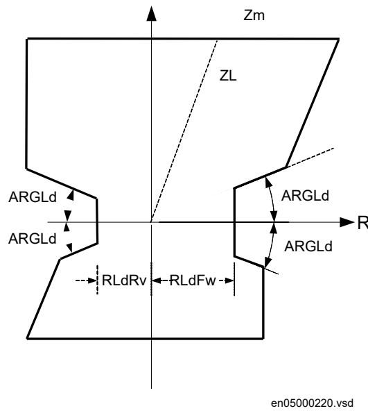
Figure 197: Characteristic for zone measurement for a long line [6]
