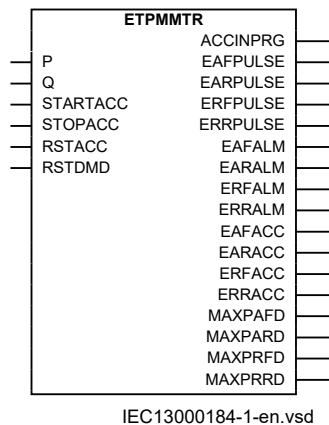
Figure 400: Connection of energy calculation and demand handling function ETPMMTR to the measurements function (CVMMXN)
