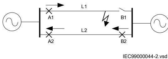
Figure 374: Current distribution for a fault close to B side when breaker B1 has opened
