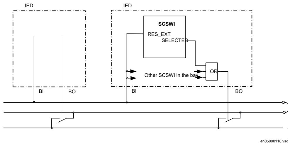
Figure 322: Application principles for reservation with external wiring
