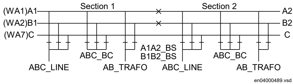
Figure 338: Busbars divided by bus-section circuit breakers
