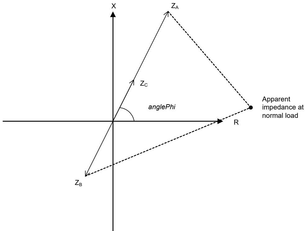
Figure 244: Impedances to be set for pole slip protection
