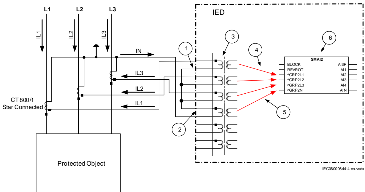
Figure 16: Star connected three-phase CT set with its star point away from the protected object and the residual/neutral current connected to the IED
