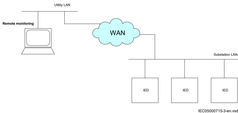
Figure 414: SPA communication structure for a remote monitoring system via a substation LAN, WAN and utility LAN
