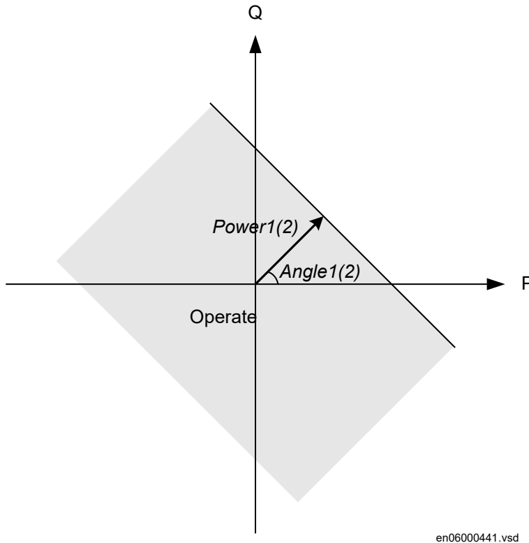
Figure 287: Underpower mode
