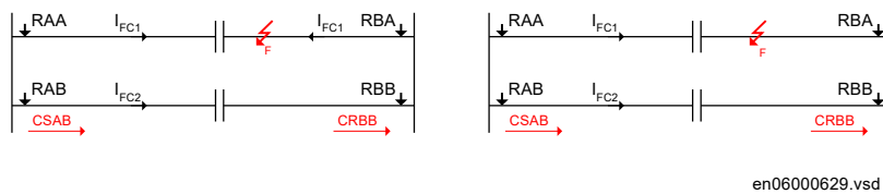
Figure 109: Current reversal phenomenon on parallel operating circuits
