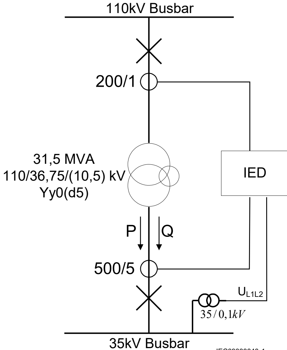
Figure 393: Single line diagram for transformer application
