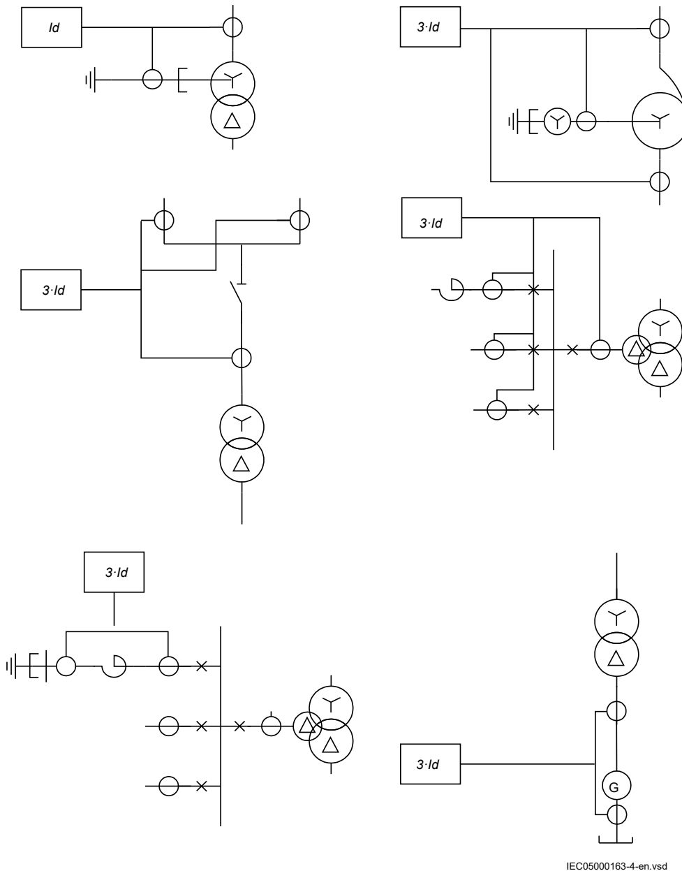
Figure 32: Different applications of a 1Ph High impedance differential protection HZPDIF function
