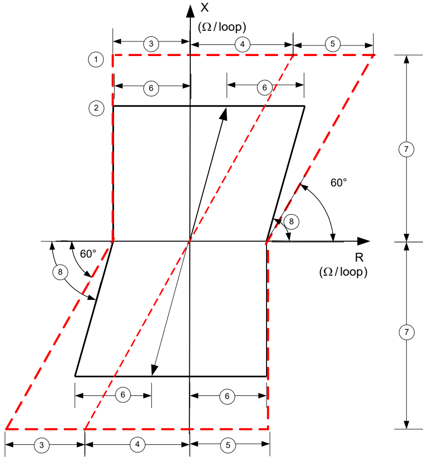
Figure 114: Relation between distance protection phase selection (FDPSDIS) and impedance zone (ZMQPDIS) for phase-to-earth fault \phi_{loop} > 60^\circ (setting parameters in italic)
