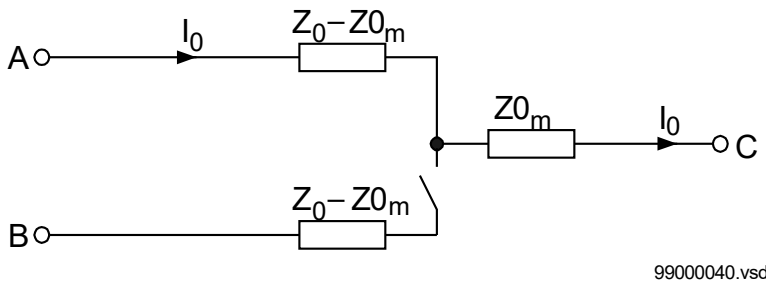
Figure 74: Equivalent zero-sequence impedance circuit for a double-circuit line with one circuit disconnected and not earthed
