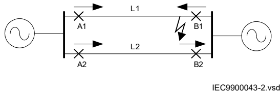
Figure 373: Current distribution for a fault close to B side when all breakers are closed
