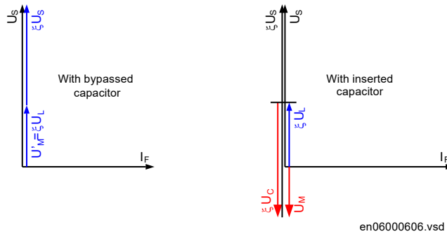
Figure 210: Phasor diagrams of currents and voltages for the bypassed and inserted series capacitor during voltage inversion
