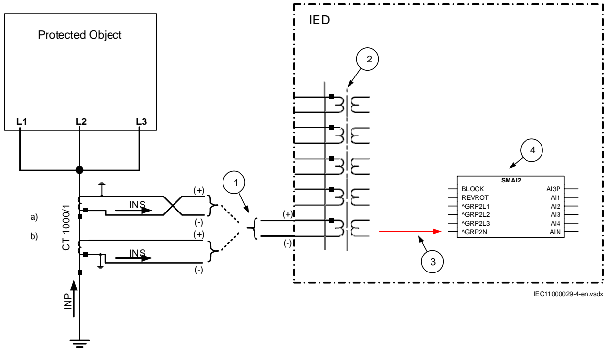
Figure 19: Connections for single-phase CT input
