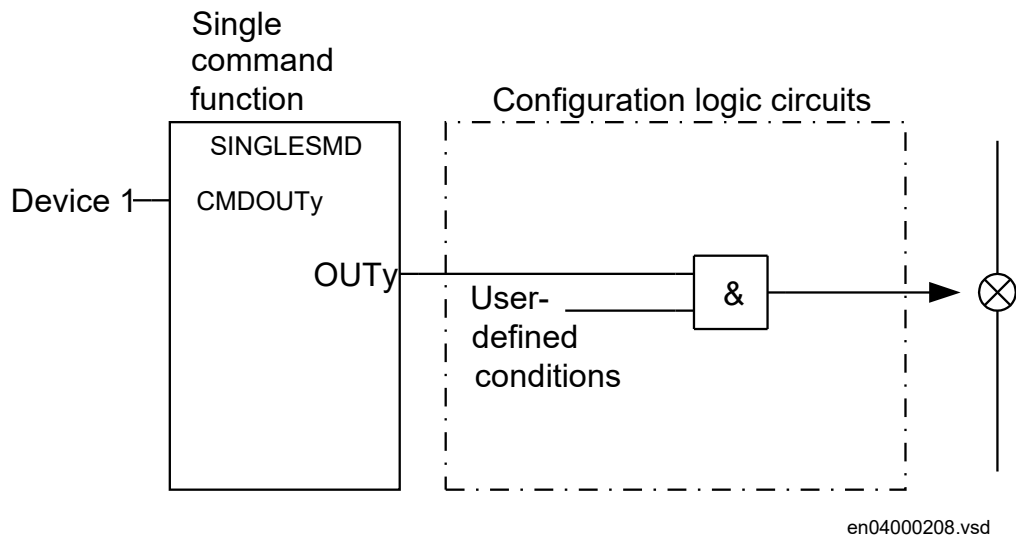
Figure 367: Application example showing a logic diagram for control of external devices via configuration logic circuits
