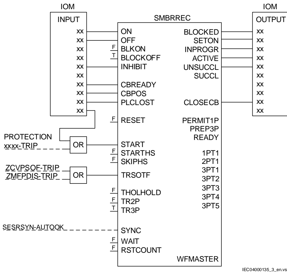
Figure 315: Example of I/O-signal connections at a three-phase reclosing function
