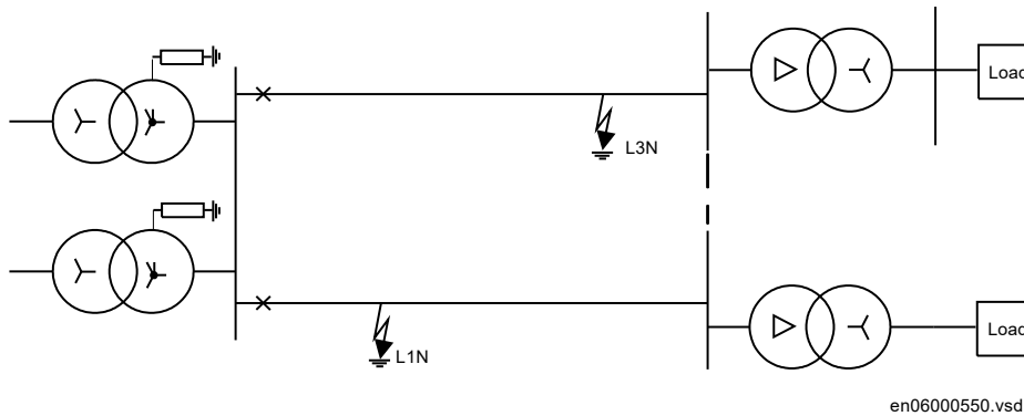
Figure 251: An occurring cross-country fault on different feeders in a sub-transmission network, high impedance (resistance, reactance) earthed
