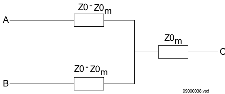
Figure 70: Equivalent zero sequence impedance circuit of the double-circuit, parallel, operating line with a single phase-to-earth-fault at the remote busbar
