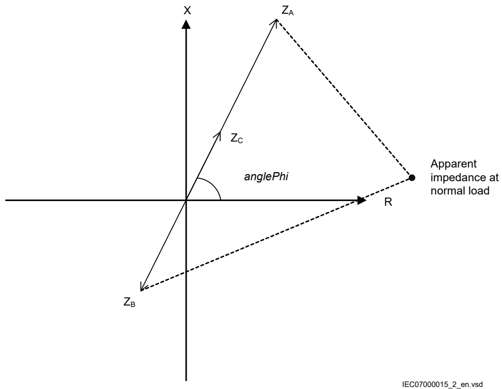
Figure 247: Impedances to be set for pole slip protection PSPPPAM
