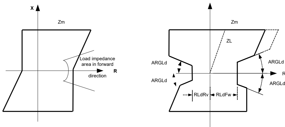
Figure 67: Load encroachment phenomena and shaped load encroachment characteristic
