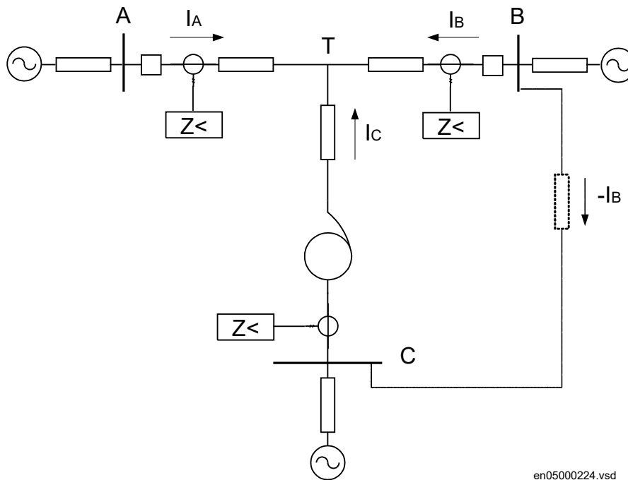
Figure 75: Example of tapped line with Auto transformer
