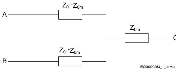
Figure 199: Equivalent zero sequence impedance circuit of the double-circuit, parallel, operating line with a single phase-to-earth fault at the remote busbar
