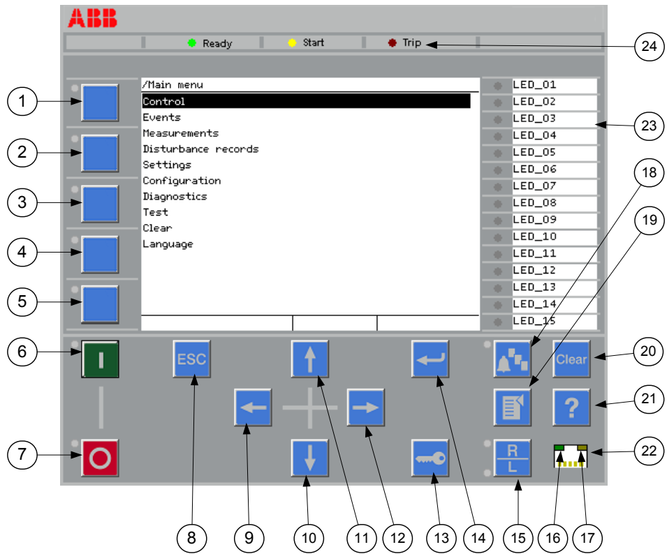
Figure 30: L1HMI keypad with object control, navigation and command push-buttons and RJ-45 communication port
