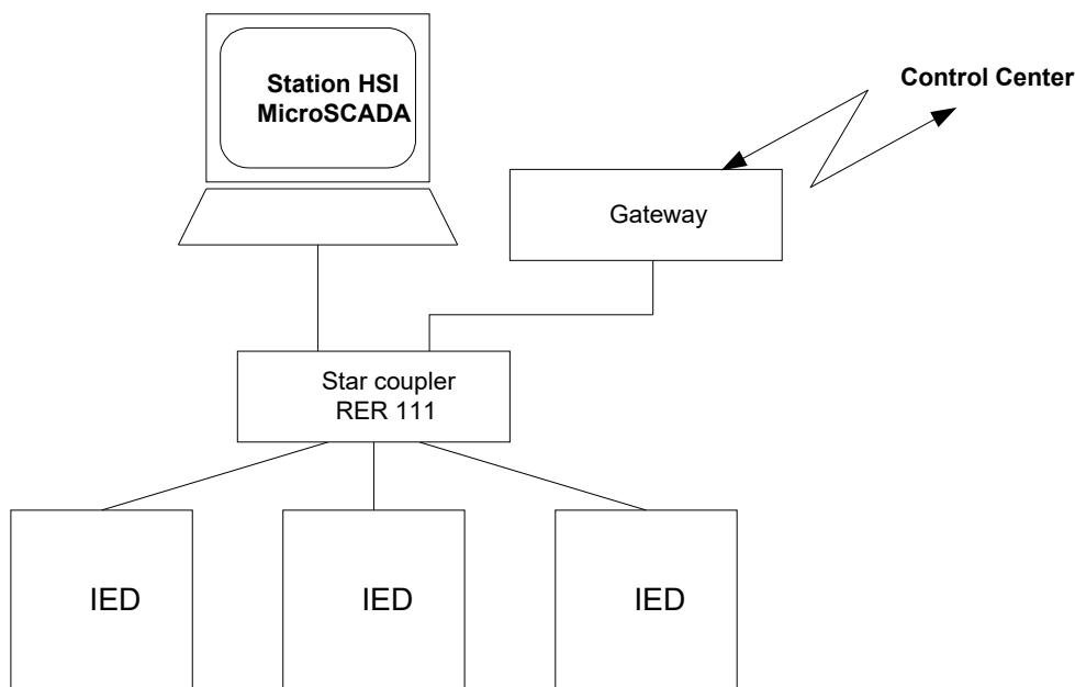
Figure 413: Example of LON communication structure for a substation automation system
