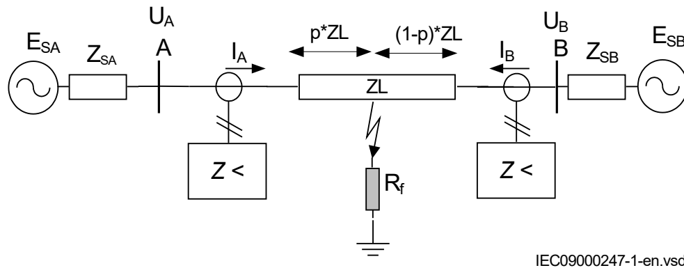
Figure 195: Influence of fault current infeed from remote line end
