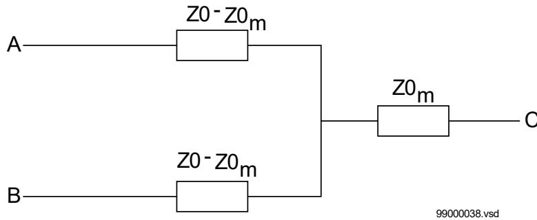
Figure 148: Equivalent zero sequence impedance circuit of the double-circuit, parallel, operating line with a single phase-to-earth fault at the remote busbar
