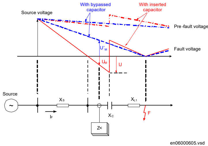
Figure 209: Voltage inversion on series compensated line
