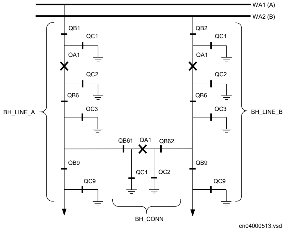
Figure 363: Switchyard layout 1 1/2 breaker
