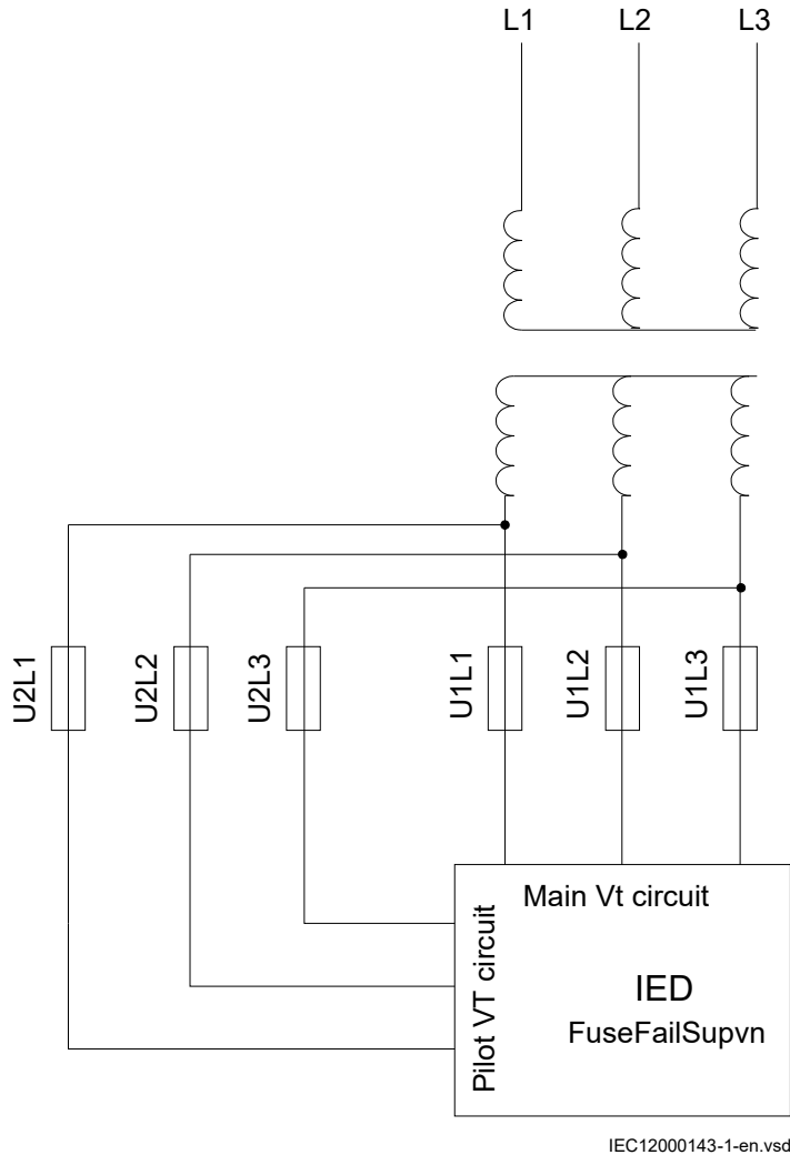
Figure 301: Application of VDSPVC
