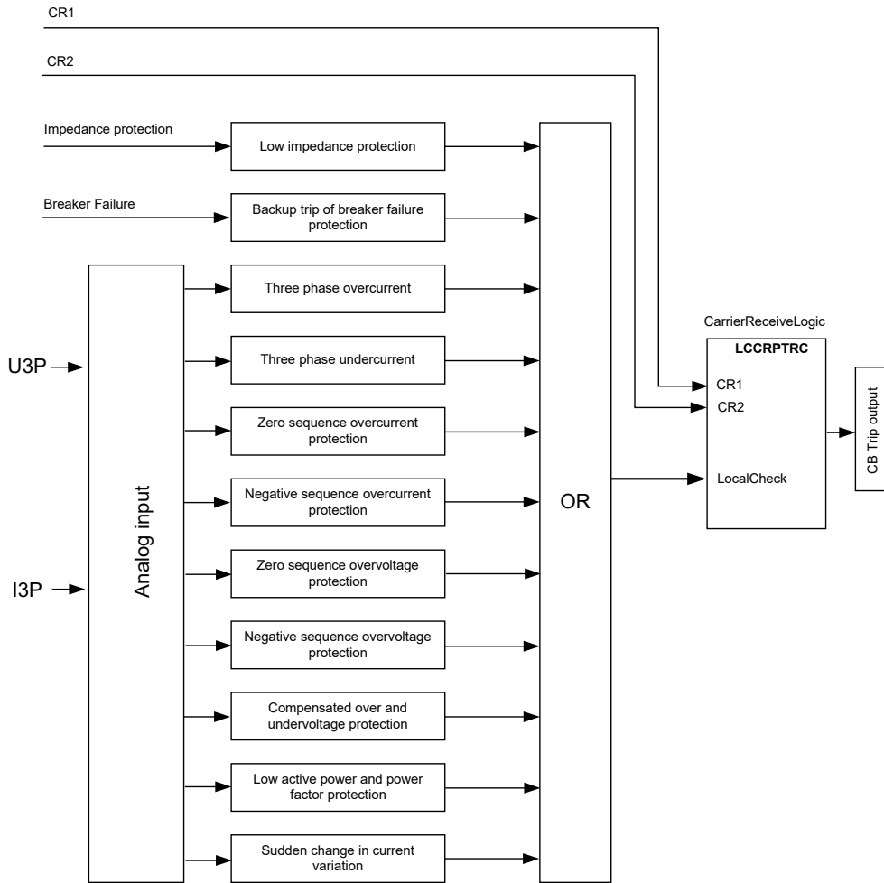
Figure 382: DTT scheme
