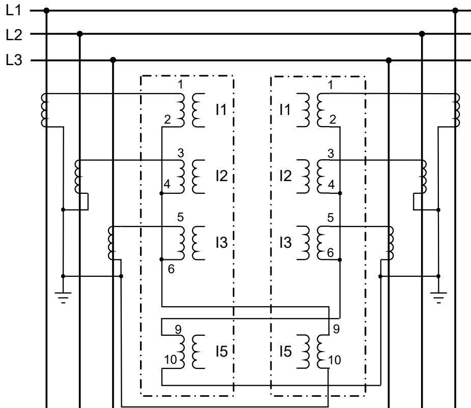
Figure 399: Example of connection of parallel line IN for Fault locator LMBRFLO
