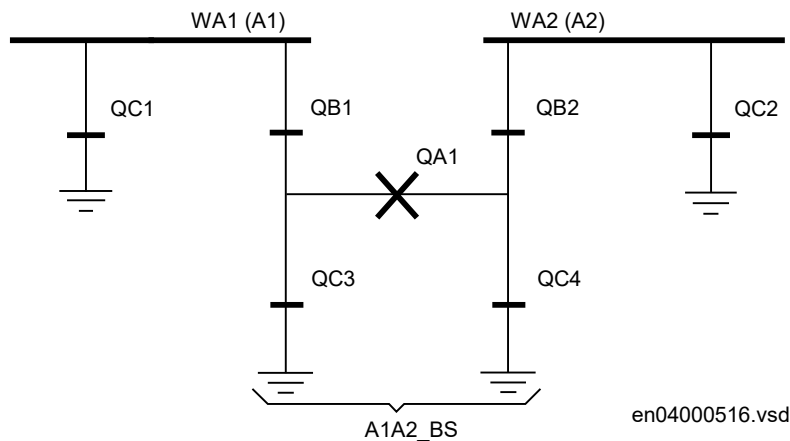
Figure 337: Switchyard layout A1A2_BS
