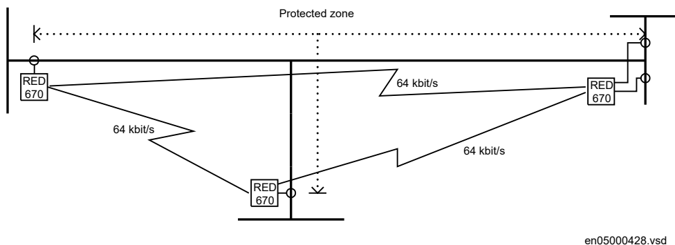
Figure 40: Line protection with 1½ breaker configurations, fed from two CTs
