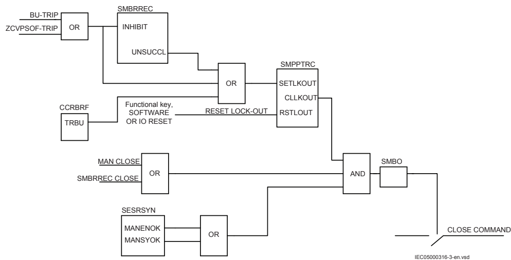
Figure 314: Lock-out arranged with internal logic with manual closing going through in IED
