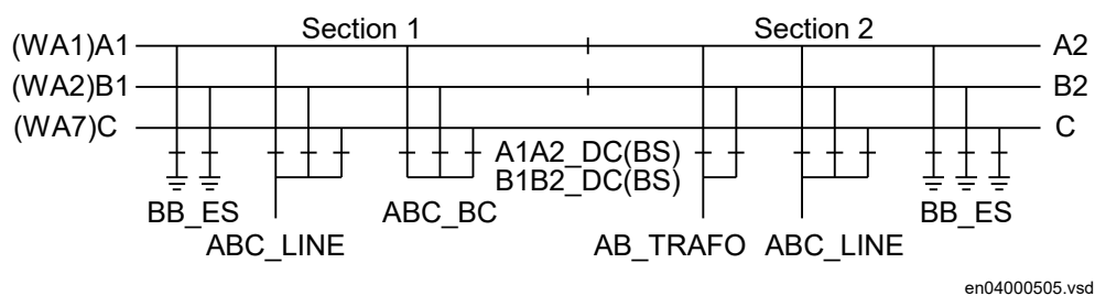
Figure 354: Busbars divided by bus-section disconnectors (circuit breakers)
