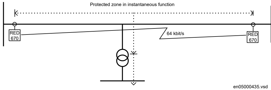
Figure 42: Line tap with a small power transformer, the currents of which are not measured, and consequently contribute to a (false) differential current
