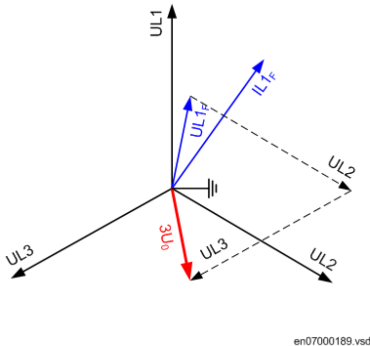
Figure 294: Earth fault in Direct earthed system
