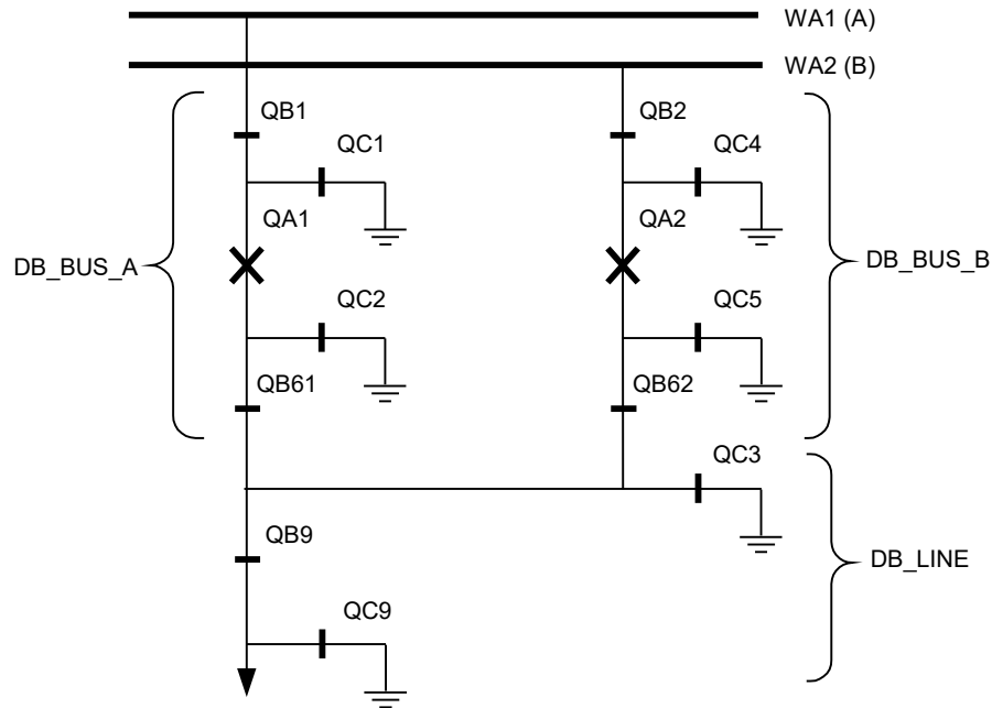
Figure 362: Switchyard layout double circuit breaker
