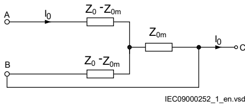
Figure 186: Equivalent zero sequence impedance circuit for the double-circuit line that operates with one circuit disconnected and earthed at both ends
