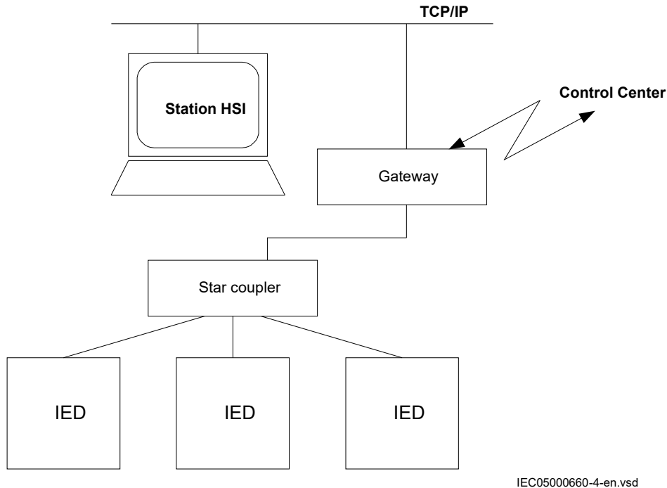
Figure 415: Example of IEC 60870-5-103 communication structure for a substation automation system
