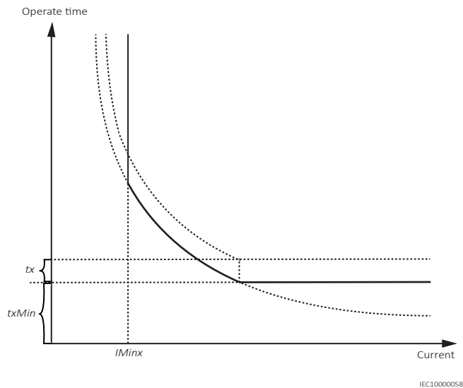
Figure 260: Minimum operate current and operate time for inverse time characteristics
