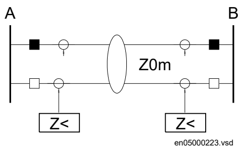
Figure 151: Parallel line is out of service and not earthed.
