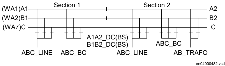
Figure 331: Busbars divided by bus-section disconnectors (circuit breakers)
