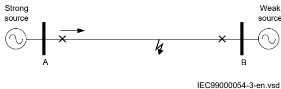
Figure 379: Initial condition for weak-end infeed
