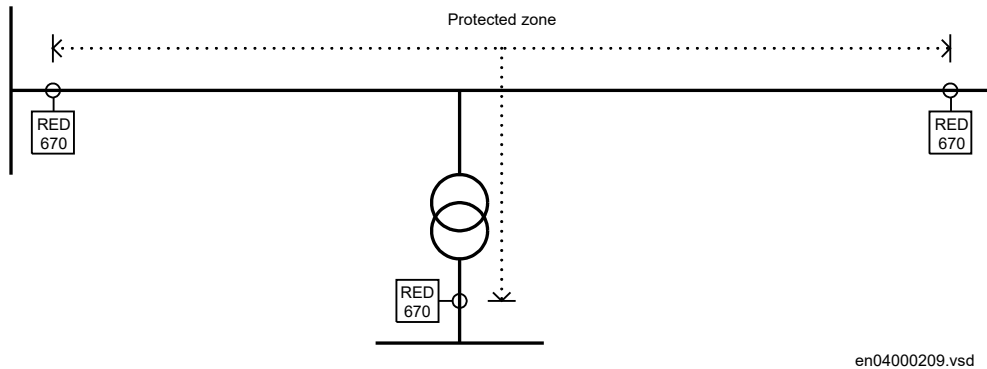
Figure 53: One two-winding transformer in the protected zone
