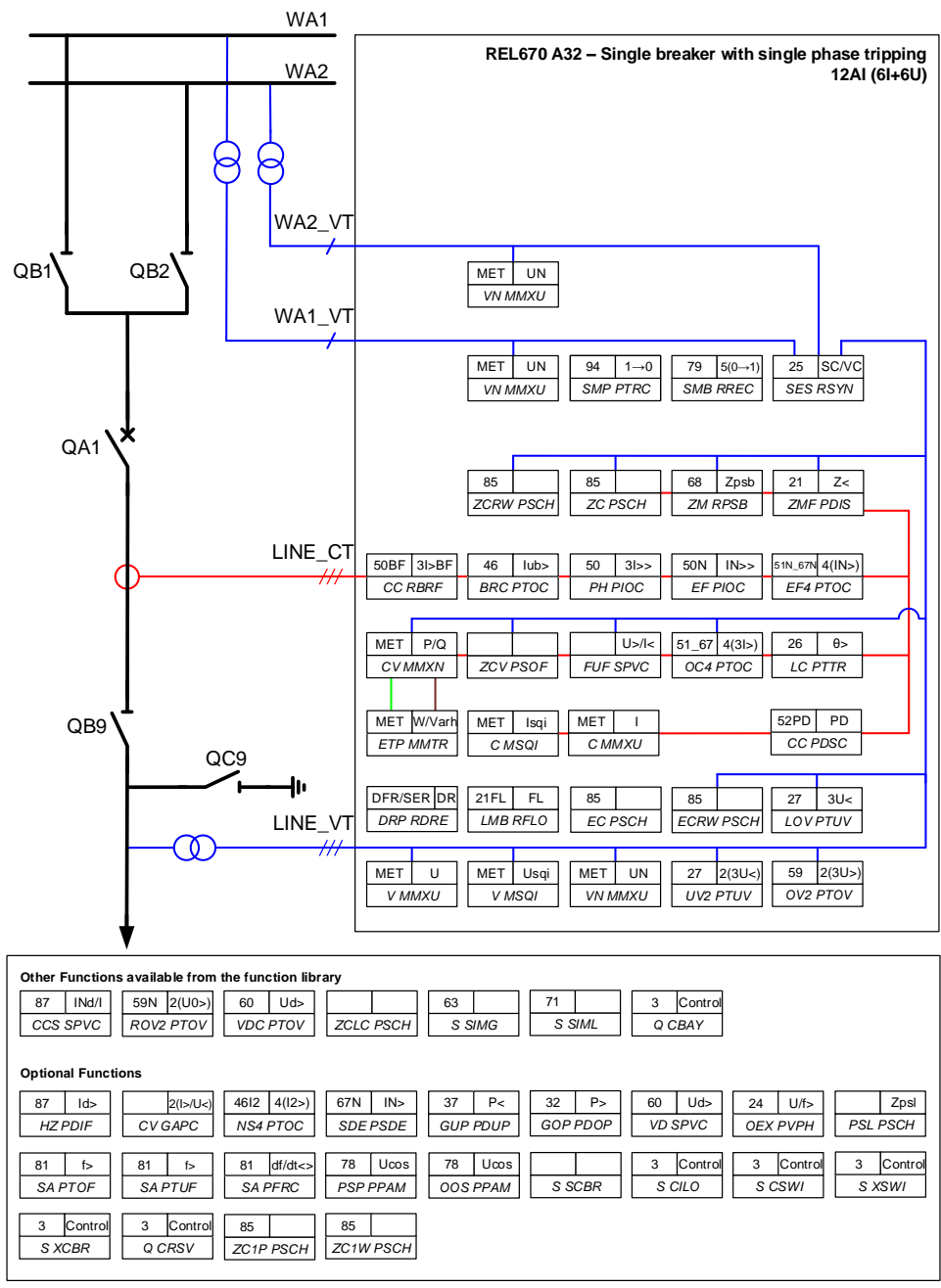
Figure 4: Configuration diagram for configuration A32
