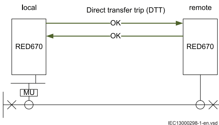
Figure 407: Normal operation
