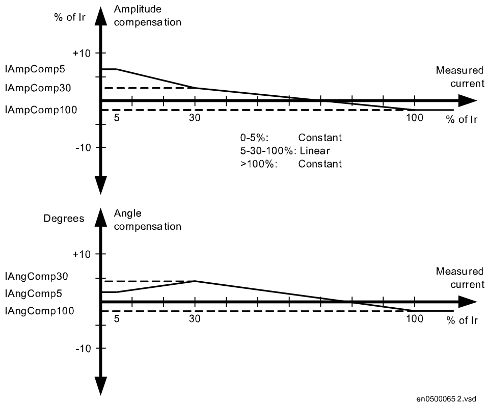
Figure 391: Calibration curves
