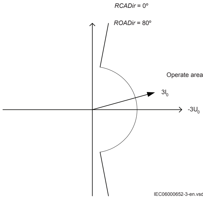
Figure 283: Characteristic for RCADir = 0^\circ and ROADir = 80^\circ
