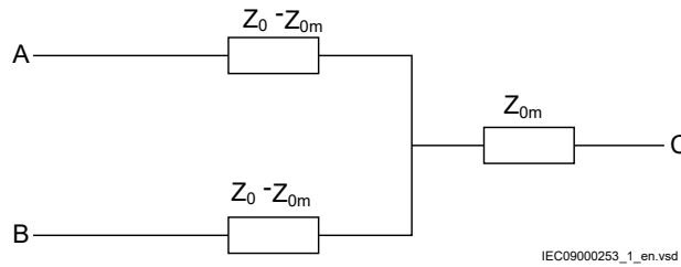
Figure 161: Equivalent zero sequence impedance circuit of the double-circuit, parallel, operating line with a single phase-to-earth fault at the remote busbar.
