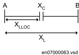
Figure 112: Simplified single line diagram of series capacitor located at X_{LLOC} ohm from A station
