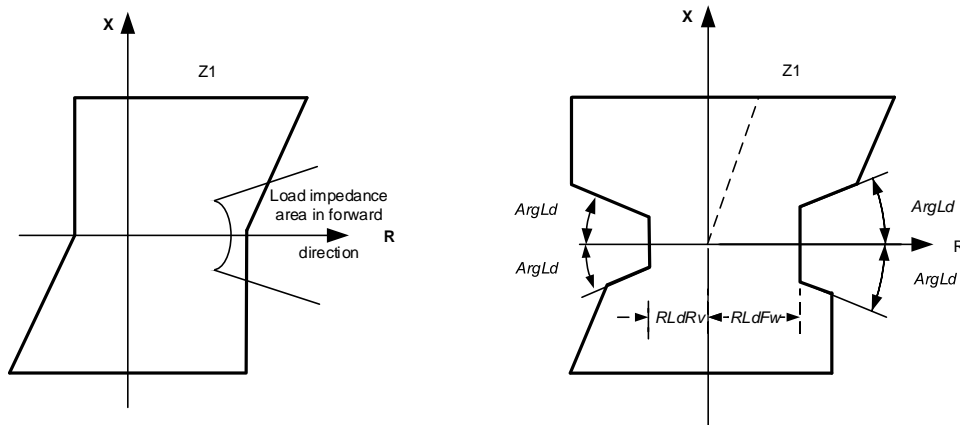
Figure 159: Load encroachment phenomena and shaped load encroachment characteristic defined in Phase selection and load encroachment function (FRPSPDIS)
