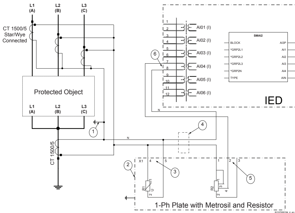
Figure 36: CT connections for restricted earth fault protection
