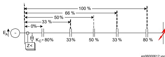
Figure 214: Typical locations of capacitor banks on series compensated line
