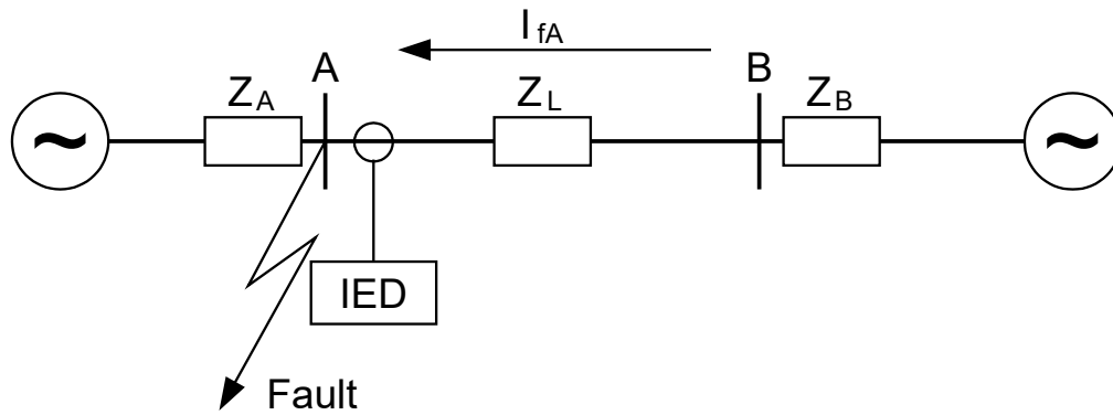
Figure 256: Through fault current from B to A: I_{fA}
