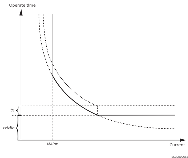
Figure 267: Minimum operate current and operate time for inverse time characteristics
