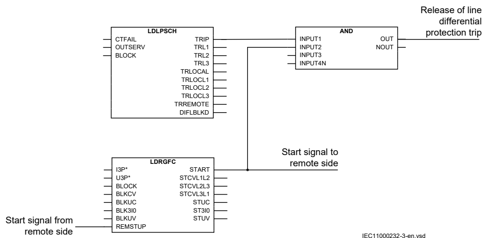
Figure 64: Local release criterion configuration for line differential protection
