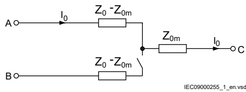
Figure 165: Equivalent zero sequence impedance circuit for a double-circuit line with one circuit disconnected and not earthed.
