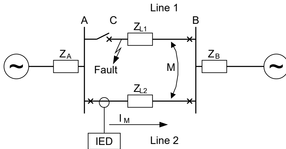
Figure 258: Two parallel lines. Influence from parallel line to the through fault current: I_M
