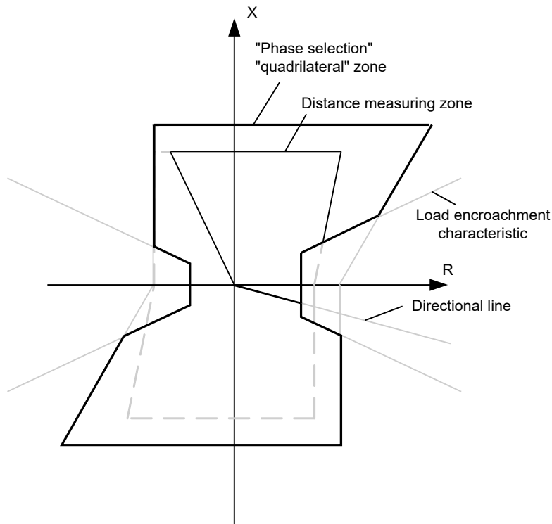
Figure 170: Operation characteristic in forward direction when load encroachment is enabled
