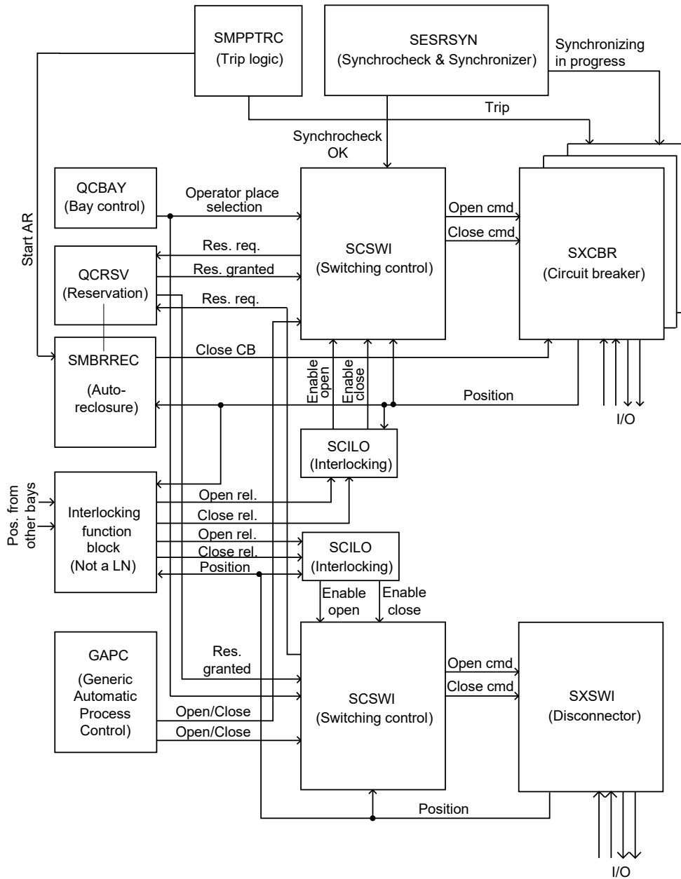
Figure 324: Example overview of the interactions between functions in a typical bay
