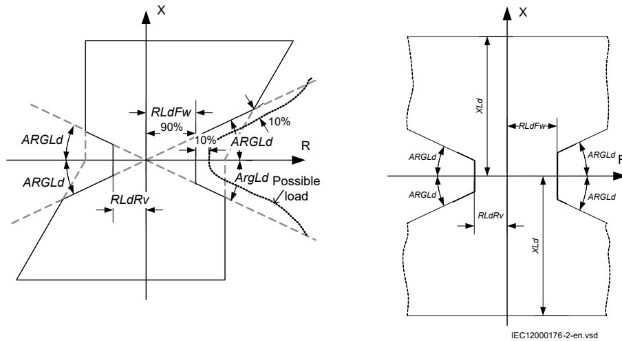
Figure 231: Load impedance limitation with load encroachment
