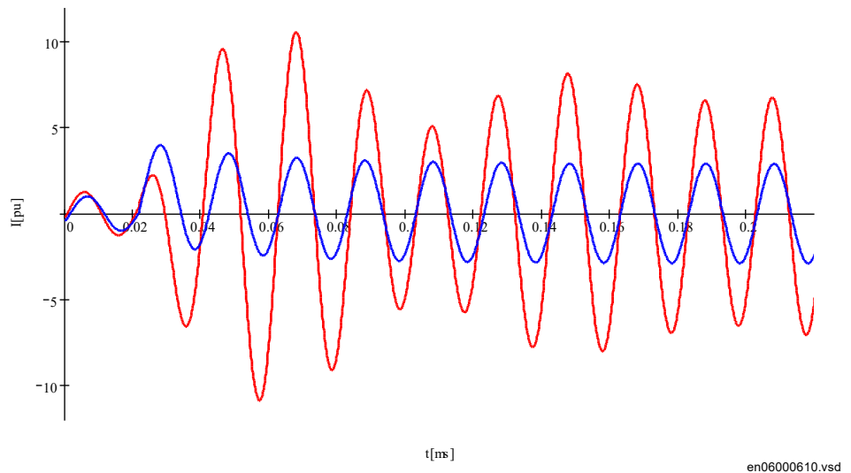
Figure 94: Short circuit currents for the fault at the end of 500 km long 500 kV line without and with SC
