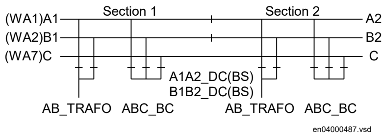
Figure 336: Busbars divided by bus-section disconnectors (circuit breakers)
