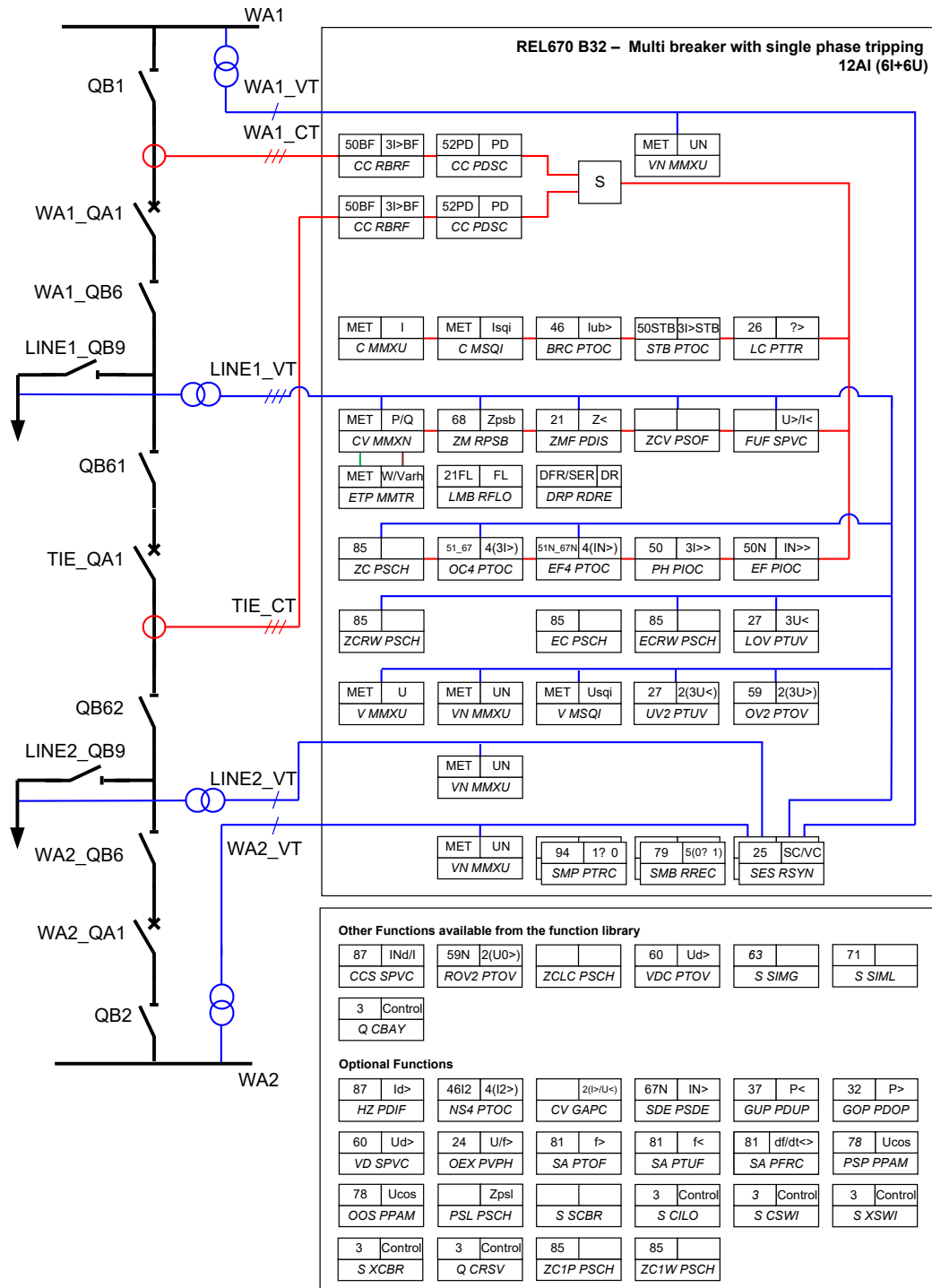
Figure 6: Configuration diagram for configuration B32
