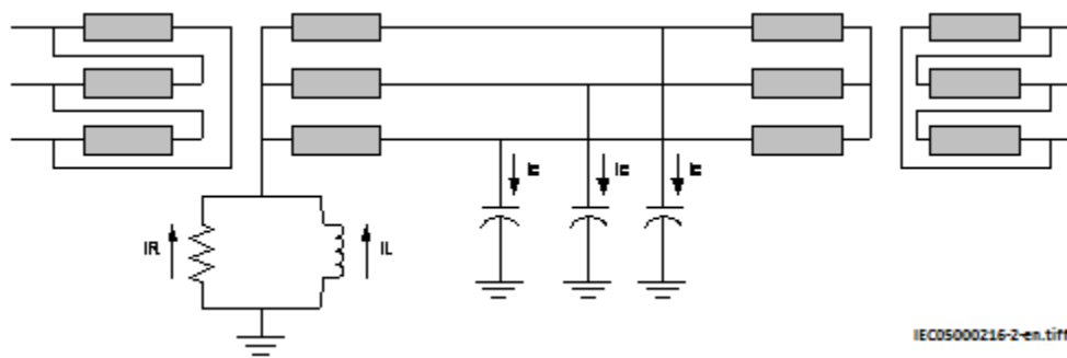
Figure 118: High impedance earthing network
