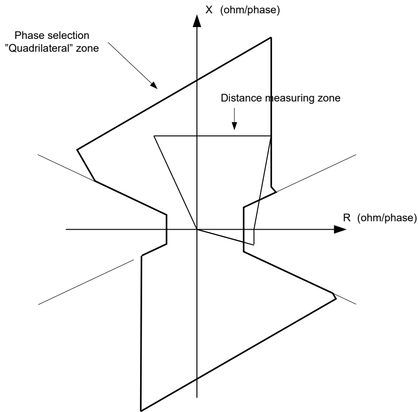
Figure 171: Operation characteristic for FRPSPDIS in forward direction for three-phase fault, ohm/phase domain
