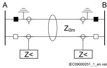
Figure 185: The parallel line is out of service and earthed
