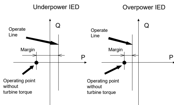
Figure 289: Reverse power protection with underpower IED and overpower IED
