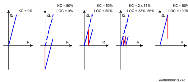
Figure 97: Apparent impedances seen by distance IED for different SC locations and spark gaps used for overvoltage protection
