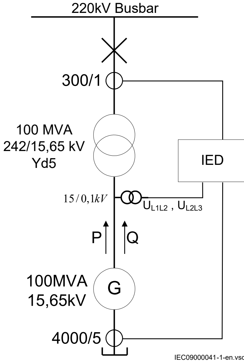
Figure 394: Single line diagram for generator application
