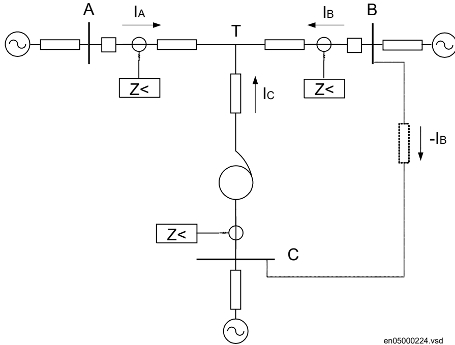
Figure 153: Example of tapped line with Auto transformer
