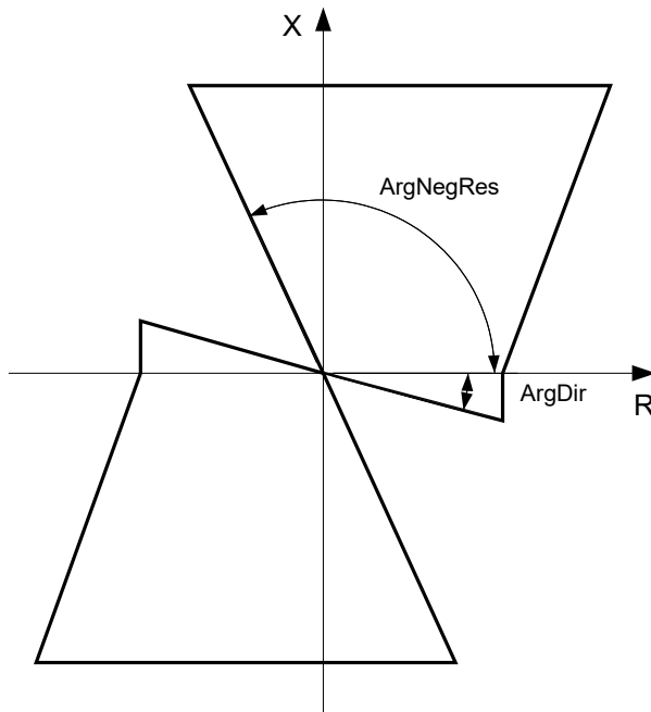
Figure 130: Setting angles for discrimination of forward and reverse fault in Directional impedance quadrilateral function ZDRDIR
