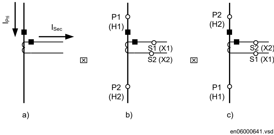
Figure 13: Commonly used markings of CT terminals
