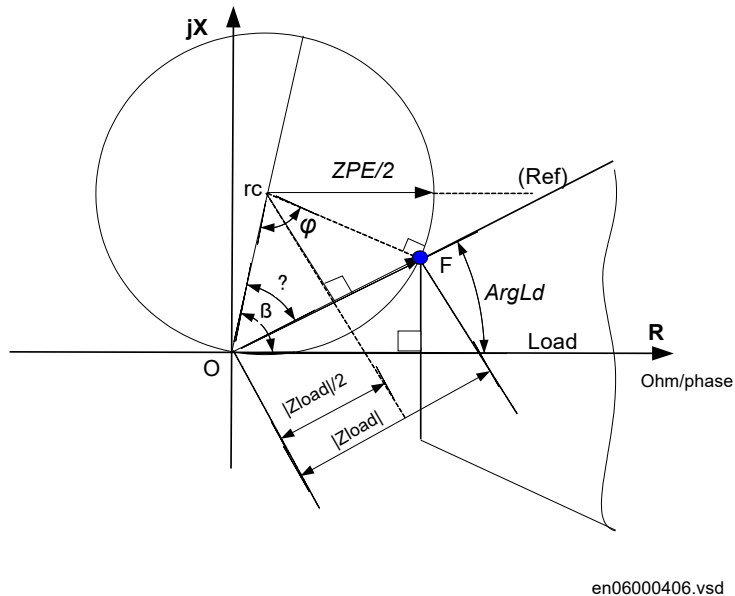
Figure 142: Definition of the setting condition to avoid load encroachment for earth-fault loop
