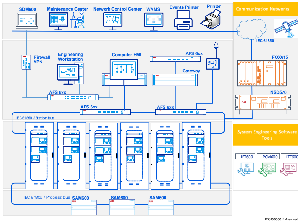
Figure 405: Example of a station configuration with separated process bus and station bus
