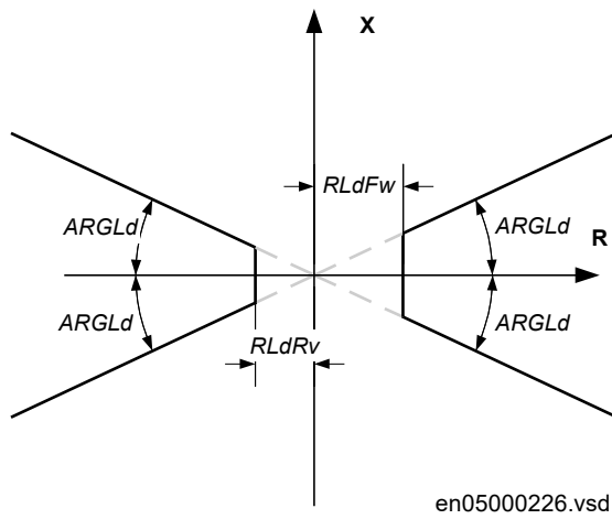
Figure 155: Load encroachment characteristic
