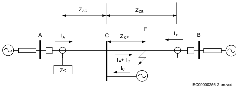
Figure 228: Setting of overreaching zone
