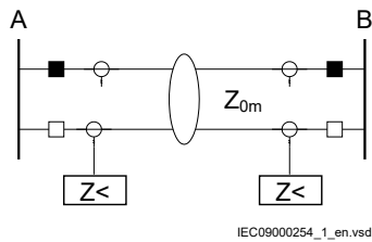
Figure 187: Parallel line is out of service and not earthed
