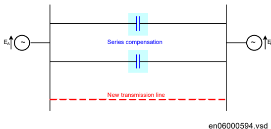
Figure 84: Series compensation is an important alternative to new transmission lines
