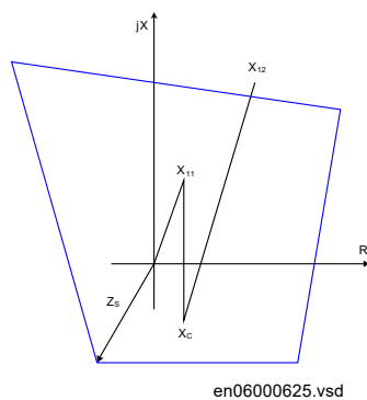
Figure 105: Cross-polarized quadrilateral characteristic
