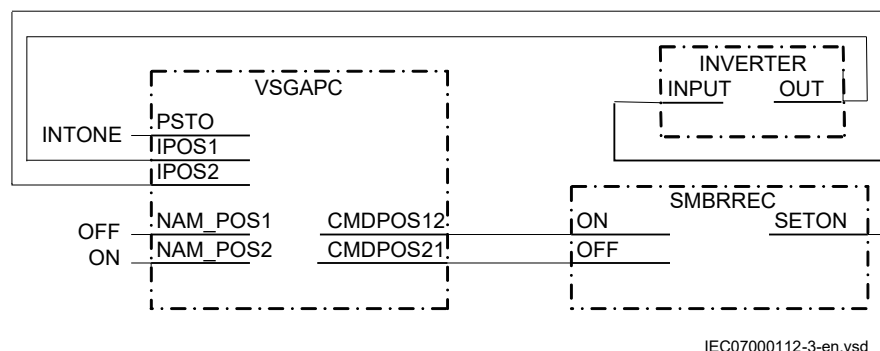
Figure 364: Control of Autorecloser from local HMI through Selector mini switch
