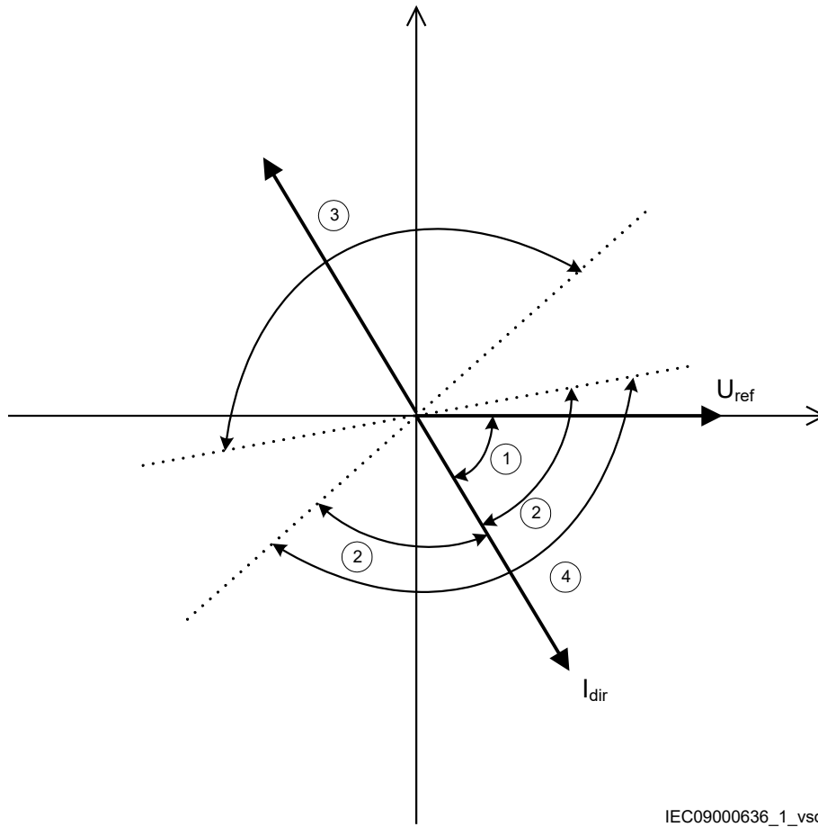
Figure 259: Directional function characteristic
