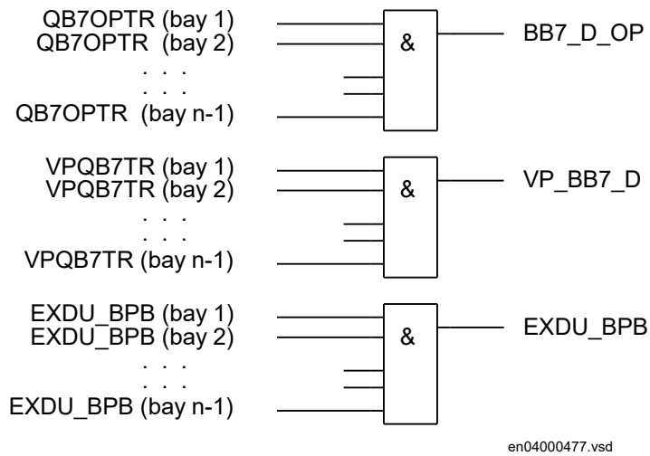
Figure 326: Signals from bypass busbar in line bay n
