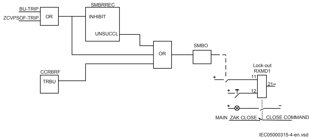
Figure 313: Lock-out arranged with an external Lock-out relay
