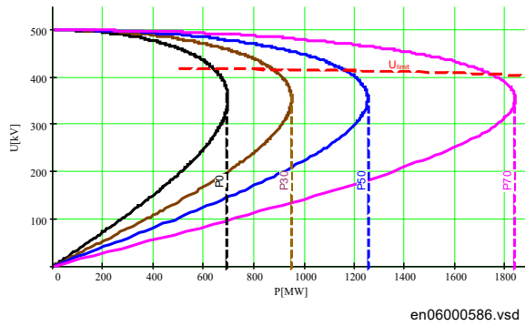
Figure 206: Voltage profile for a simple radial power line with 0, 30, 50 and 70% of compensation
