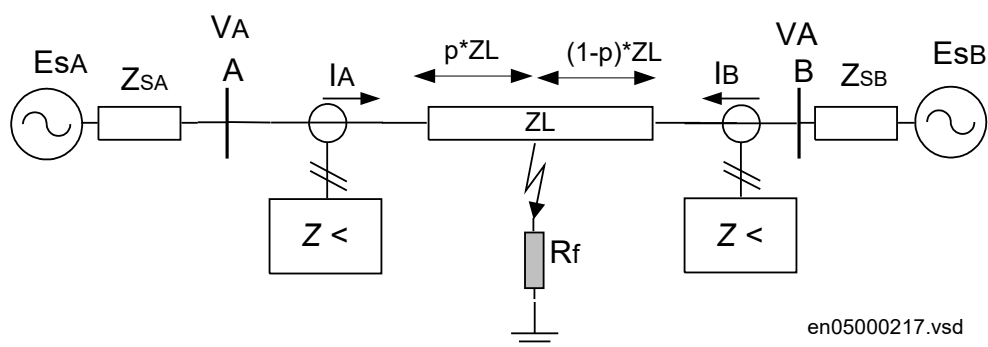
Figure 66: Influence of fault infeed from remote end
