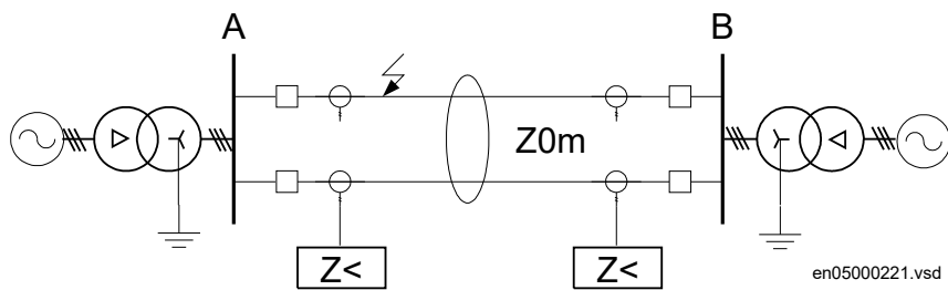
Figure 69: Class 1, parallel line in service
