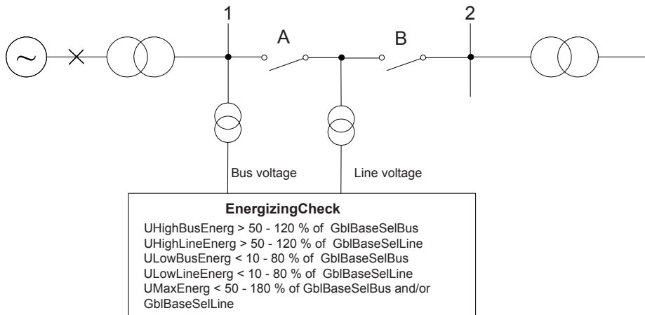
Figure 304: Principle for the energizing check function
