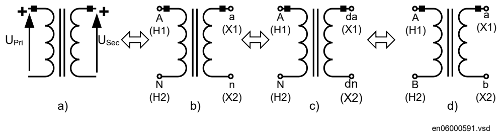
Figure 20: Commonly used markings of VT terminals
