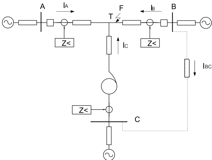
Figure 204: Example of tapped line with Auto transformer
