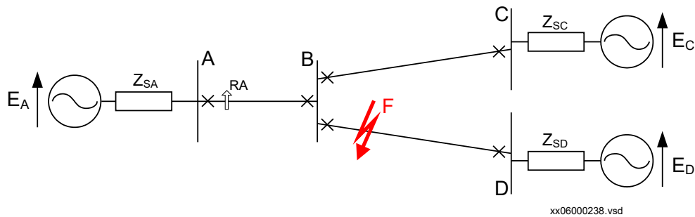
Figure 236: Fault on adjacent line and its clearance causes power swinging between sources A and C
