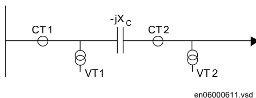
Figure 213: Possible positions of instrument transformers relative to line end series capacitor
