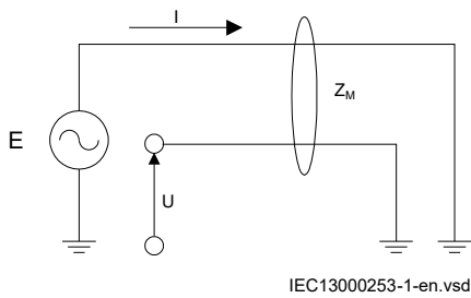
Figure 136: Mutual coupling
