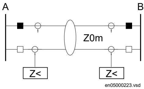
Figure 73: Parallel line is out of service and not earthed
