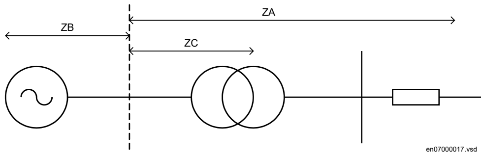
Figure 246: Generator application of pole slip protection
