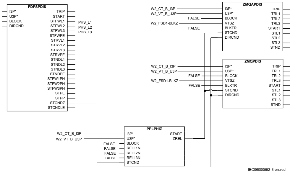
Figure 253: The connection of Phase preference logic function PPLPHIZ between Distance protection zone, quadrilateral characteristic ZMQPDIS and ZMQAPDIS and Phase selection with load encroachment, quadrilateral characteristic function FDPSPDIS
