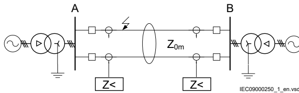
Figure 183: Class 1, parallel line in service
