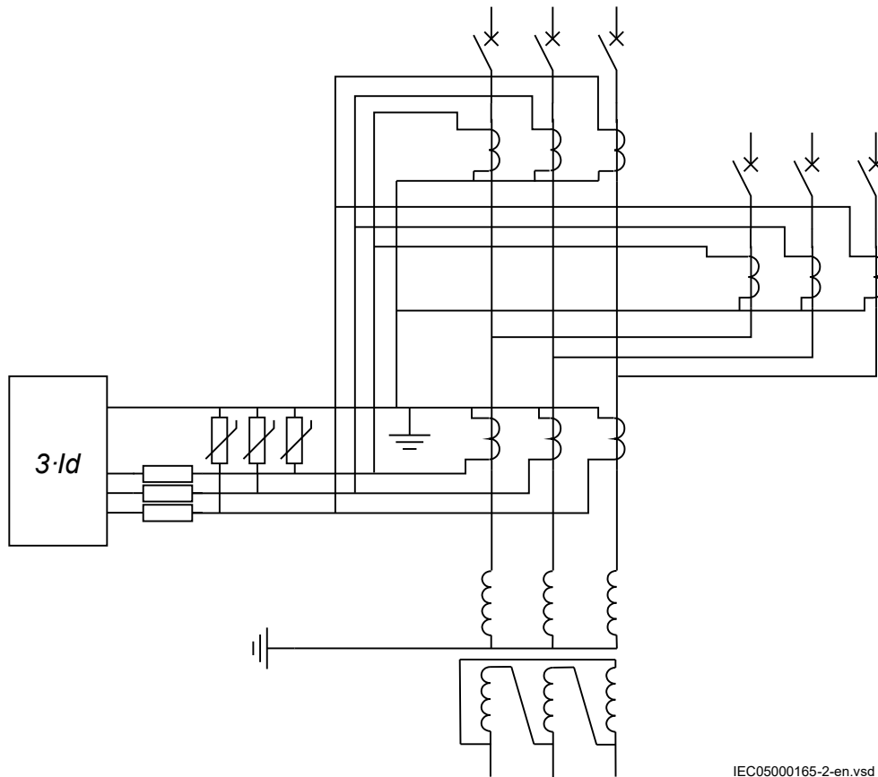
Figure 37: The protection scheme utilizing the high impedance function for the T-feeder
