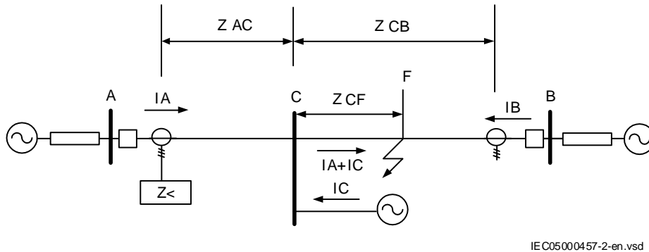
Figure 154: Setting of overreaching zone
