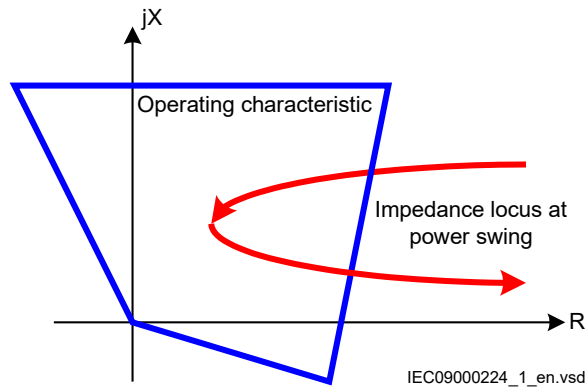
Figure 233: Impedance plane with Power swing detection operating characteristic and impedance locus at power swing
