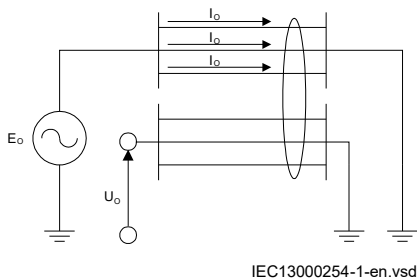
Figure 137: Mutual coupling of two three-phase lines
