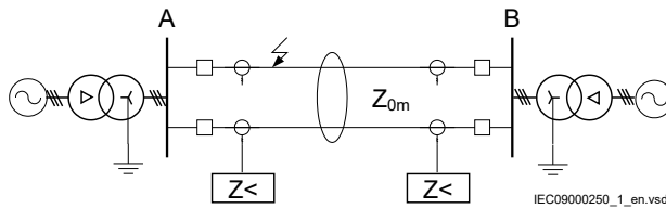
Figure 122: Class 1, parallel line in service
