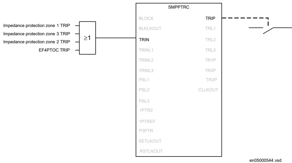
Figure 385: Tripping logic SMPPTRC is used for a simple three-phase tripping application
