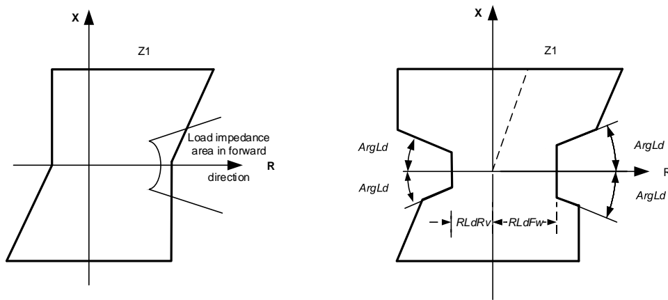
Figure 120: Load encroachment phenomena and shaped load encroachment characteristic defined in Phase selection with load encroachment function FDPSPDIS
