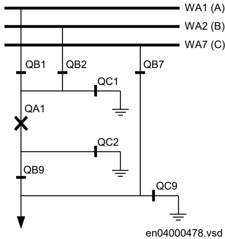
Figure 325: Switchyard layout ABC_LINE
