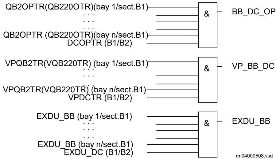
Figure 357: Signals from any bays in section B1 to a busbar earthing switch in the same section
