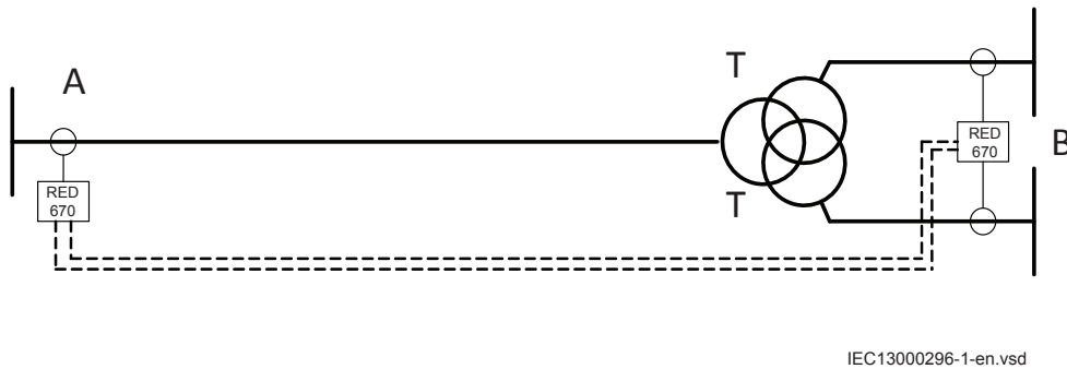
Figure 63: Three-winding transformer in the zone
