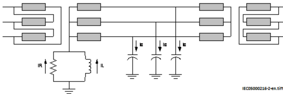
Figure 157: High impedance earthing network.
