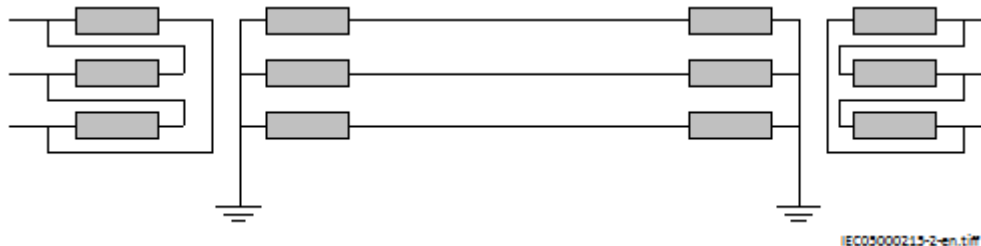
Figure 131: Solidly earthed network
