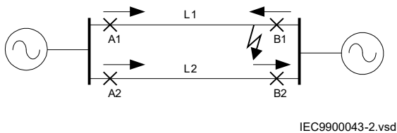
Figure 377: Current distribution for a fault close to B side when all breakers are closed
