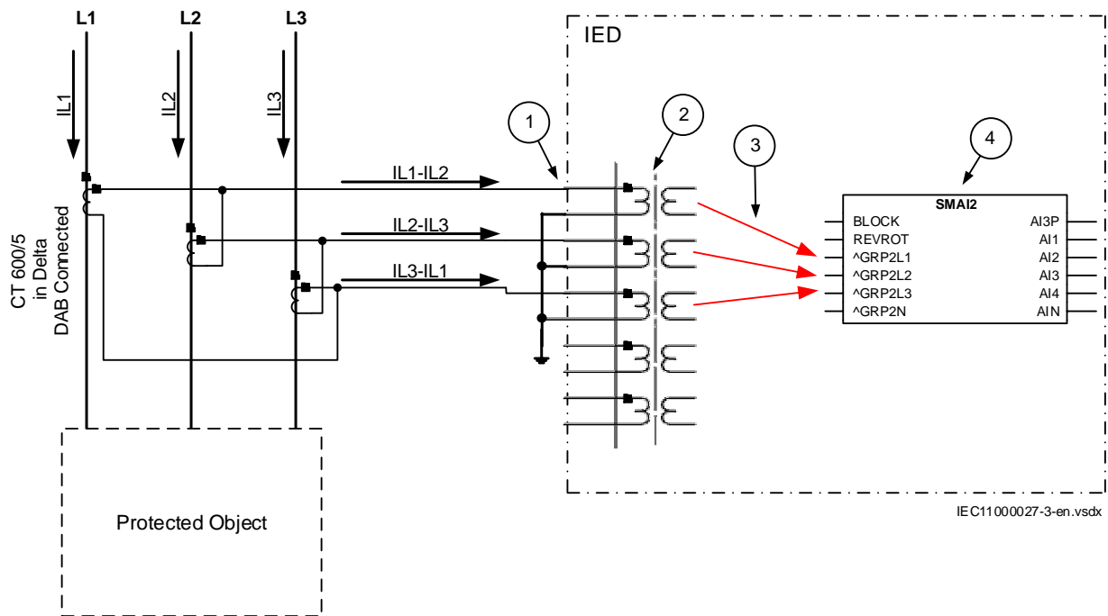
Figure 17: Delta DAB connected three-phase CT set
