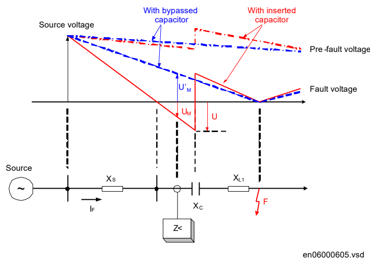
Figure 89: Voltage inversion on series compensated line
