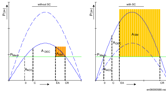
Figure 79: Equal area criterion and first swing stability without and with series compensation
