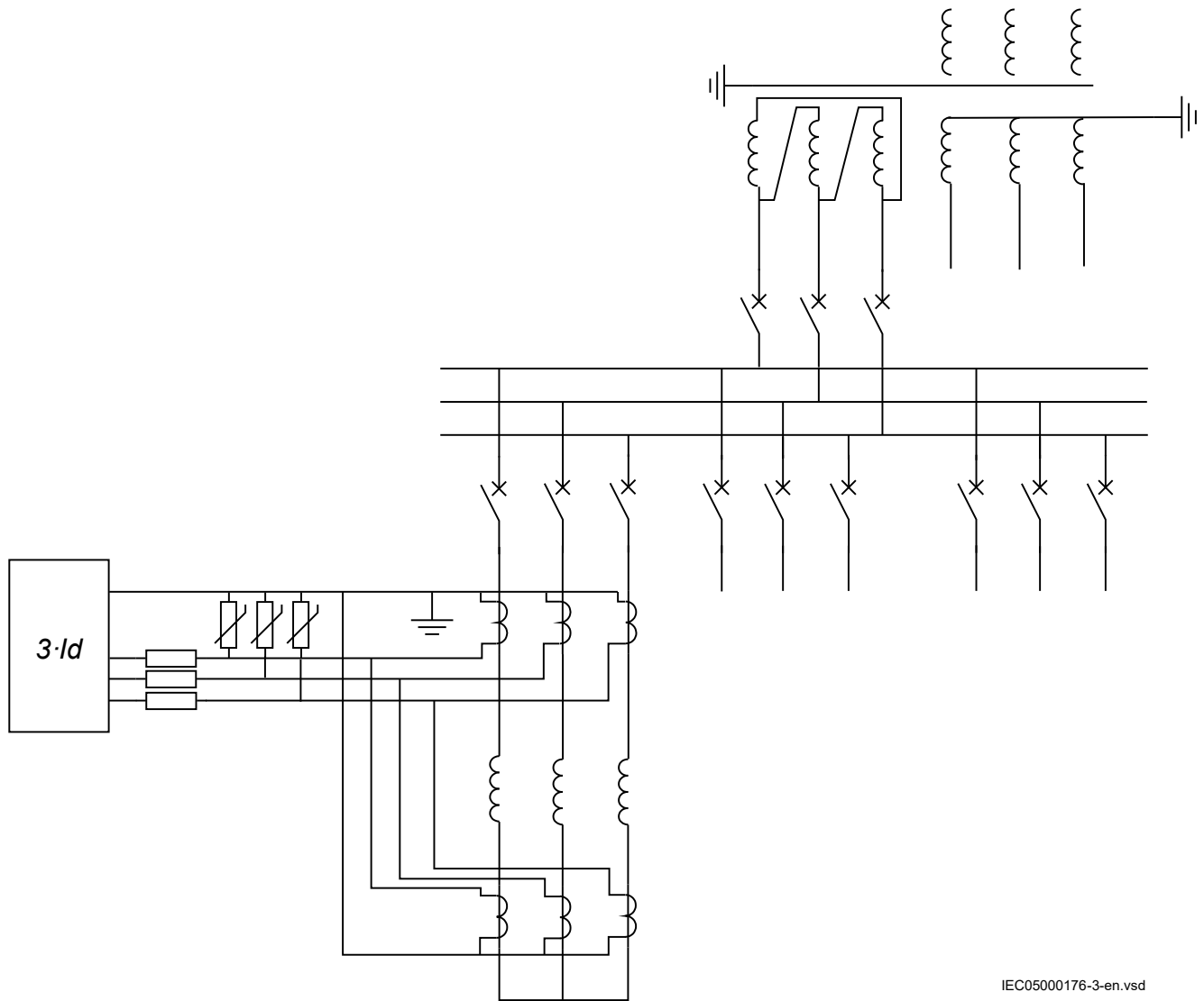
Figure 38: Application of the 1Ph High impedance differential protection HZPDIF function on a reactor
