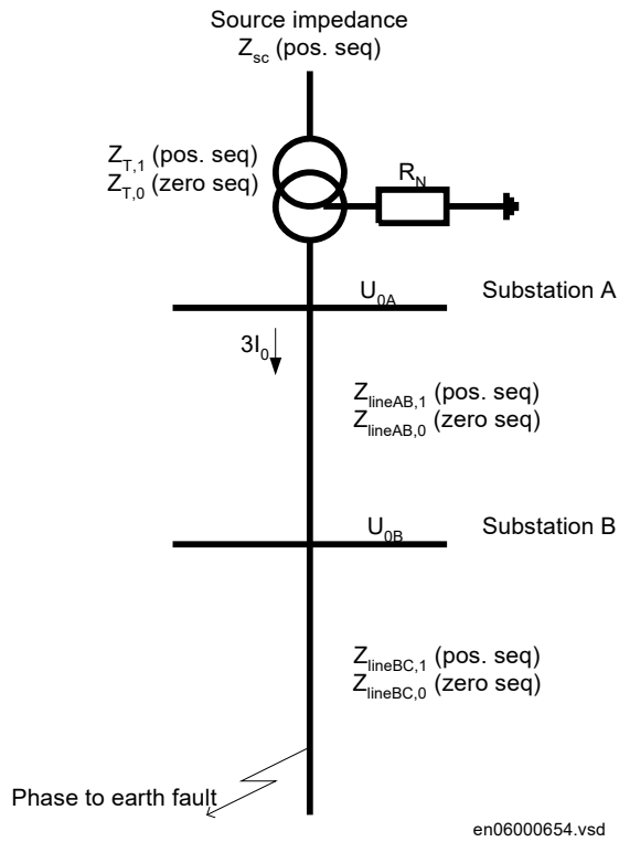
Figure 280: Equivalent of power system for calculation of setting
