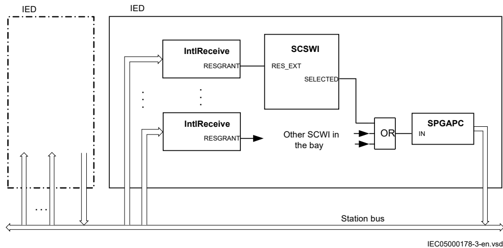
Figure 323: Application principle for an alternative reservation solution
