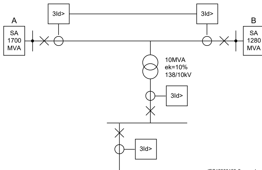
Figure 59: Setting example
