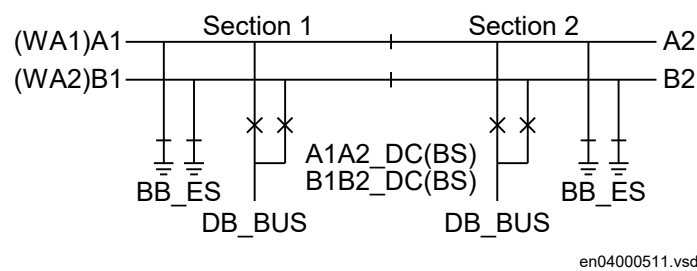
Figure 360: Busbars divided by bus-section disconnectors (circuit breakers)
