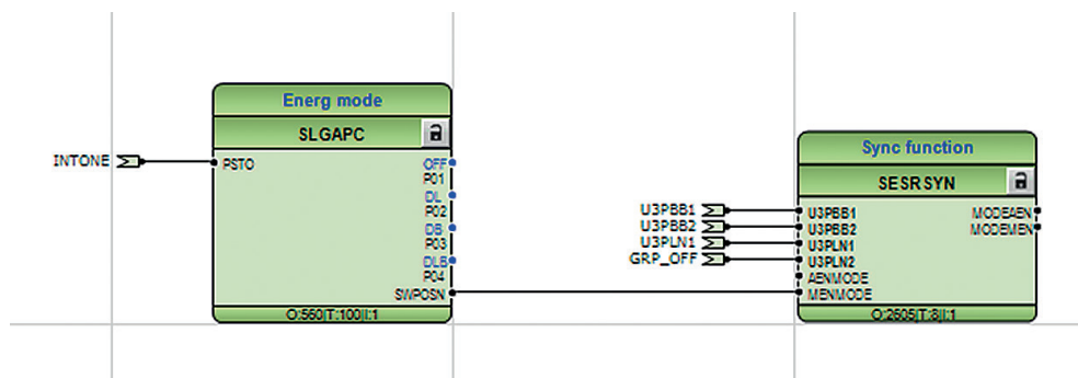
Figure 305: Selection of the energizing direction from a local HMI symbol through a selector switch function block.
