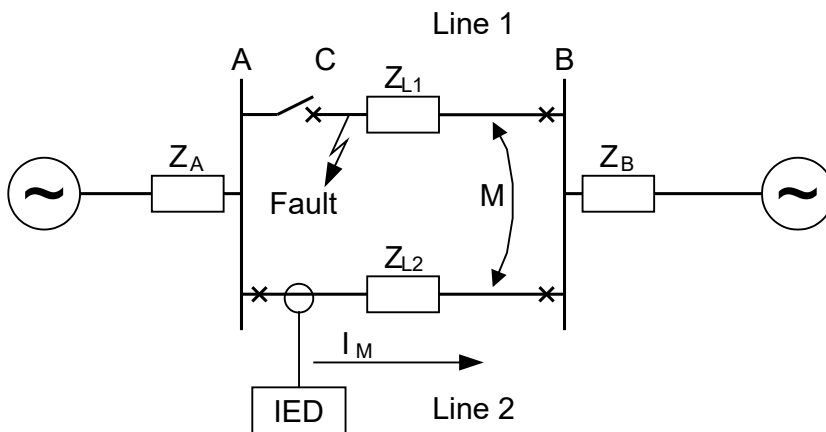
Figure 266: Two parallel lines. Influence from parallel line to the through fault current: I_M
