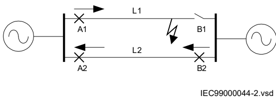
Figure 378: Current distribution for a fault close to B side when breaker at B1 is opened
