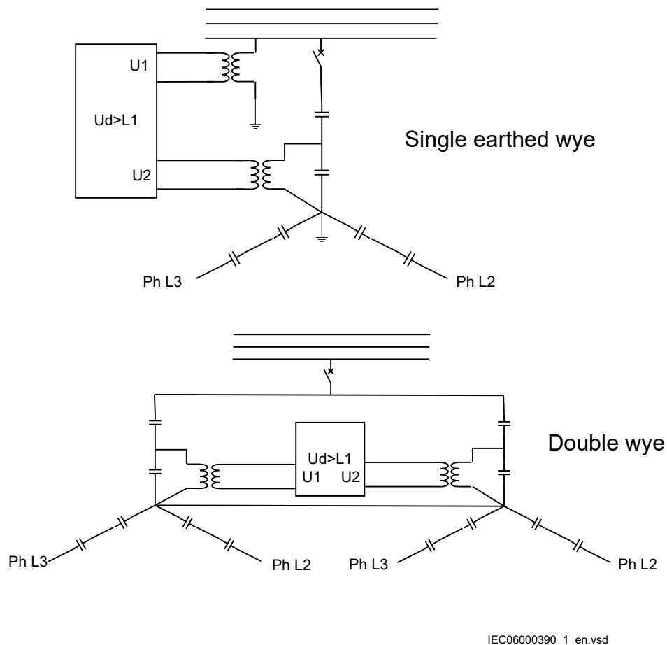
Figure 297: Connection of voltage differential protection VDCPTOV function to detect unbalance in capacitor banks (one phase only is shown)
