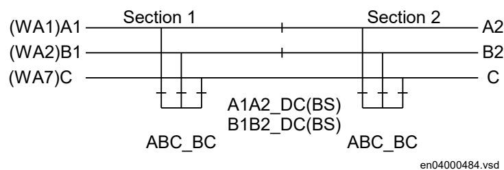
Figure 333: Busbars divided by bus-section disconnectors (circuit breakers)
