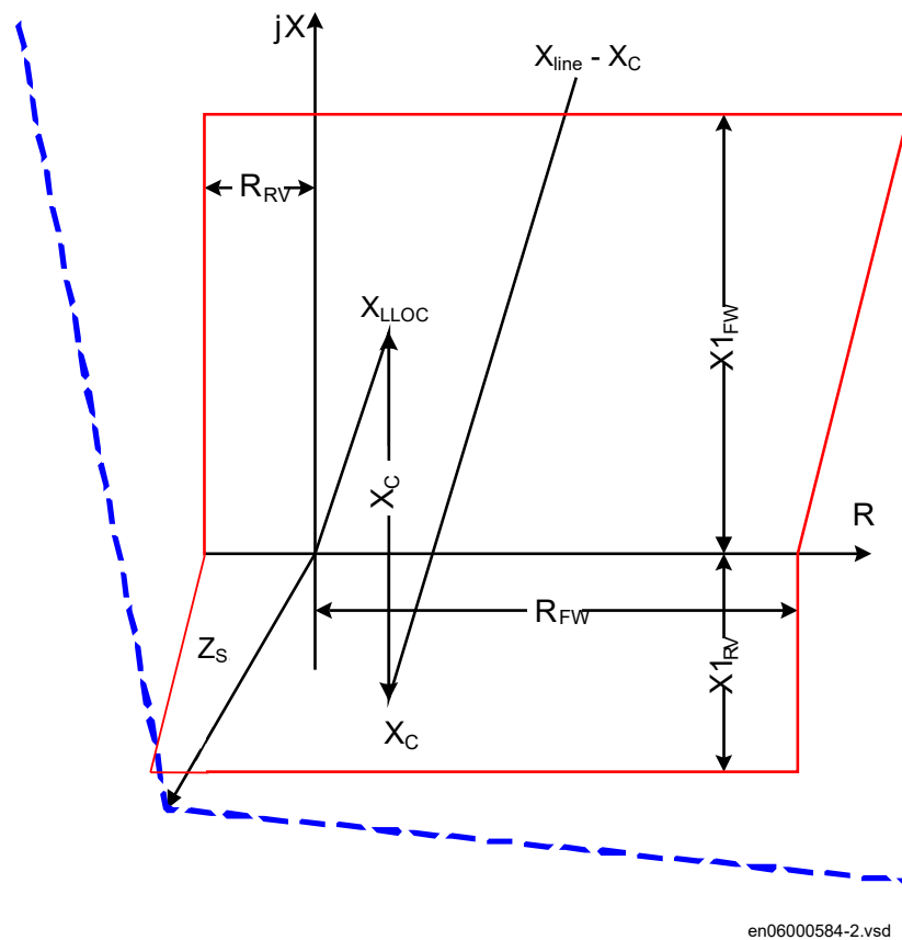
Figure 230: Measured impedance at voltage inversion
