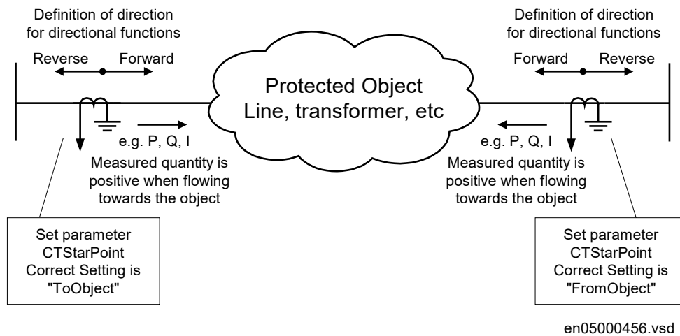
Figure 7: Internal convention of the directionality in the IED
