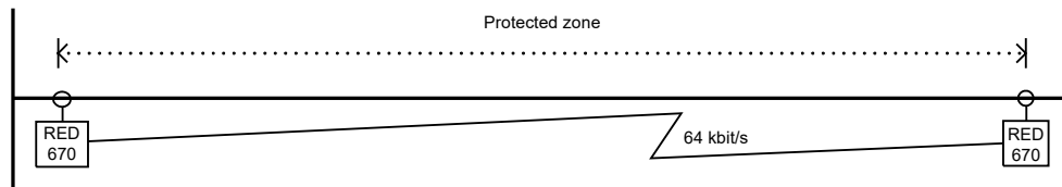
Figure 45: Two-terminal line
