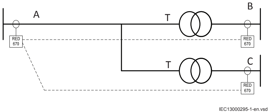
Figure 62: Master- Slave differential operation
