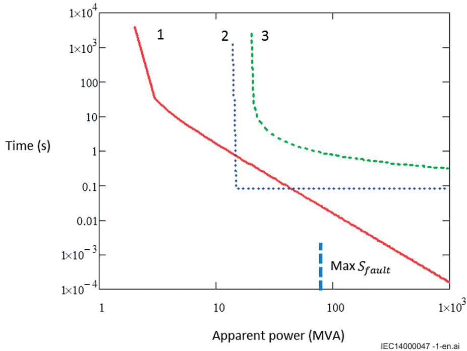
Figure 61: Selectivity chart
