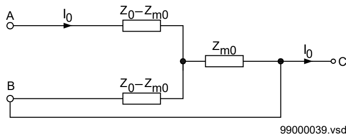
Figure 72: Equivalent zero-sequence impedance circuit for the double-circuit line that operates with one circuit disconnected and earthed at both ends
