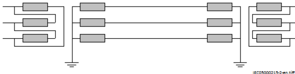
Figure 143: Solidly earthed network
