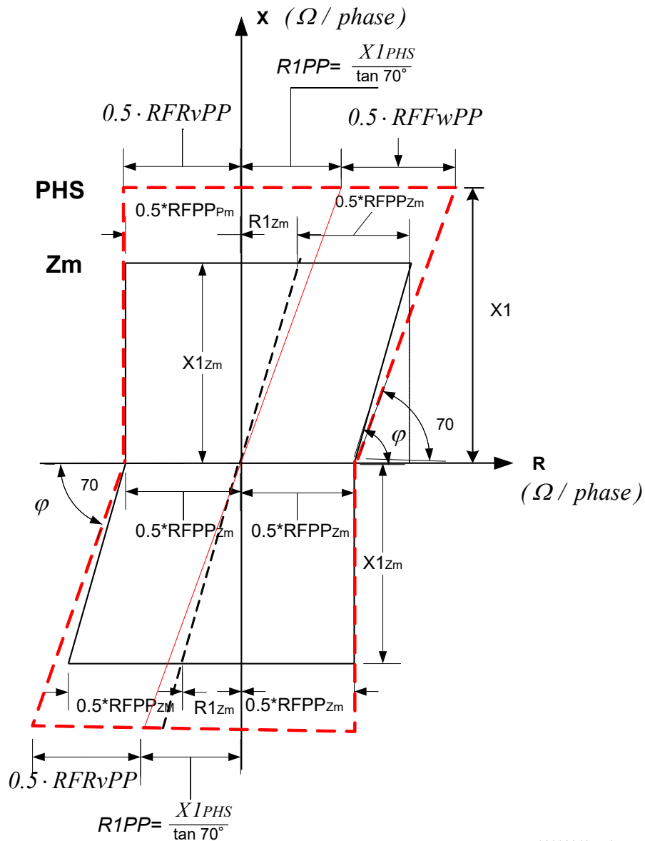
Figure 174: Relation between measuring zone and FRSPDIS characteristic for phase-to-phase fault for \phi_{line} > 70^\circ (setting parameters in italic)
