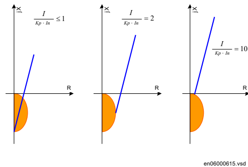
Figure 217: Equivalent impedance of MOV protected capacitor in dependence of protection factor K_p
