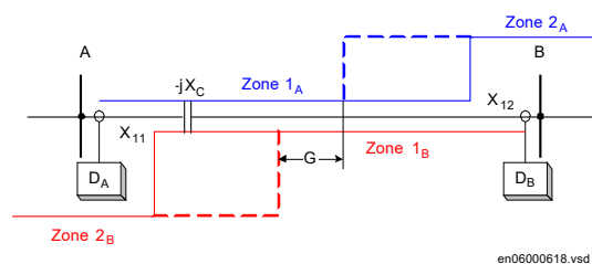
Figure 219: Underreaching (Zone 1) and overreaching (Zone 2) on series compensated line
