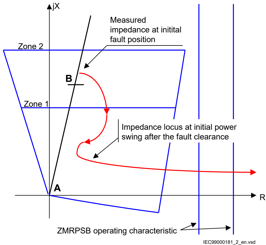
Figure 237: Impedance trajectory within the distance protection zones 1 and 2 during and after the fault on line B – D
