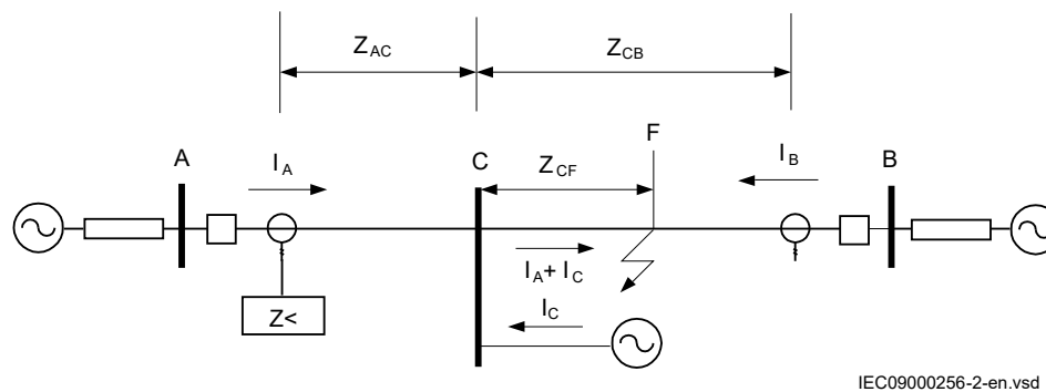
Figure 129: Setting of overreaching zone
