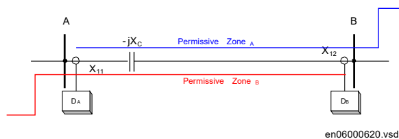
Figure 103: Permissive overreach distance protection scheme
