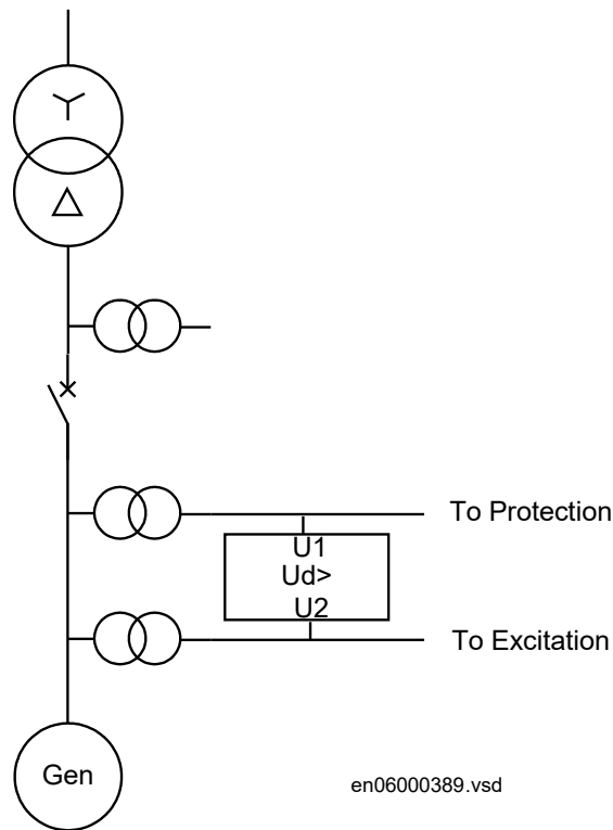
Figure 298: Supervision of fuses on generator circuit voltage transformers
