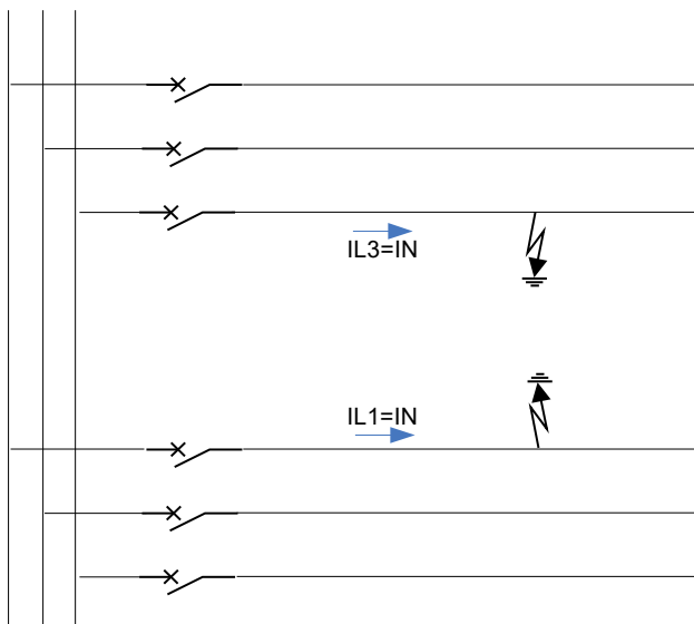
Figure 254: The currents in the phases at a double earth fault
