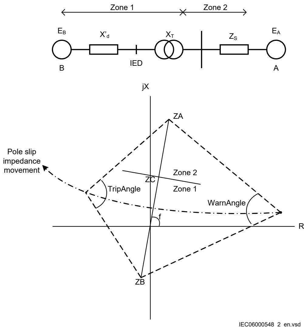
Figure 242: Settings for the Pole slip detection function
