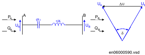
Figure 81: Transmission line with series capacitor
