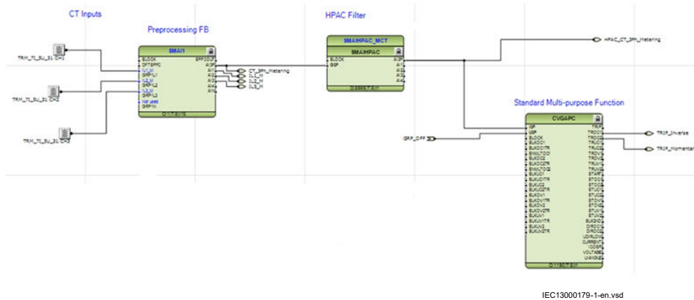
Figure 300: Required ACT configuration
