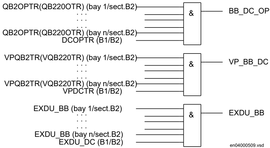
Figure 358: Signals from any bays in section B2 to a busbar earthing switch in the same section
