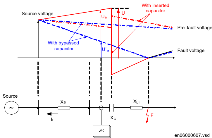
Figure 91: Current inversion on series compensated line
