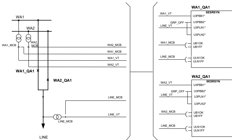
Figure 309: Connections of the SESRSYN function block in a double breaker arrangement
