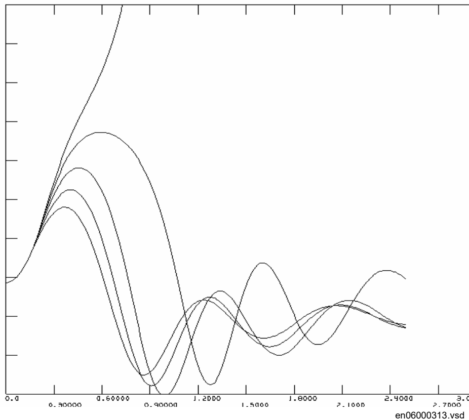
Figure 240: Relative generator phase angle at a fault and pole slip relative to the external power system
