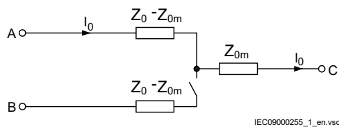
Figure 127: Equivalent zero-sequence impedance circuit for a double-circuit line with one circuit disconnected and not earthed
