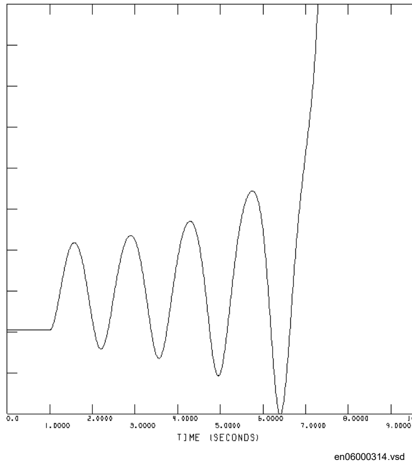
Figure 241: Undamped oscillations causing pole slip
