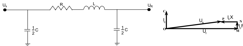
Figure 383: Vector diagram for local end and remote end voltage at no power transfer conditions
