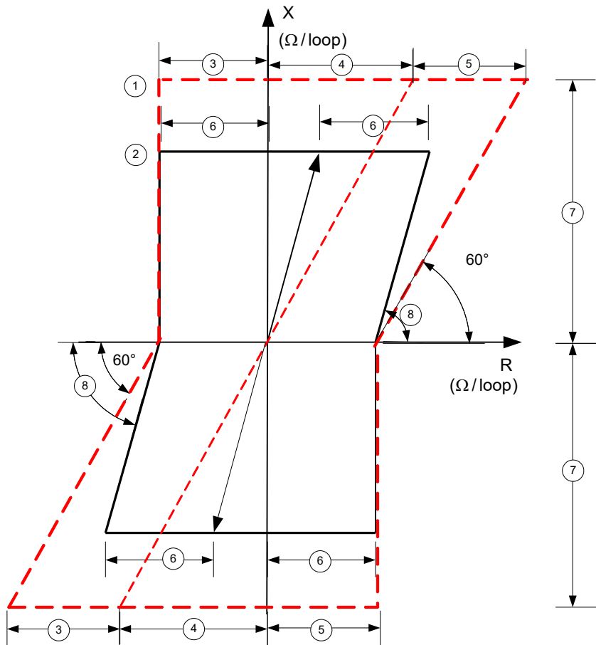
Figure 176: Relation between distance protection phase selection (FDPSDIS) and impedance zone (ZMQPDIS) for phase-to-earth fault \phi_{loop} > 60^\circ (setting parameters in italic)
