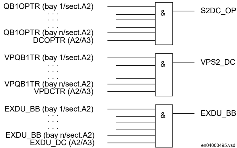
Figure 344: Signals from any bays in section A2 to a bus-section disconnecter
