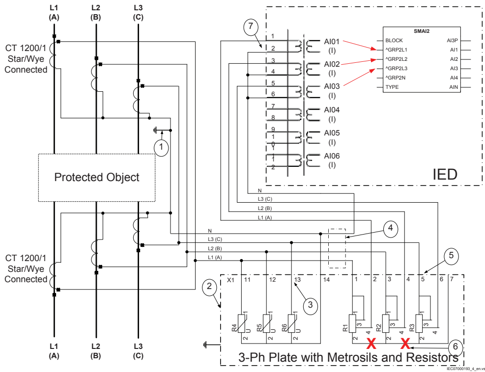
Figure 35: CT connections for high impedance differential protection
