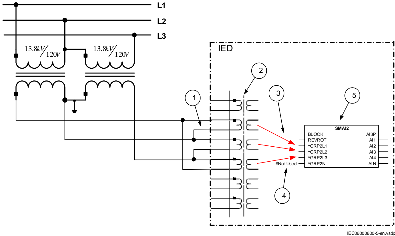
Figure 22: A Two phase-to-phase connected VT
