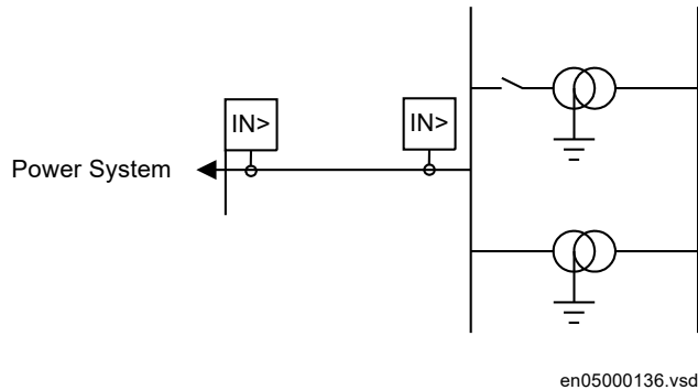
Figure 269: Application for parallel transformer inrush current logic
