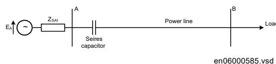
Figure 205: A simple radial power system
