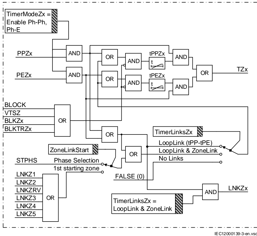
Figure 193: Logic for linking of timers
