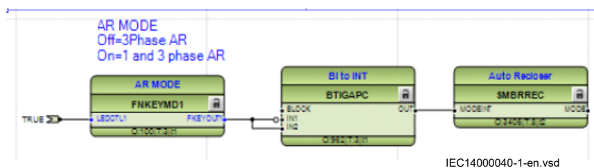
Figure 312: Selection of the auto-reclose mode from a hardware functional key in front of the IED
