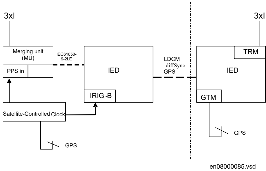
Figure 423: Time synchronization of merging unit and IED
