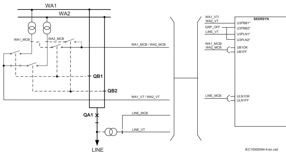
Figure 307: Connection of SESRSYN function block in a single breaker, double busbar arrangement with external voltage selection
