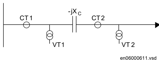
Figure 95: Possible positions of instrument transformers relative to line end series capacitor
