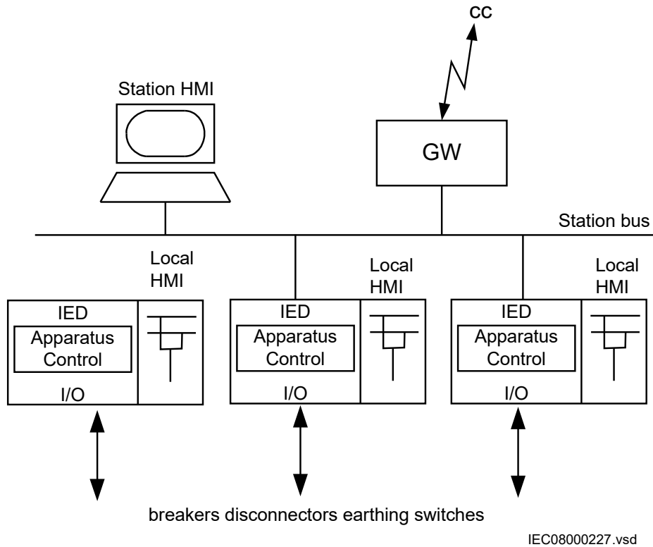
Figure 318: Overview of the apparatus control functions
