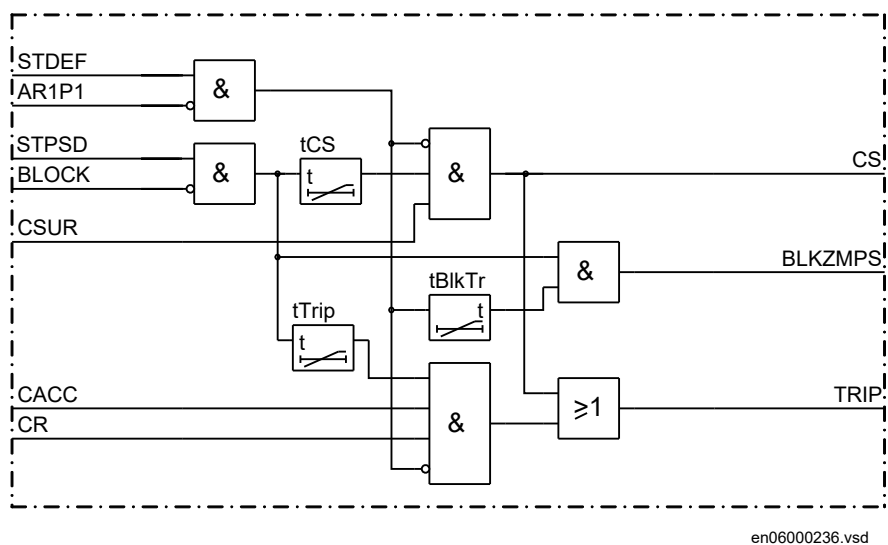
Figure 238: Simplified logic diagram - power swing communication and tripping logic
