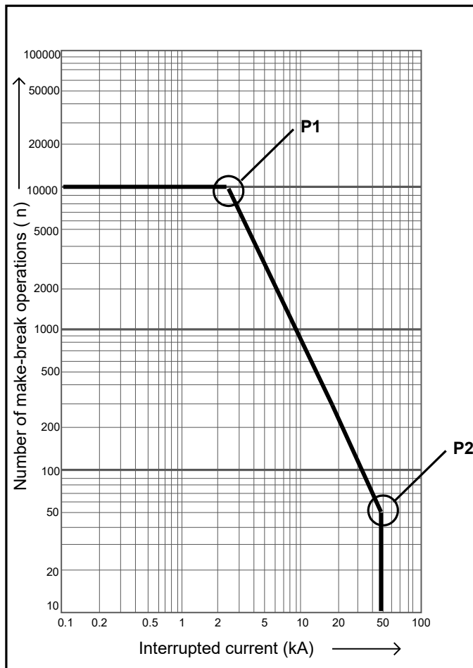
Figure 395: An example for estimating the remaining life of a circuit breaker
