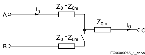
Figure 203: Equivalent zero-sequence impedance circuit for a double-circuit line with one circuit disconnected and not earthed
