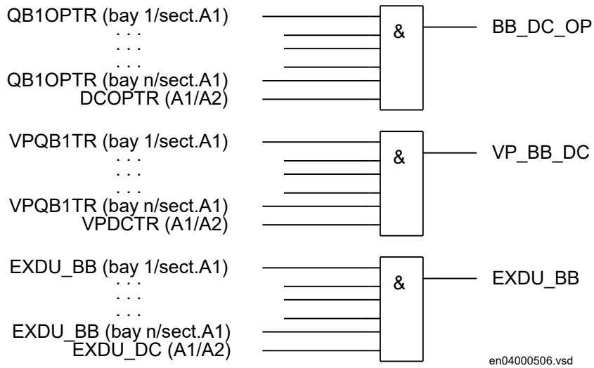
Figure 355: Signals from any bays in section A1 to a busbar earthing switch in the same section
