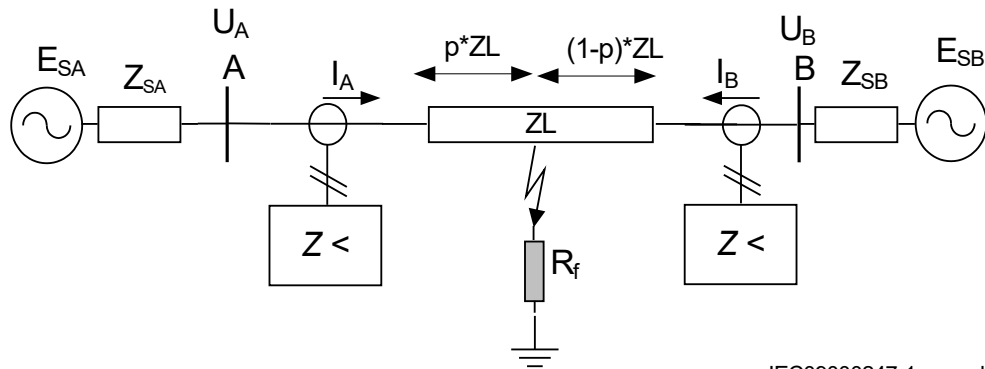
Figure 133: Influence of fault current infeed from remote end.
