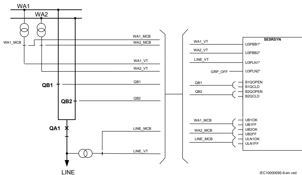
Figure 308: Connection of the SESRSYN function block in a single breaker, double busbar arrangement with internal voltage selection
