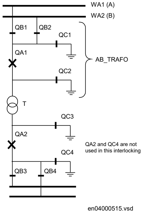
Figure 335: Switchyard layout AB_TRAFO
