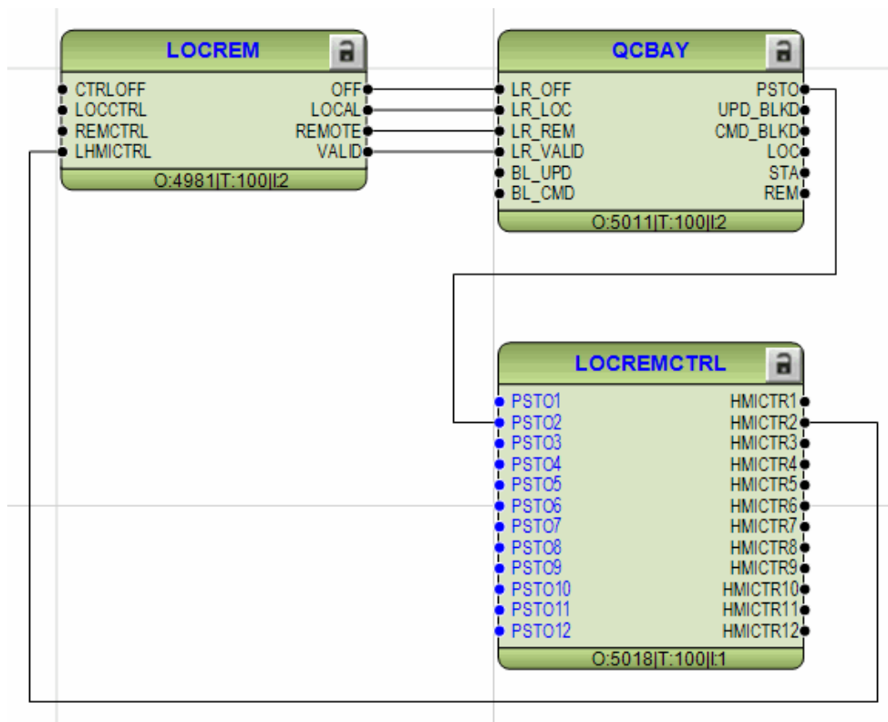
Figure 320: APC - Local remote function block
