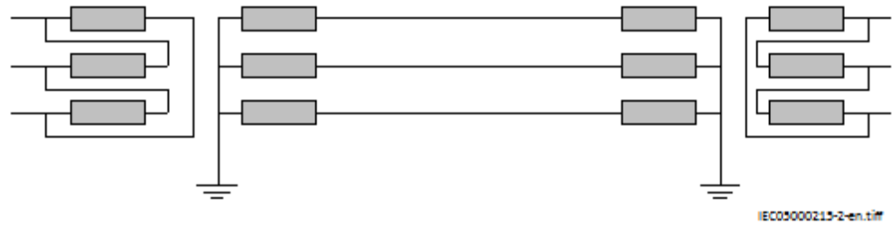
Figure 65: Solidly earthed network
