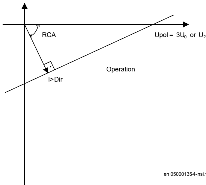
Figure 268: Relay characteristic angle given in degree
