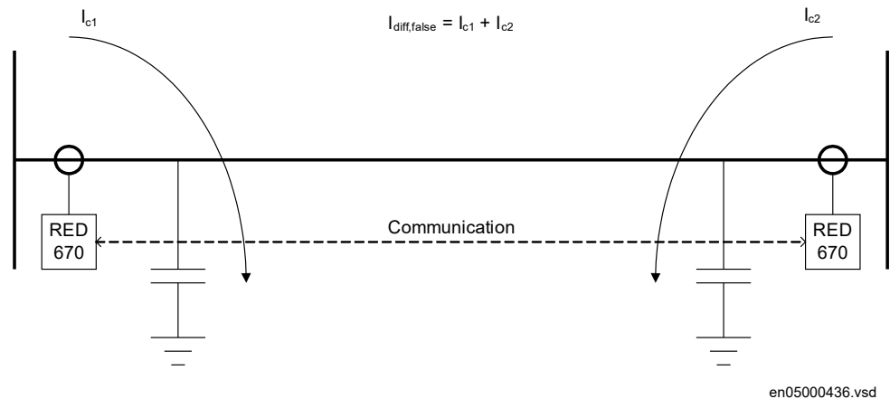
Figure 43: Charging currents
