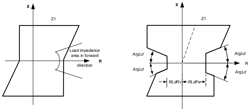
Figure 182: Load encroachment phenomena and shaped load encroachment characteristic
