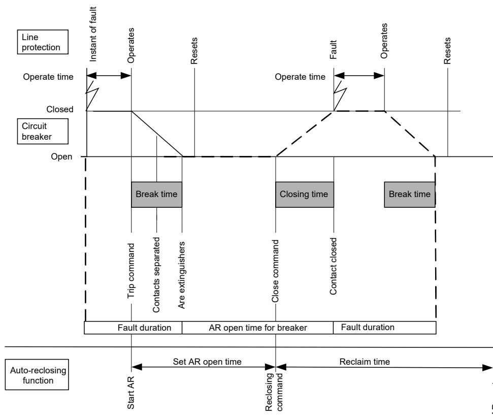
Figure 311: Single-shot automatic reclosing at a permanent fault
