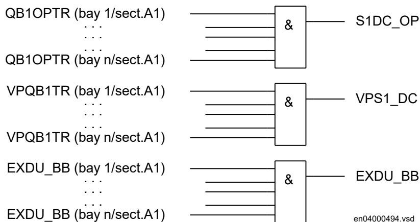
Figure 343: Signals from any bays in section A1 to a bus-section disconnecter
