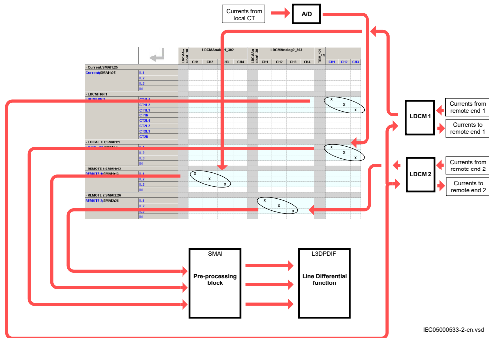
Figure 47: Typical configuration of analog signals for a three-terminal line
