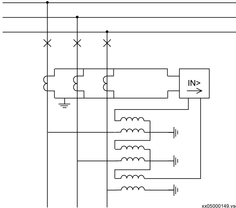
Figure 270: Connection of polarizing voltage from an open delta
