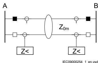
Figure 164: Parallel line is out of service and not earthed.
