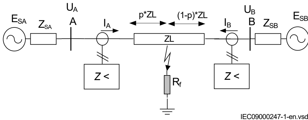
Figure 119: Influence of fault current infeed from remote line end
