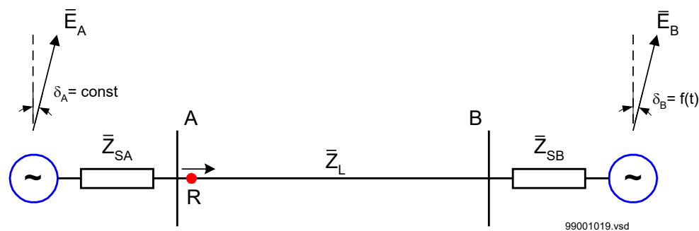
Figure 234: Protected power line as part of a two-machine system
