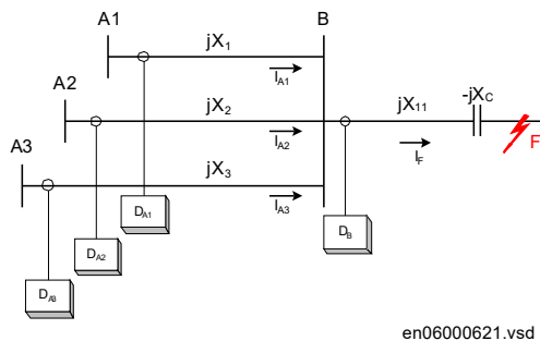
Figure 104: Distance IED on adjacent power lines are influenced by the negative impedance
