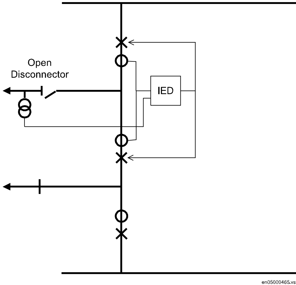
Figure 285: Typical connection for STBPTOC in 1½-breaker arrangement.
