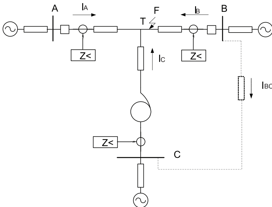
Figure 189: Example of tapped line with Auto transformer
