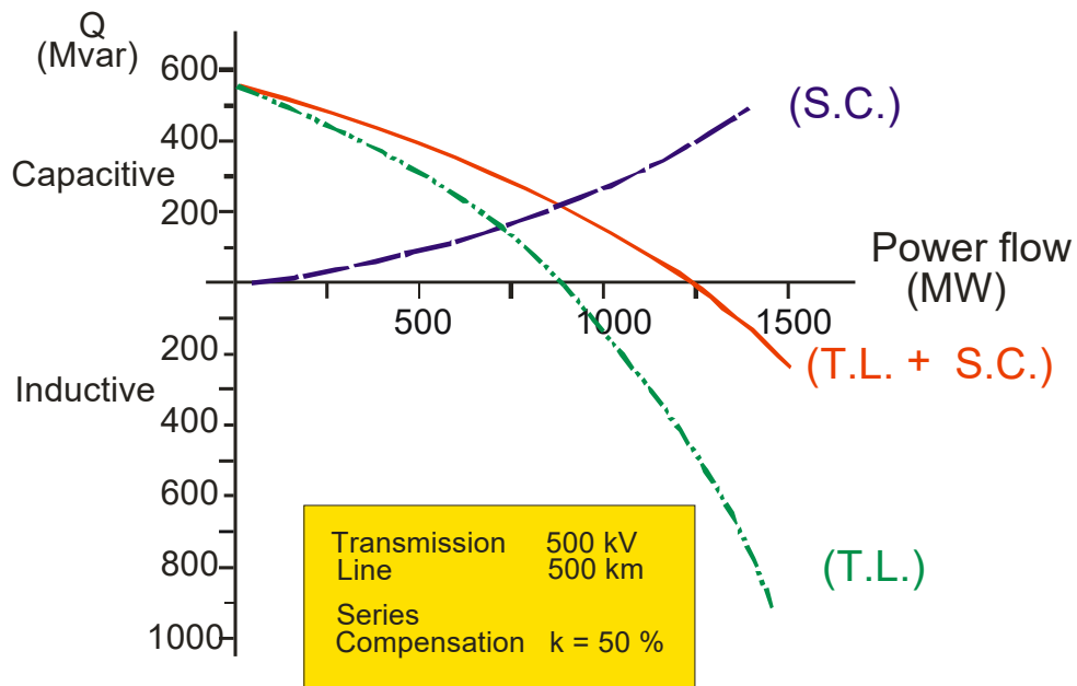
Figure 80: Self-regulating effect of reactive power balance
