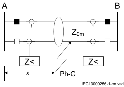
Figure 140: Parallel line is out of service and not earthed
