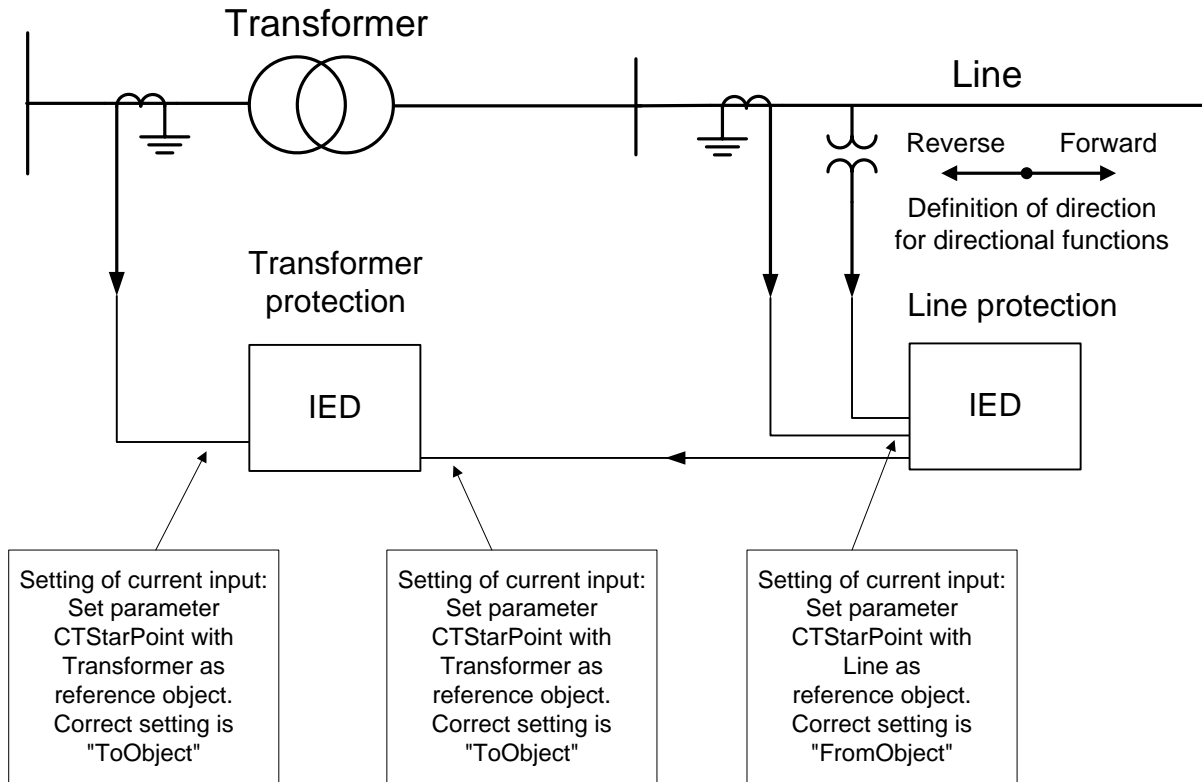
Figure 9: Example how to set CTStarPoint parameters in the IED
