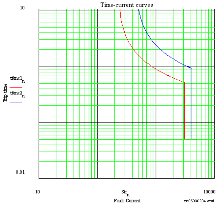
Figure 262: Fault time with maintained selectivity
