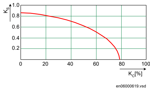
Figure 220: Underreaching safety factor K_S in dependence on system compensation degree K_C
