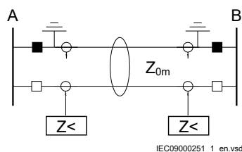
Figure 162: The parallel line is out of service and earthed.
