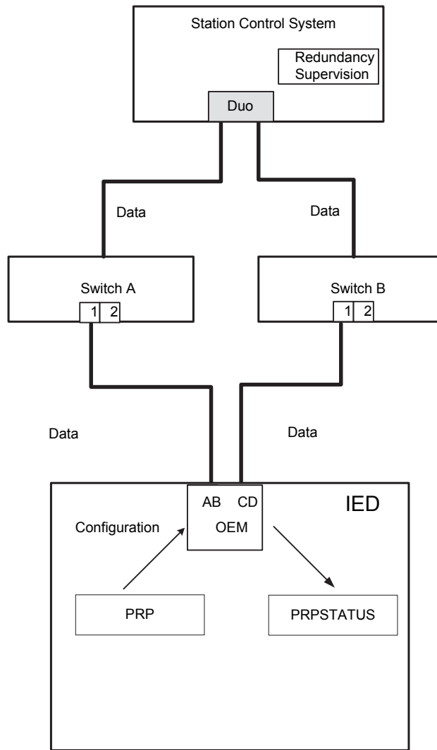
Figure 403: Redundant station bus
