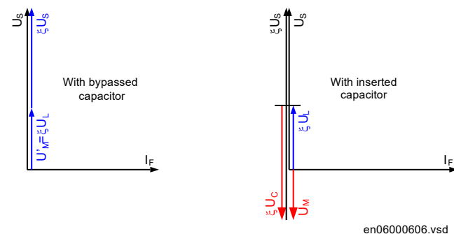
Figure 90: Phasor diagrams of currents and voltages for the bypassed and inserted series capacitor during voltage inversion
