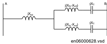
Figure 108: Zero sequence equivalent circuit of a series compensated double circuit line with one circuit disconnected and earthed at both IEDs
