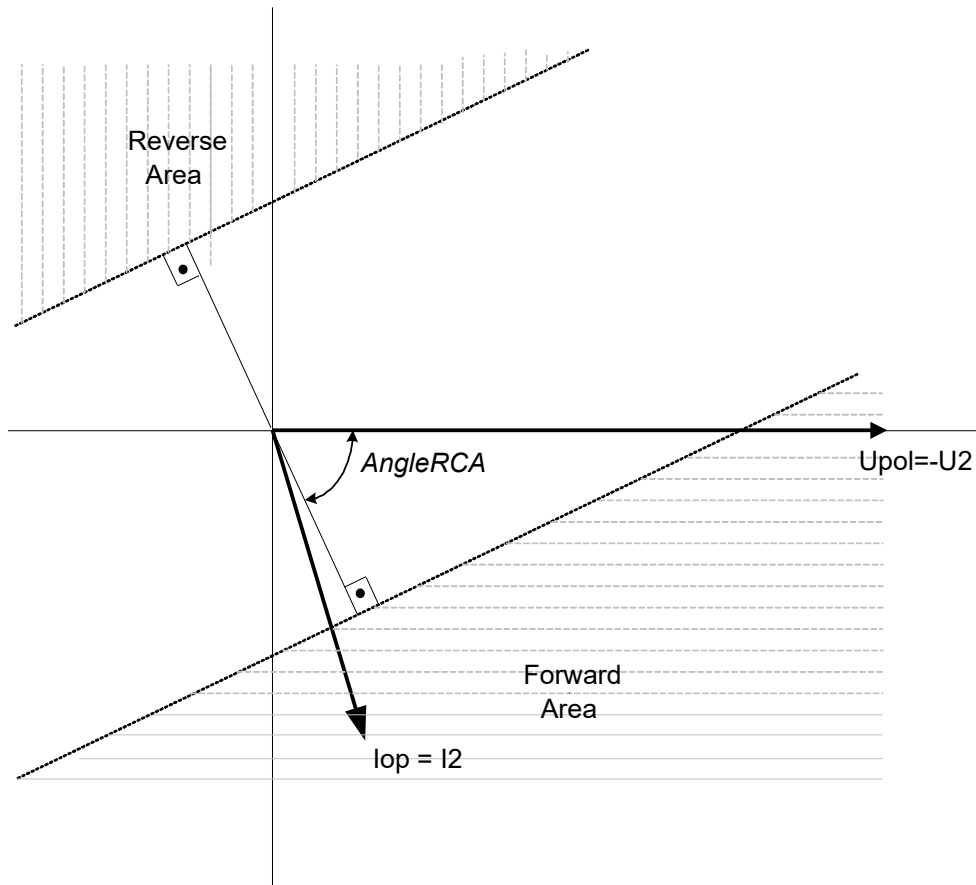
Figure 278: Relay characteristic angle given in degree
