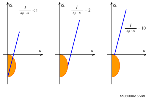
Figure 99: Equivalent impedance of MOV protected capacitor in dependence of protection factor K_p
