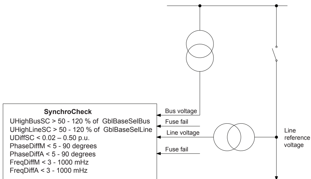
Figure 303: Principle for the synchrocheck function
