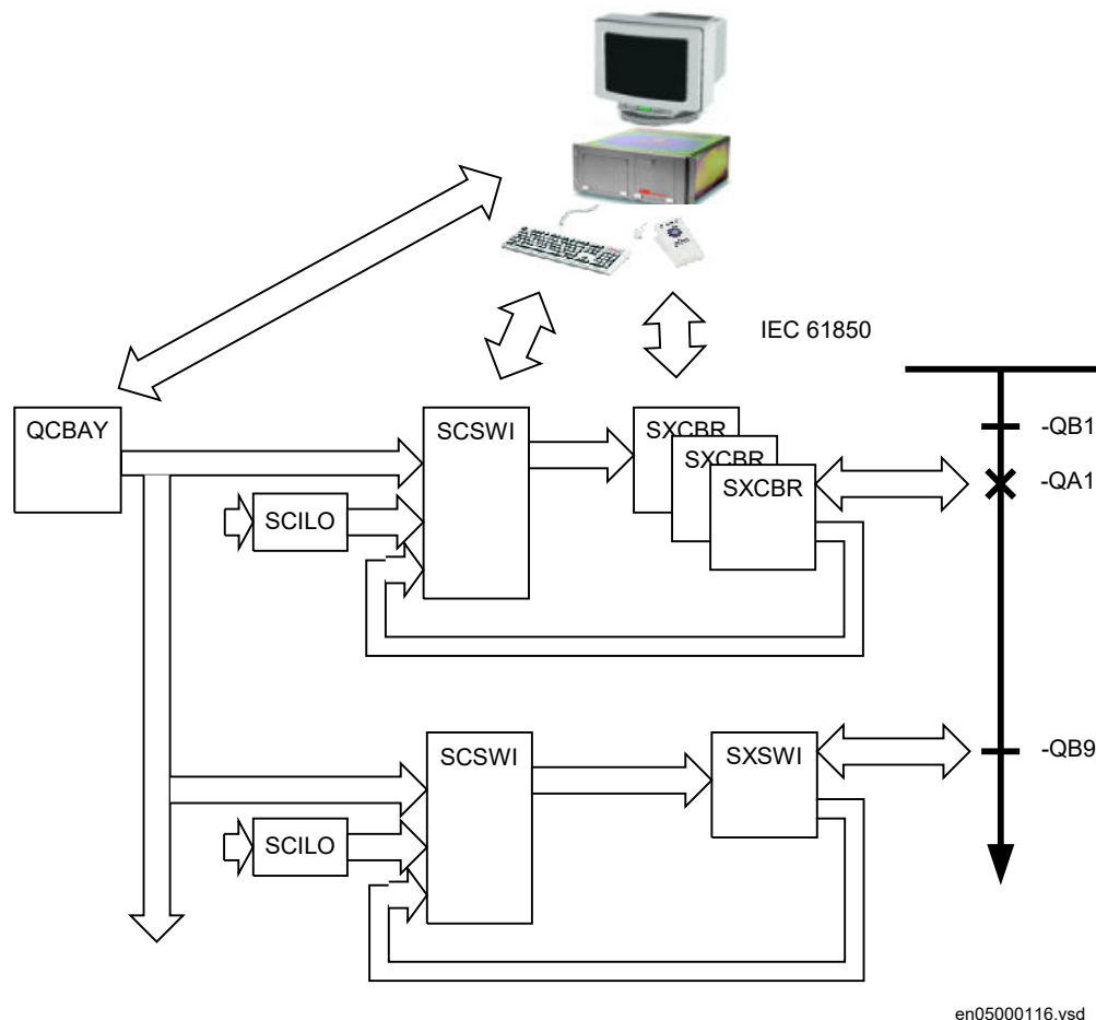
Figure 319: Signal flow between apparatus control function blocks
