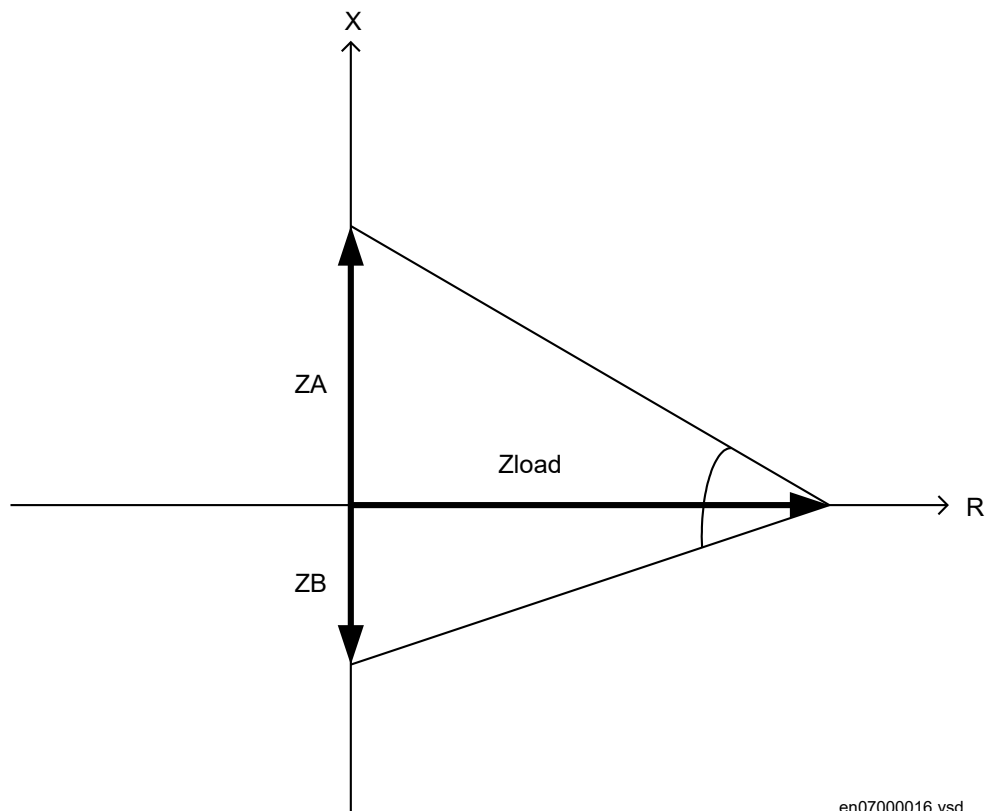
Figure 248: Simplified figure to derive StartAngle
