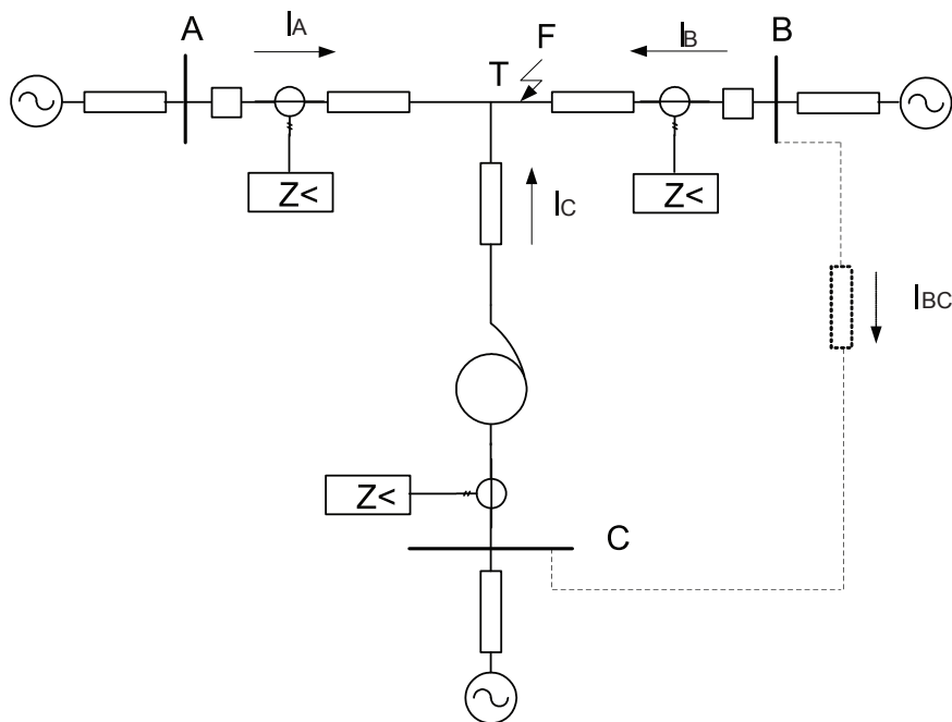
Figure 128: Example of tapped line with Auto transformer
