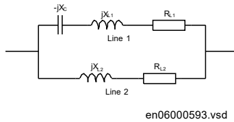
Figure 83: Two parallel lines with series capacitor for optimized load sharing and loss reduction
