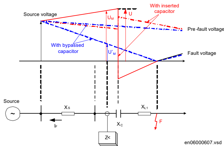
Figure 211: Current inversion on series compensated line
