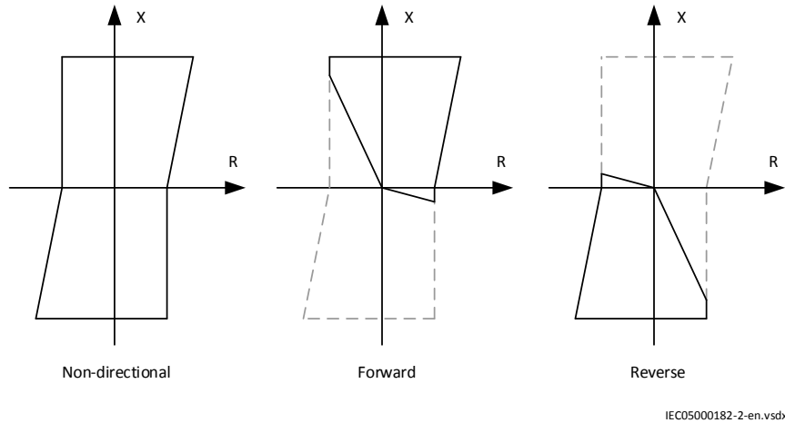
Figure 232: Directional operating modes of the distance measuring zones 3 to 5 tPPZx , tPEZx , TimerModeZx , ZoneLinkStart and TimerLinksZx
