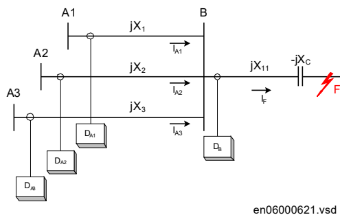
Figure 222: Distance IED on adjacent power lines are influenced by the negative impedance
