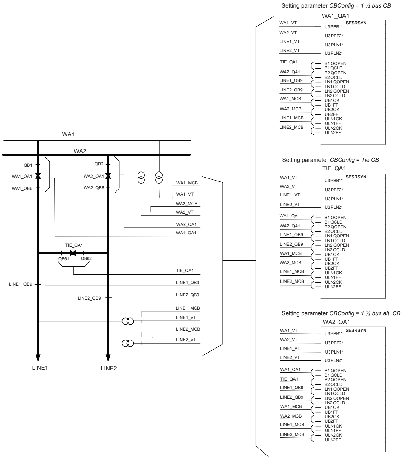
Figure 310: Connections of the SESRSYN function block in a 1 1/2 breaker arrangement with internal voltage selection
