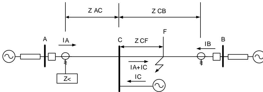
Figure 110: Setting of overreaching zone
