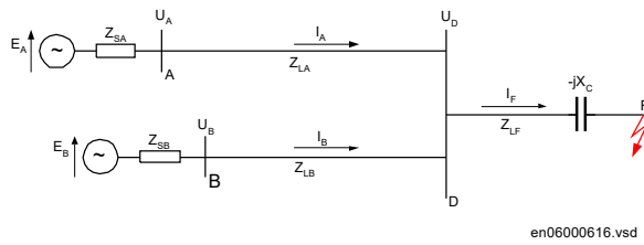
Figure 218: Voltage inversion in series compensated network due to fault current infeed
