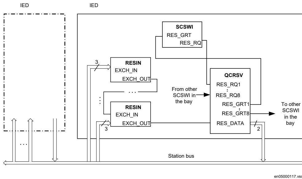
Figure 321: Application principles for reservation over the station bus
