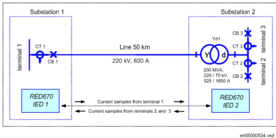
Figure 57: Line differential protection with power transformer in protected zone
