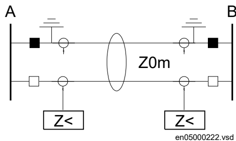
Figure 149: The parallel line is out of service and earthed.
