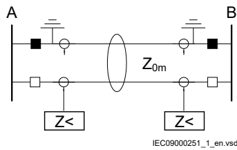
Figure 124: The parallel line is out of service and earthed
