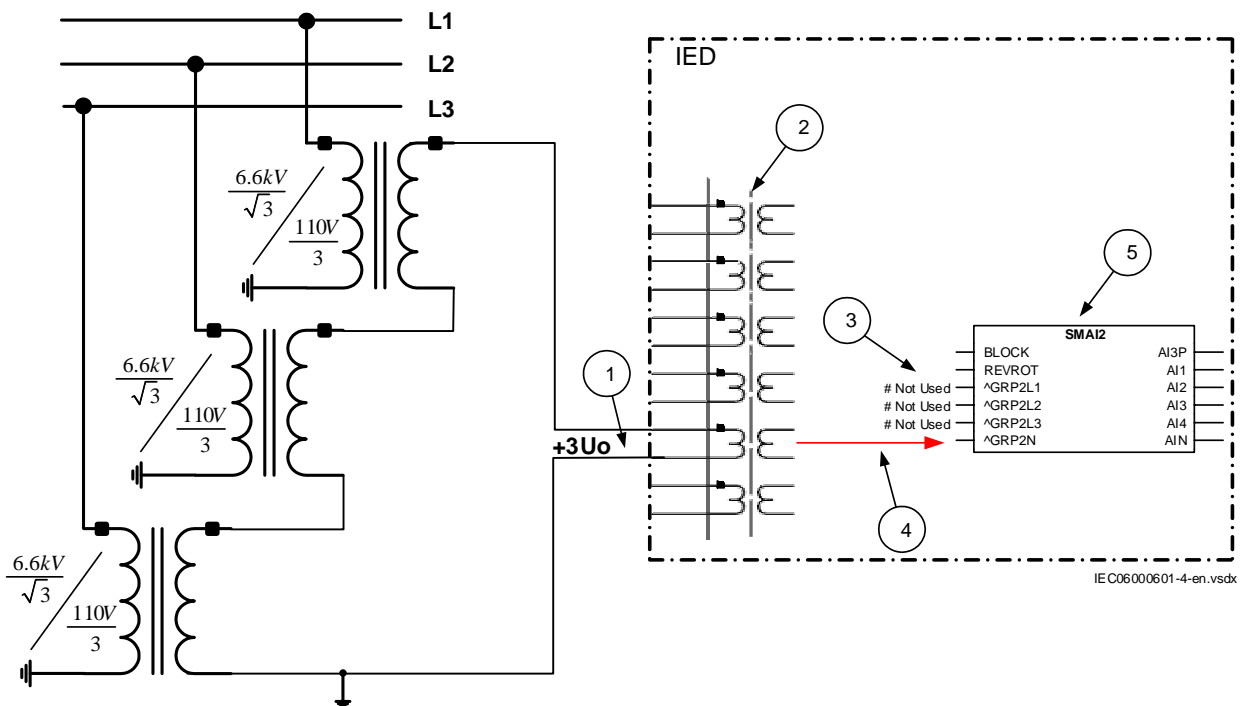
Figure 23: Open delta connected VT in high impedance earthed power system
