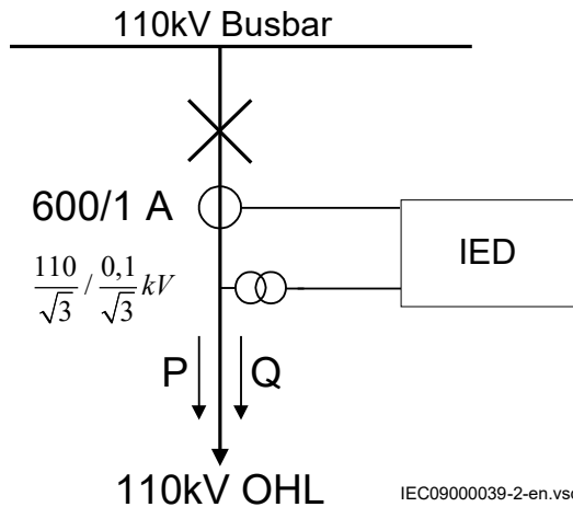
Figure 392: Single line diagram for 110kV OHL application
