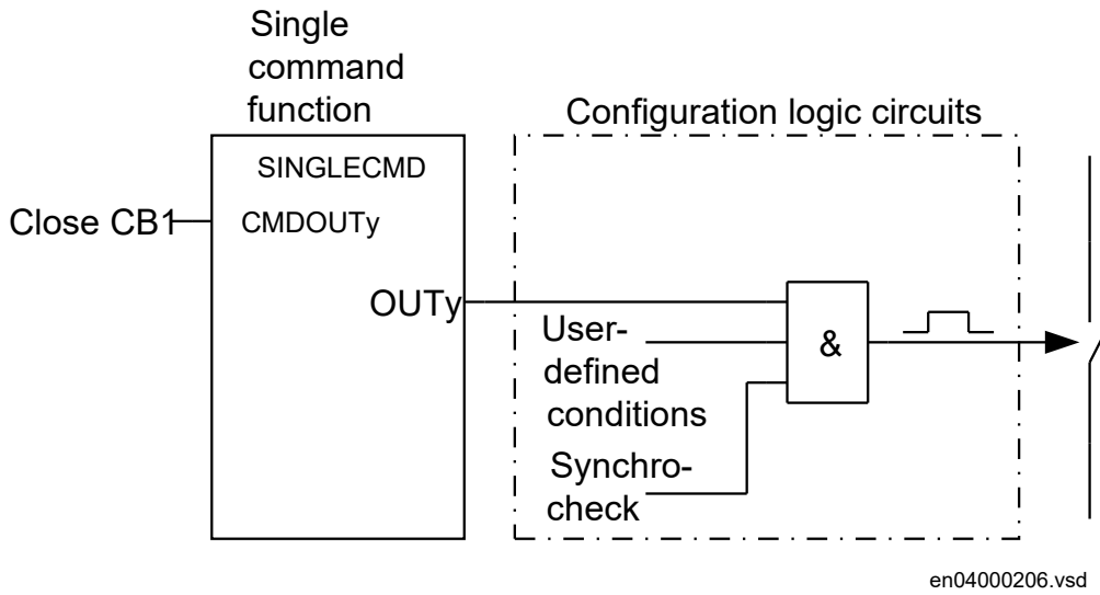
Figure 365: Application example showing a logic diagram for control of a circuit breaker via configuration logic circuits
