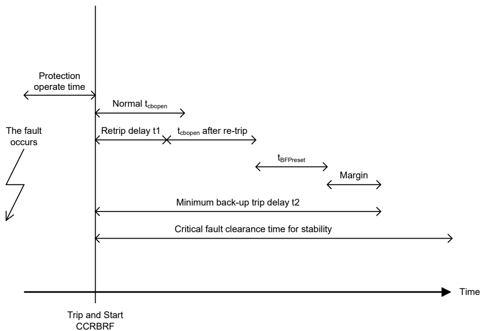
Figure 284: Time sequence
