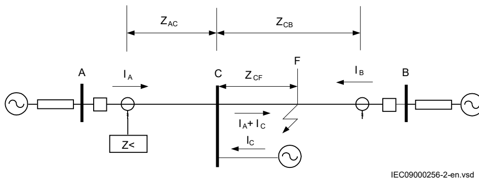
Figure 167: Setting of overreaching zone
