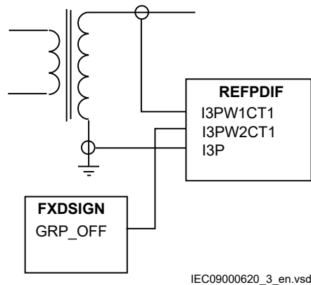
Figure 390: REFPDIF function inputs for normal transformer application
