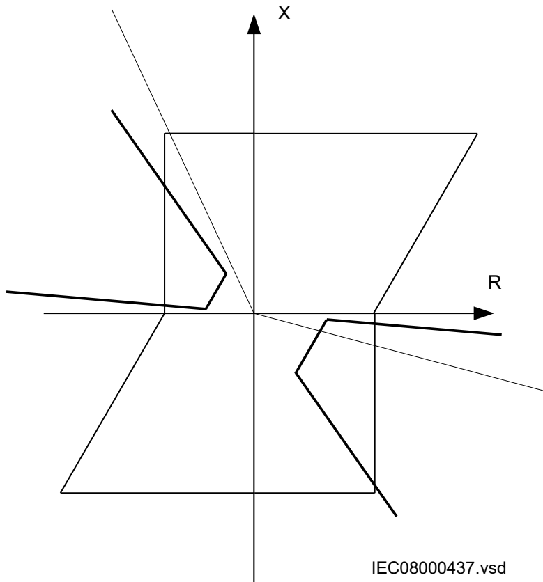
Figure 172: Rotation of load characteristic for a fault between two phases
