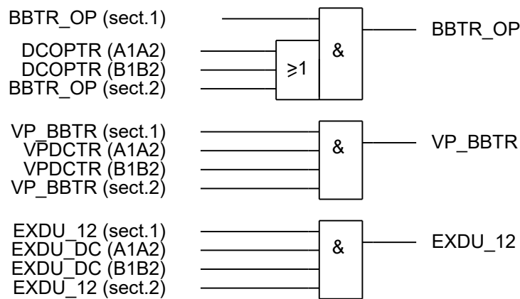
Figure 332: Signals to a bus-coupler bay in section 1 from any bays in each section
