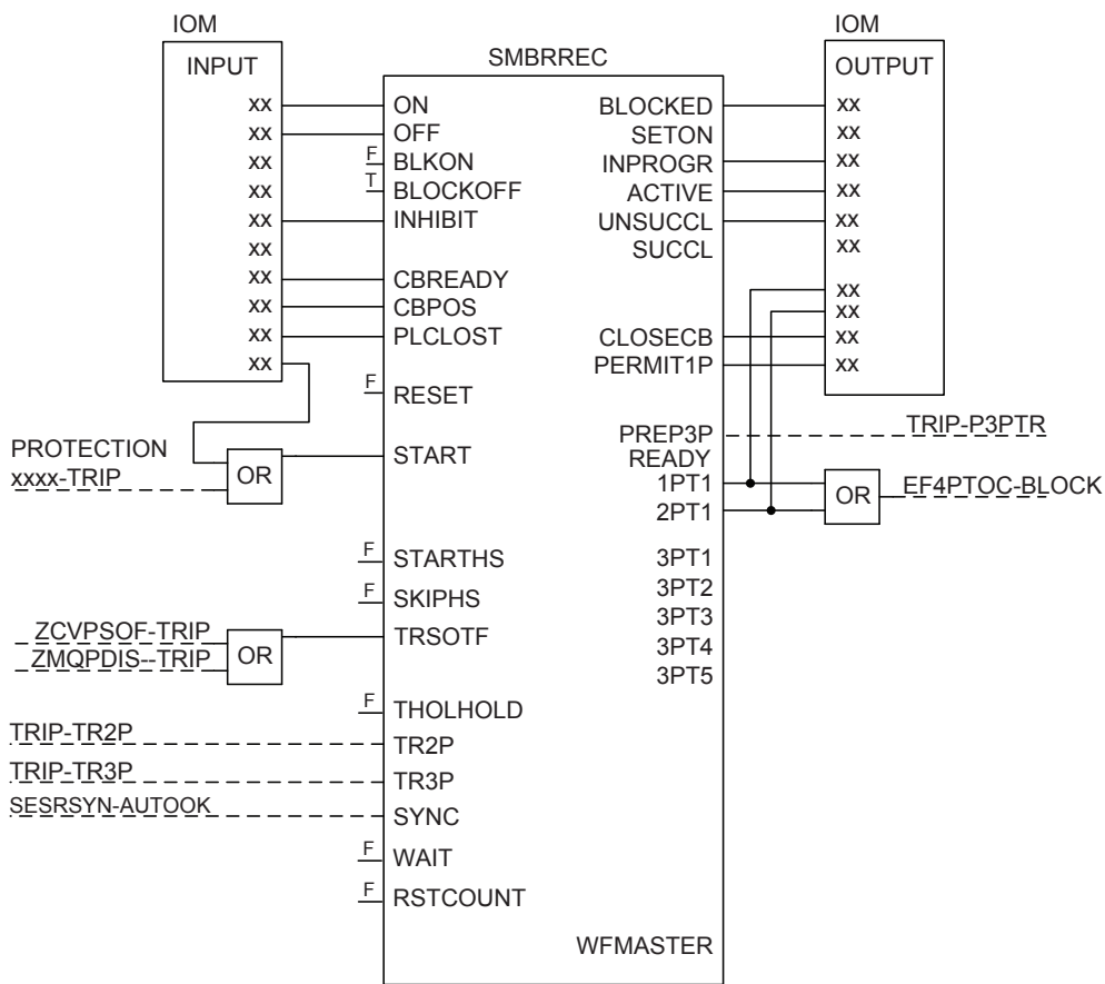
Figure 316: Example of I/O-signal connections in a single-phase, two-phase or three-phase reclosing function
