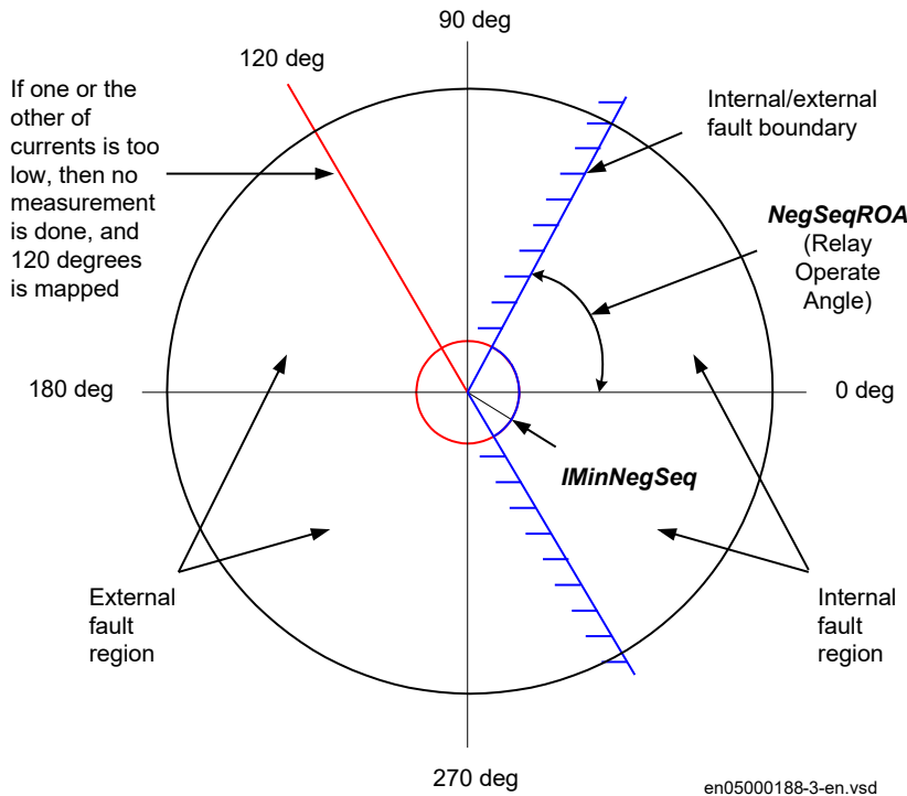
Figure 51: Negative sequence current function Relay Operate Angle (ROA)
