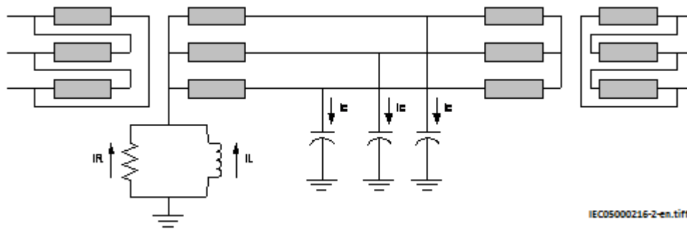
Figure 132: High impedance earthing network
