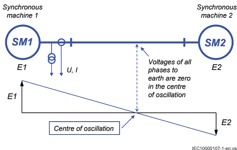
Figure 249: The centre of electromechanical oscillation
