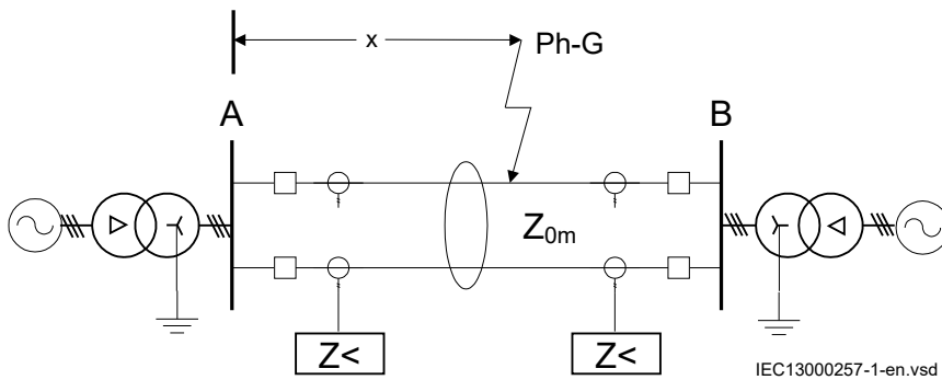
Figure 141: Class 1, parallel line in service
