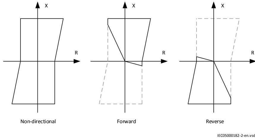
Figure 192: Directional operating modes of the distance measuring zones 3 to 5 tPPZx, tPEZx, TimerModeZx, ZoneLinkStart and TimerLinksZx
