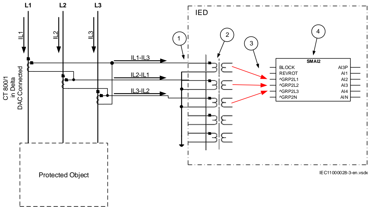
Figure 18: Delta DAC connected three-phase CT set
