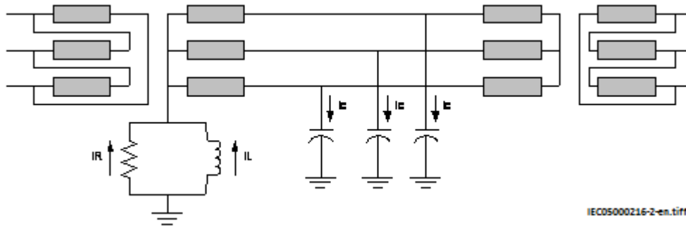
Figure 144: High impedance earthing network
