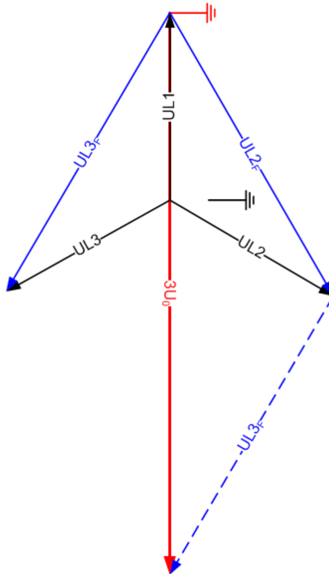
Figure 293: Earth fault in Non-effectively earthed systems
