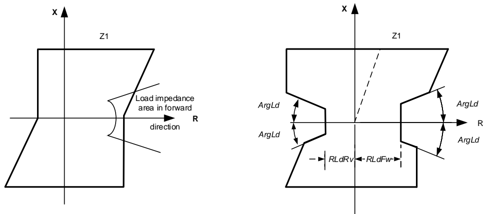
Figure 196: Load encroachment phenomena and shaped load encroachment characteristic
