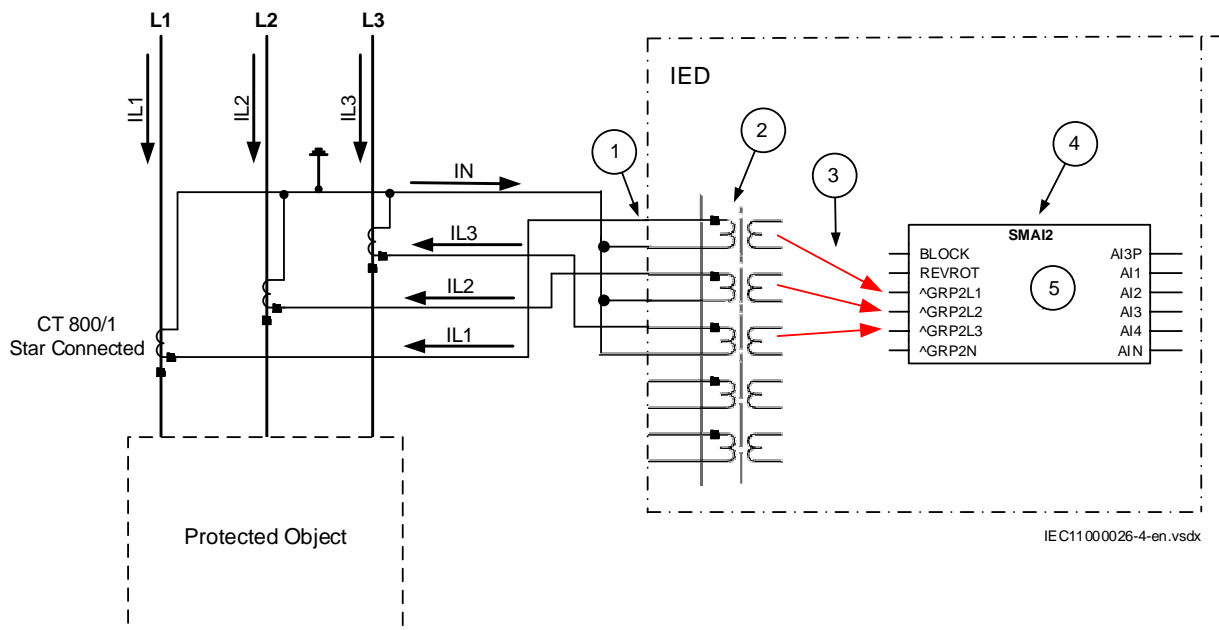
Figure 15: Star connected three-phase CT set with its star point away from the protected object
