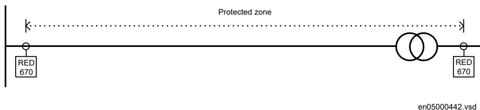
Figure 52: One two-winding transformer in the protected zone
