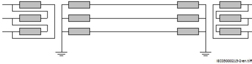
Figure 117: Solidly earthed network
