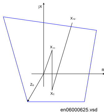
Figure 223: Cross-polarized quadrilateral characteristic
