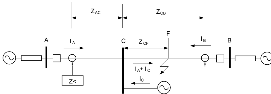
Figure 190: Setting of overreaching zone
