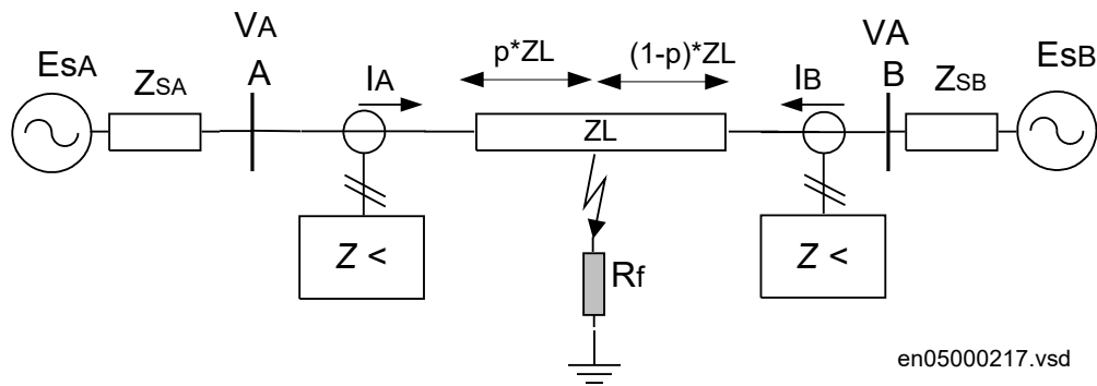
Figure 145: Influence of fault infeed from remote end.
