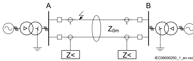
Figure 160: Class 1, parallel line in service.
