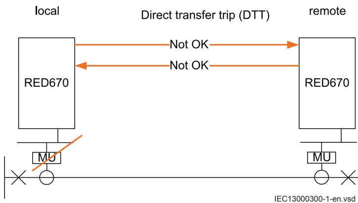
Figure 409: MU failed, 9-2 system
