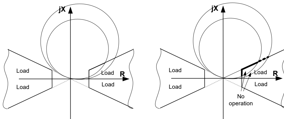
Figure 134: Load encroachment phenomena and shaped load encroachment characteristic
