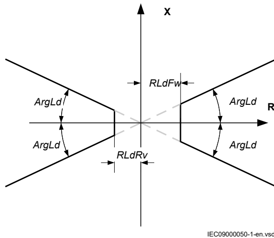
Figure 175: Load encroachment characteristic
