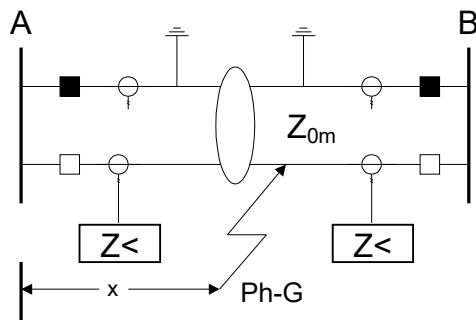
Figure 139: The parallel line is out of service and earthed
