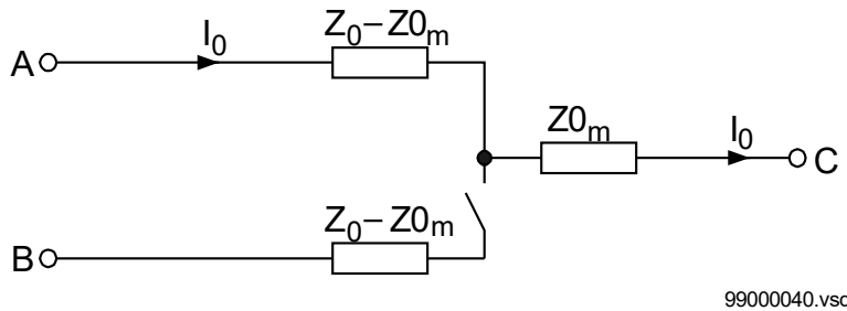
Figure 152: Equivalent zero-sequence impedance circuit for a double-circuit line with one circuit disconnected and not earthed.
