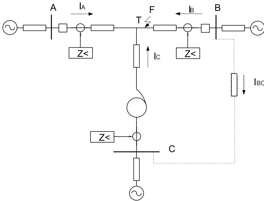
Figure 166: Example of tapped line with Auto transformer.
