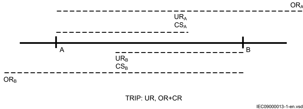
Figure 370: Principle of Permissive underreaching scheme
