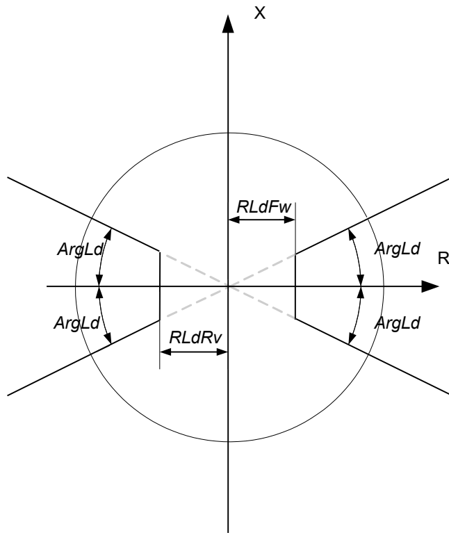
Figure 135: Load encroachment of Faulty phase identification with load encroachment for mho function FMPSPDIS characteristic
