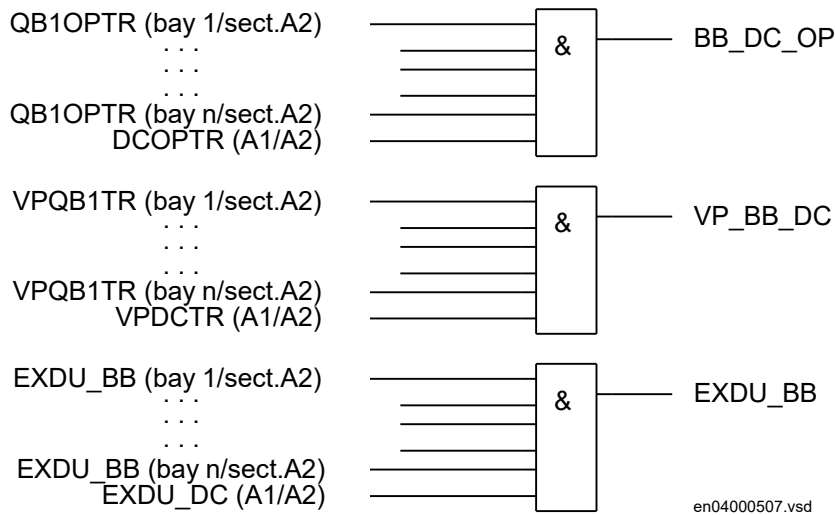
Figure 356: Signals from any bays in section A2 to a busbar earthing switch in the same section
