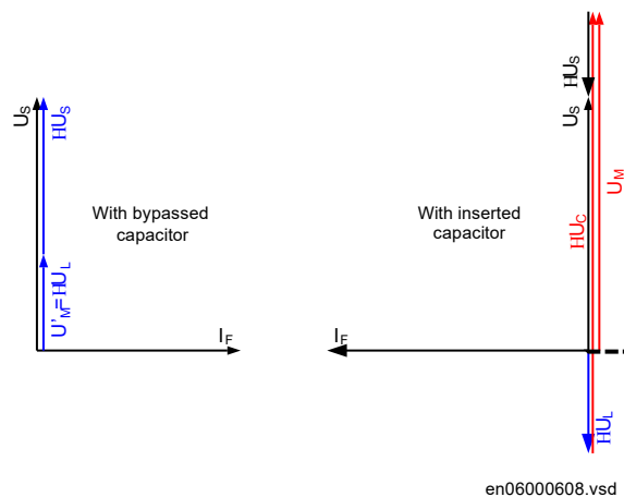
Figure 92: Phasor diagrams of currents and voltages for the bypassed and inserted series capacitor during current inversion
