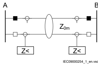
Figure 126: Parallel line is out of service and not earthed
