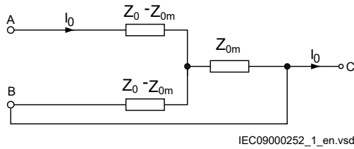
Figure 163: Equivalent zero sequence impedance circuit for the double-circuit line that operates with one circuit disconnected and earthed at both ends.
