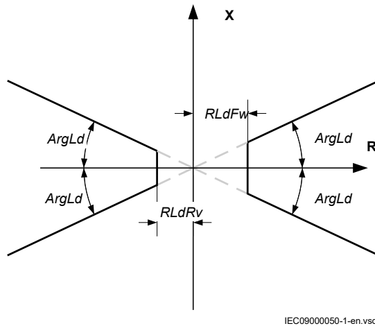
Figure 178: Load encroachment characteristic
