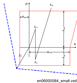
Figure 224: Quadrilateral characteristic with separate impedance and directional measurement
