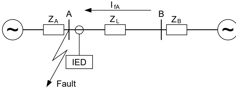
Figure 265: Through fault current from B to A: I_{fA}
