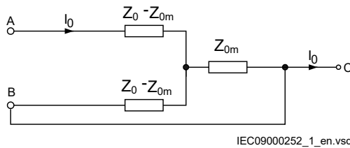
Figure 125: Equivalent zero sequence impedance circuit for the double-circuit line that operates with one circuit disconnected and earthed at both ends
