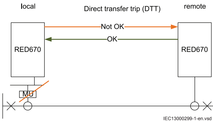
Figure 408: MU failed, mixed system
