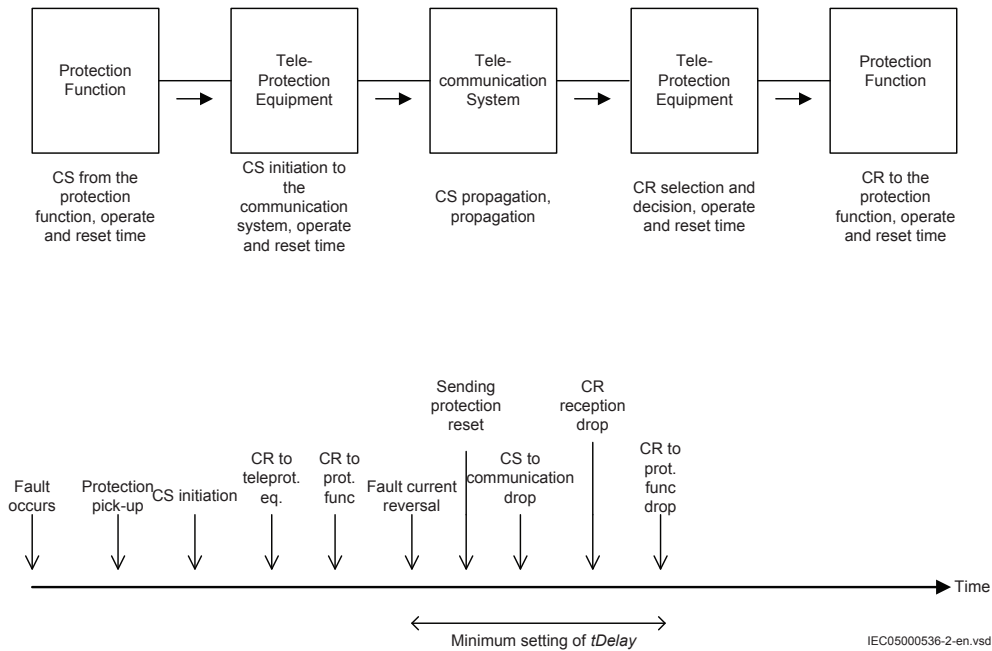
Figure 380: Time sequence of signaling at current reversal
