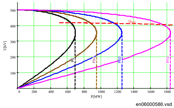
Figure 77: Voltage profile for a simple radial power line with 0, 30, 50 and 70% of compensation
