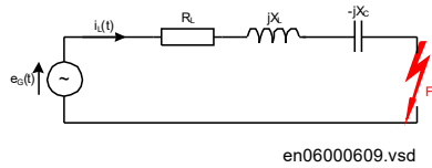
Figure 93: Simplified equivalent scheme of SC network during fault conditions
