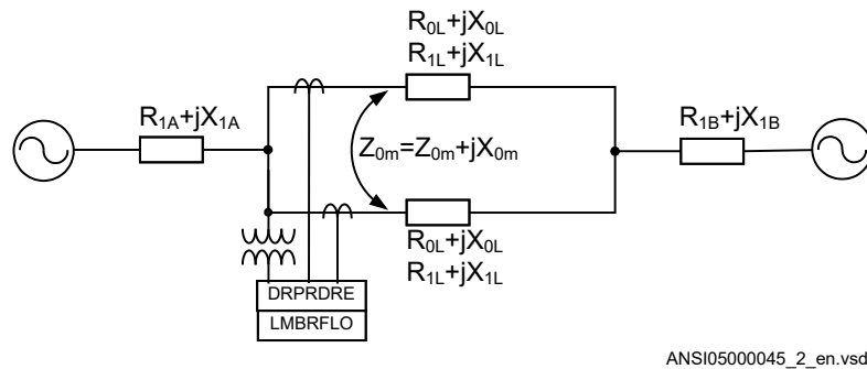
Figure 398: Simplified network configuration with network data, required for settings of the fault location-measuring function
