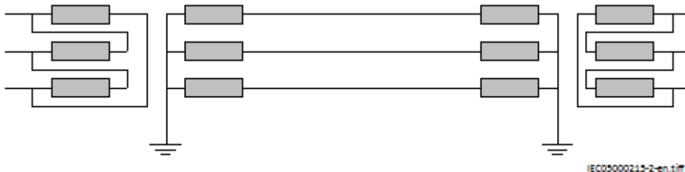
Figure 179: Solidly earthed network
