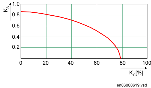
Figure 102: Underreaching safety factor K_S in dependence on system compensation degree K_C
