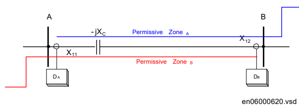
Figure 221: Permissive overreach distance protection scheme
