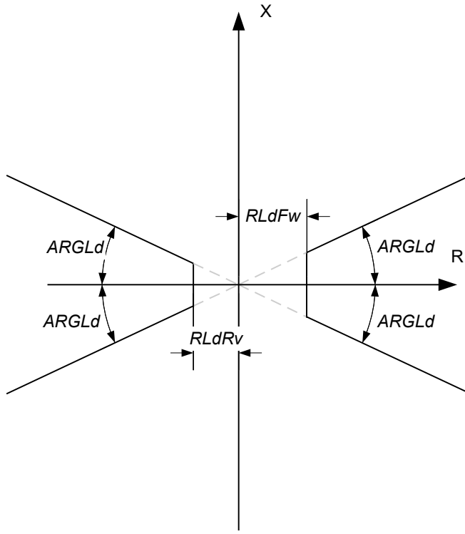
Figure 168: Characteristic of load encroachment function
