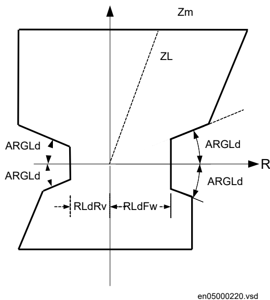
Figure 68: Characteristic for zone measurement for long line with load encroachment activated
