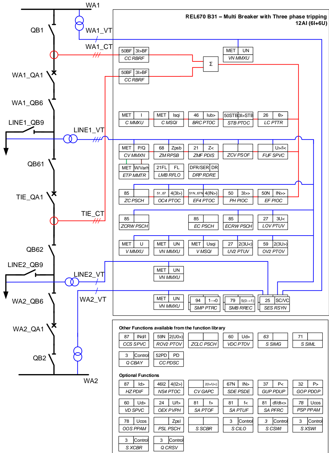
Figure 5: Configuration diagram for configuration B31
