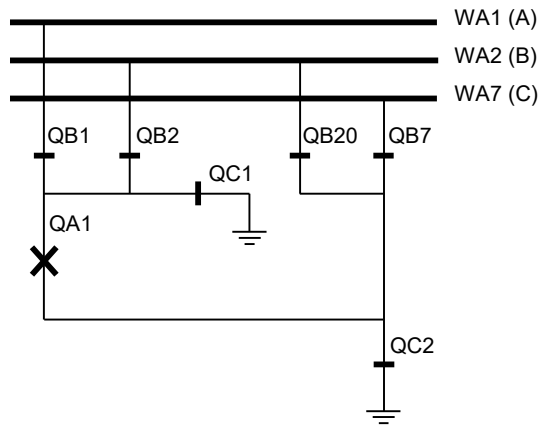
Figure 329: Switchyard layout ABC_BC
