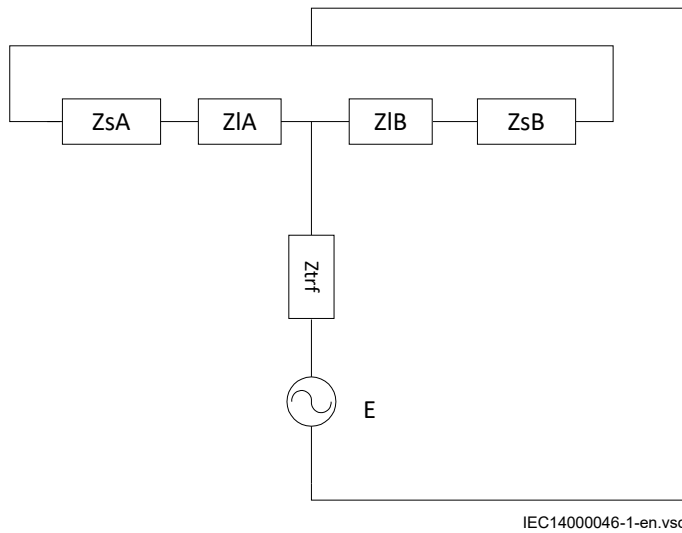
Figure 60: Thevenin equivalent for tap transformer
