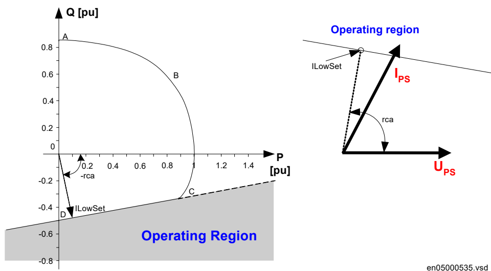
Figure 299: Loss of excitation
