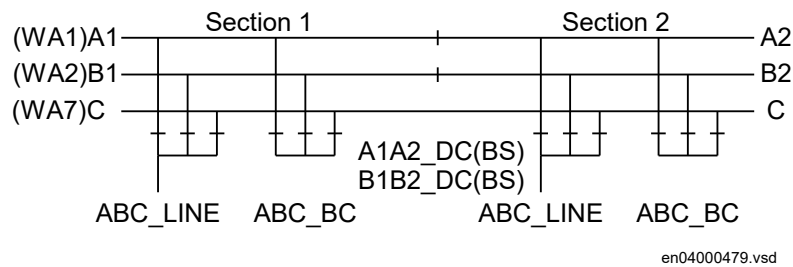
Figure 327: Busbars divided by bus-section disconnectors (circuit breakers)
