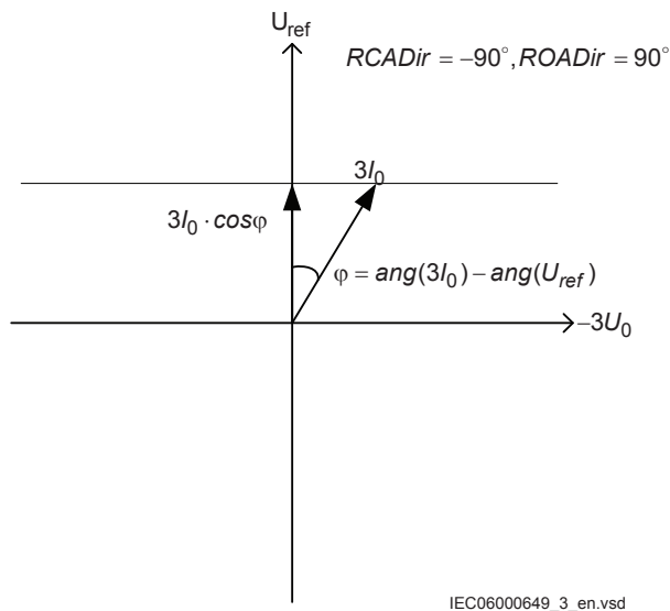
Figure 282: Characteristic for RCADir equal to -90^\circ
