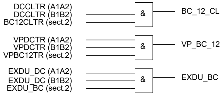
Figure 334: Signals to a bus-coupler bay in section 1 from a bus-coupler bay in another section
