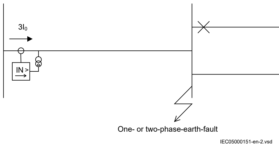
Figure 272: Step 1, second calculation. Remote busbar with, one line taken out of service
