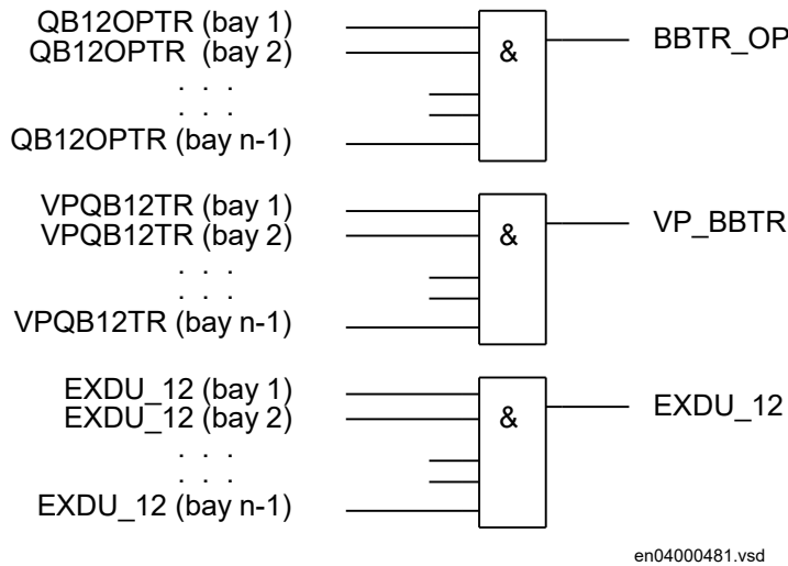
Figure 330: Signals from any bays in bus-coupler bay n
