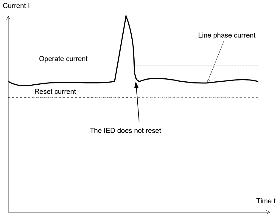
Figure 261: Operate and reset current for an overcurrent protection
