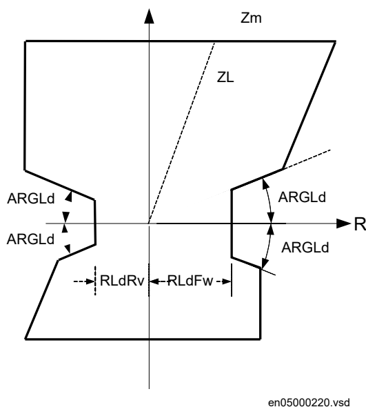
Figure 121: Characteristic for zone measurement for a long line
