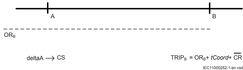
Figure 369: Principle of delta blocking scheme
