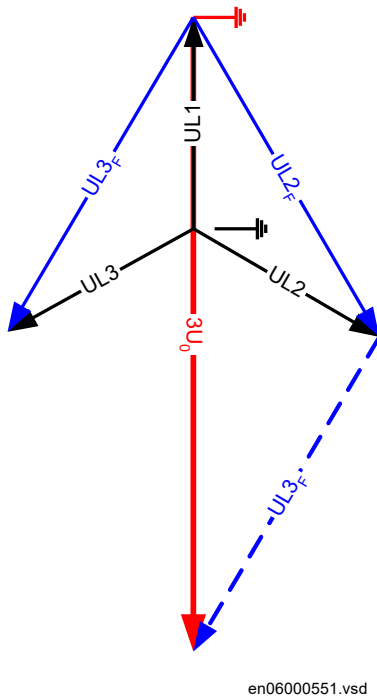
Figure 252: The voltage increase on healthy phases and occurring neutral point voltage ( 3U_0 ) at a single phase-to-earth fault and an occurring cross-country fault on different feeders in a sub-transmission network, high impedance (resistance, reactance) earthed
