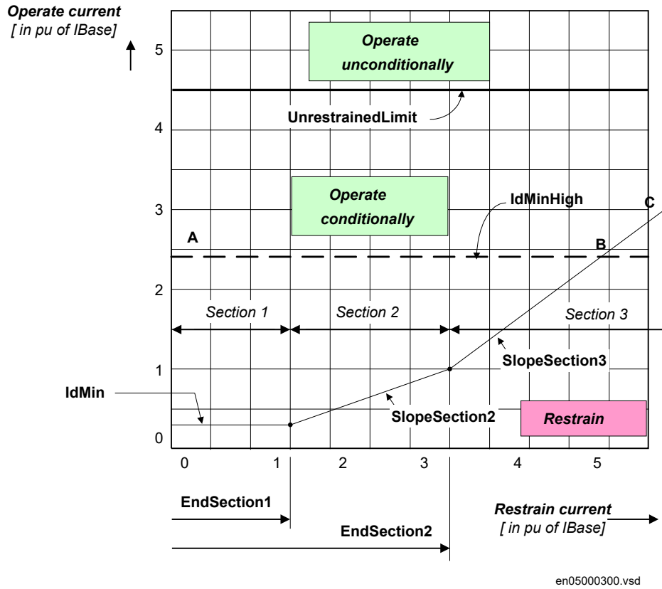
Figure 50: Restrained differential function characteristic (reset ratio 0.95)
