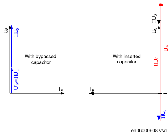
Figure 212: Phasor diagrams of currents and voltages for the bypassed and inserted series capacitor during current inversion
