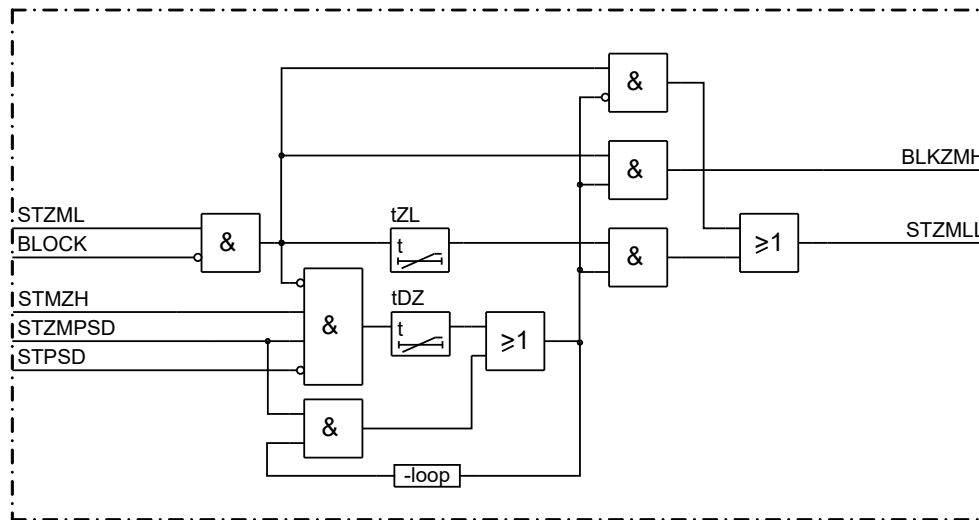
Figure 239: Blocking and tripping logic for evolving power swings
