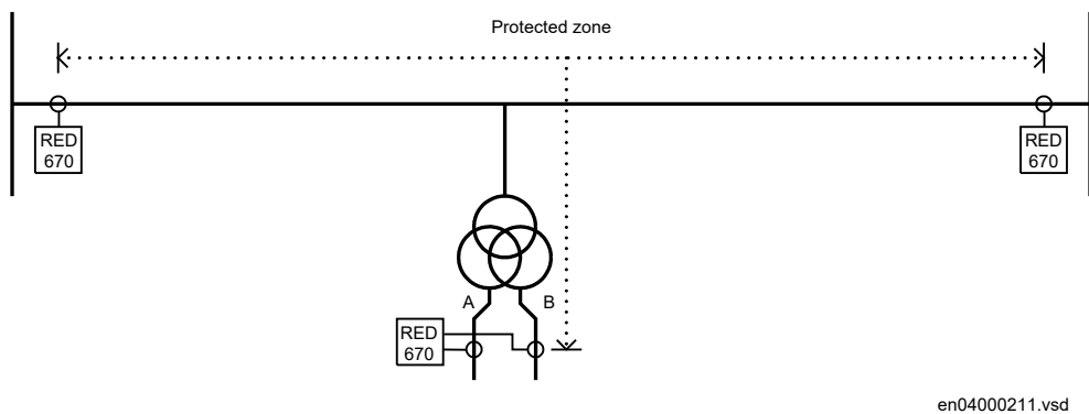
Figure 55: One three-winding transformer in the protected zone
