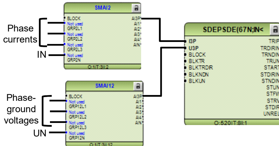
Figure 279: Connection of SDEPSDE to analog preprocessing function block
