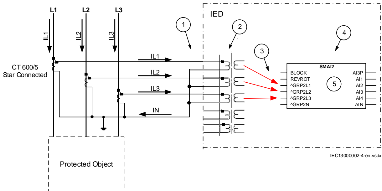
Figure 14: Star connected three-phase CT set with star point towards the protected object
