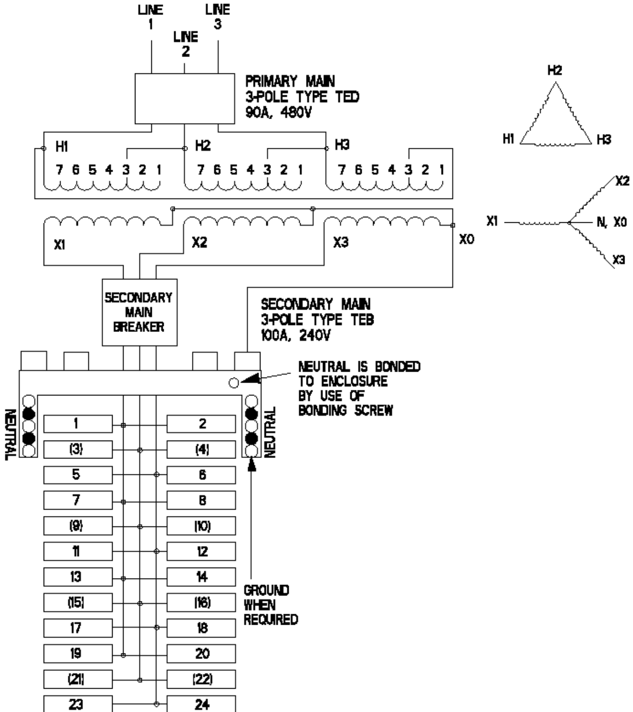
FIGURE 1 - TYPICAL WIRING DIAGRAM DO NOT MAKE OR CHANGE CONNECTIONS WHILE UNIT IS ENERGIZED !!
