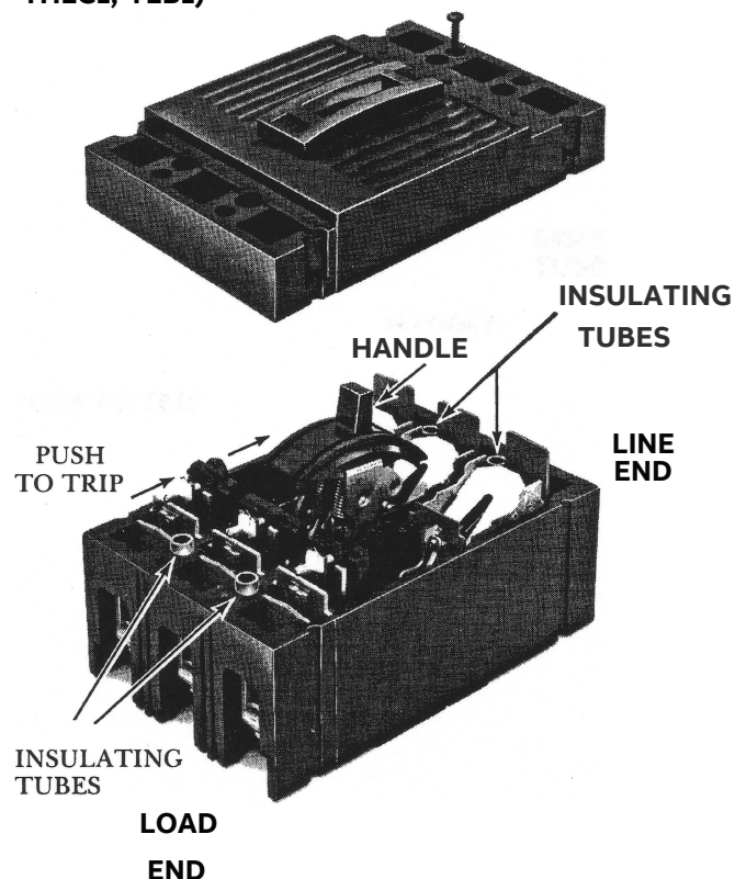
Figure 3. TED Breaker with cover removed
