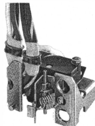
TWO STAGE AUXILIARY SWITCH (LEFT POLE ASSEMBLY SHOWN)
