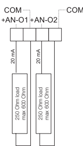
M2M I/O analogue outputs
