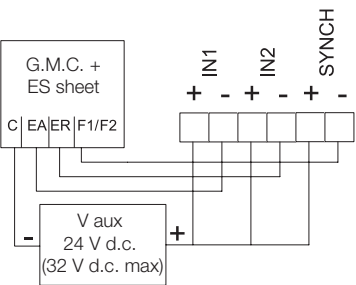
M2M I/O digital inputs (example in NPN mode)
