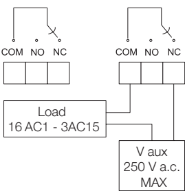
M2M ALARM electromechanical relay outputs
