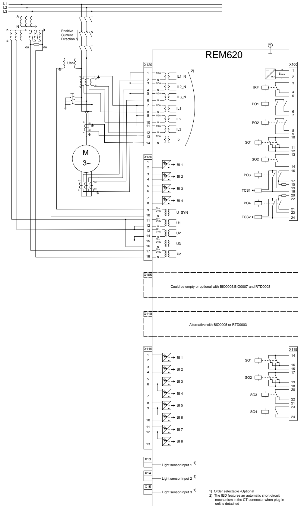
Figure: REM620 ME201 Connection diagram for standard modules
