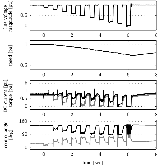
Fig. 7. Simulation results: Speed, DC current, torque and control angles during a voltage dip scenario with MPC. The current and inverter angle are plotted in black. The torque and rectifier angle are plotted in gray.
