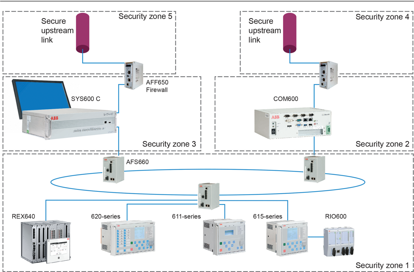
Figure 2: Distribution substation example
